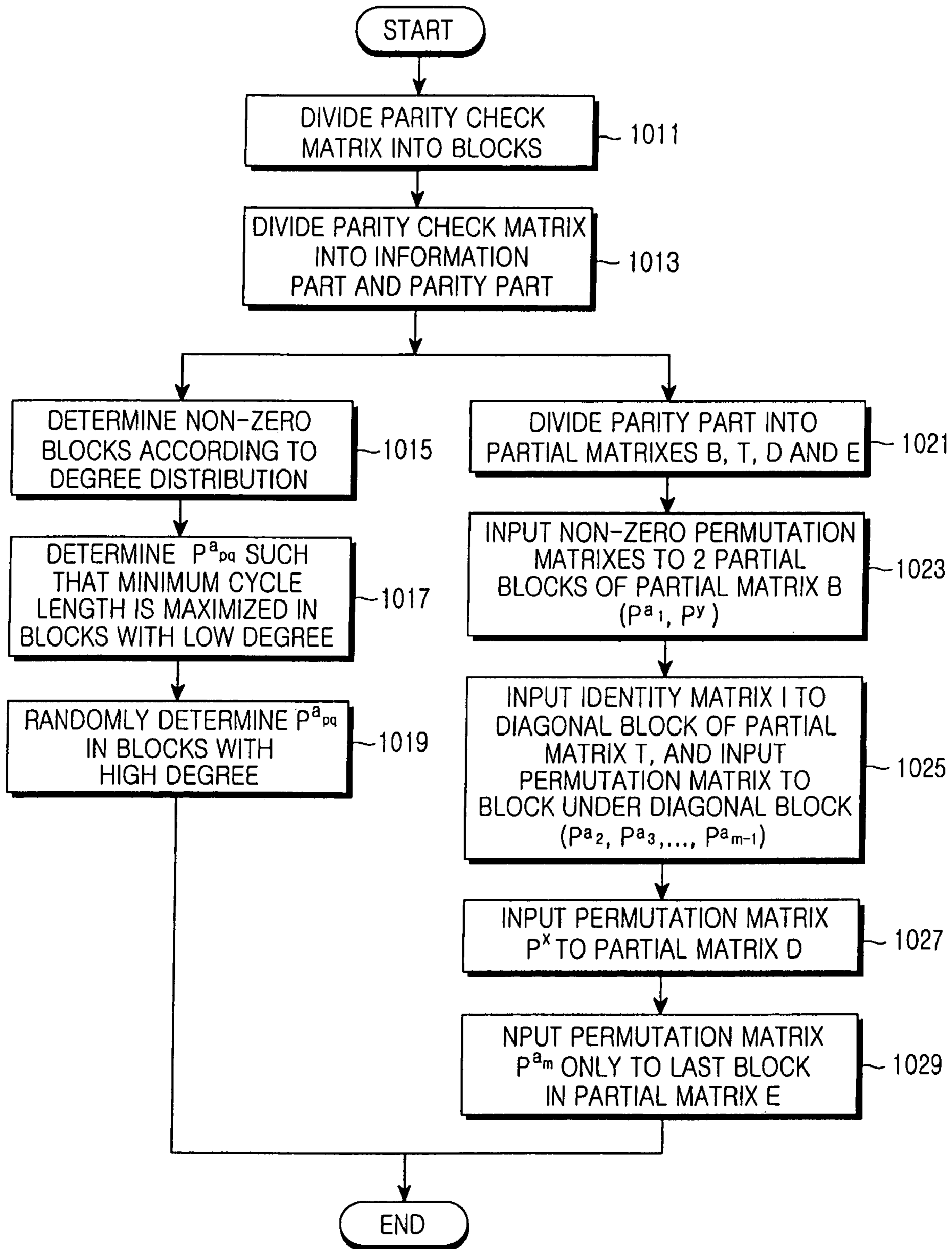
FIG. 10 (PRIOR ART)
