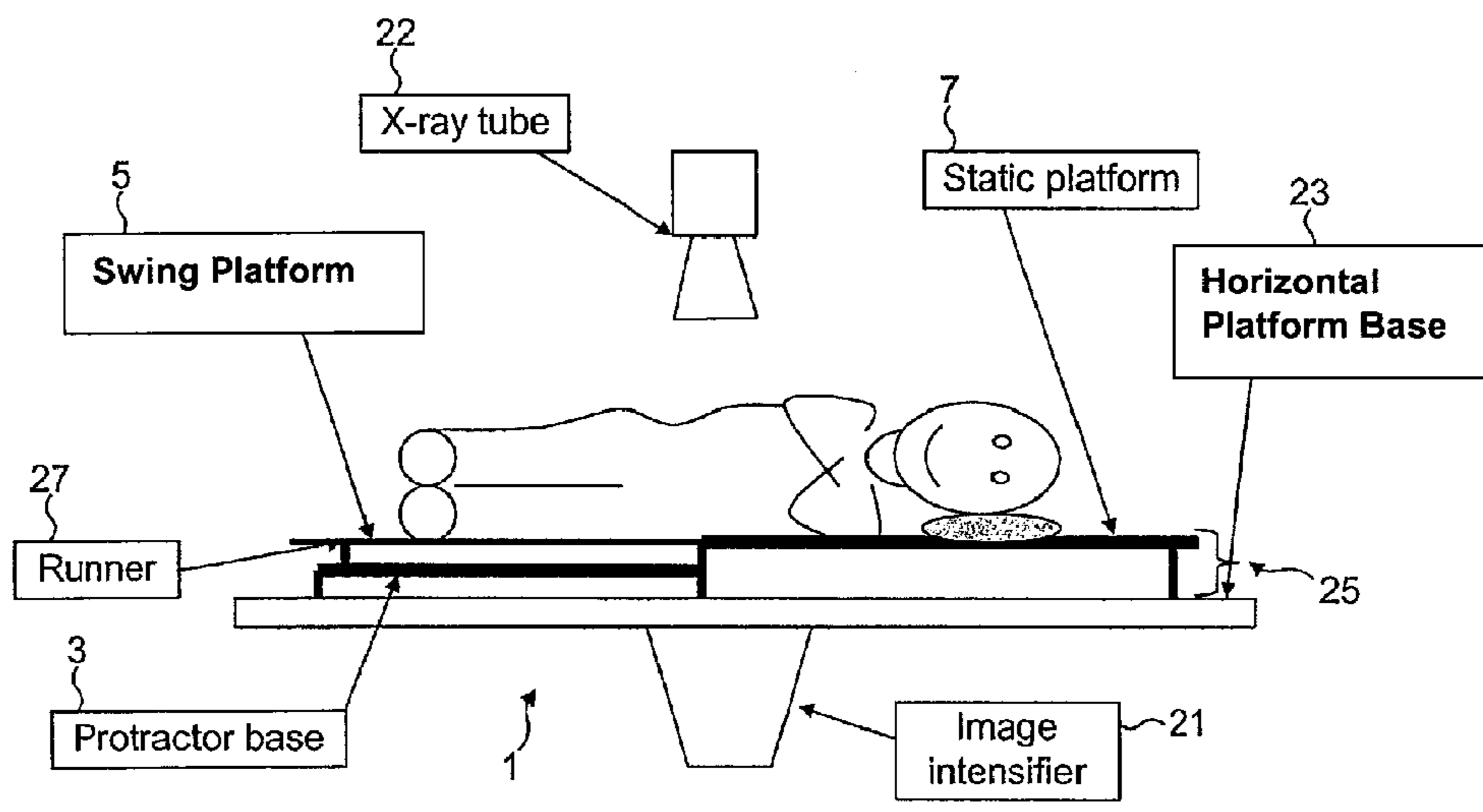
Passive Motion Platform - Side Elevation
