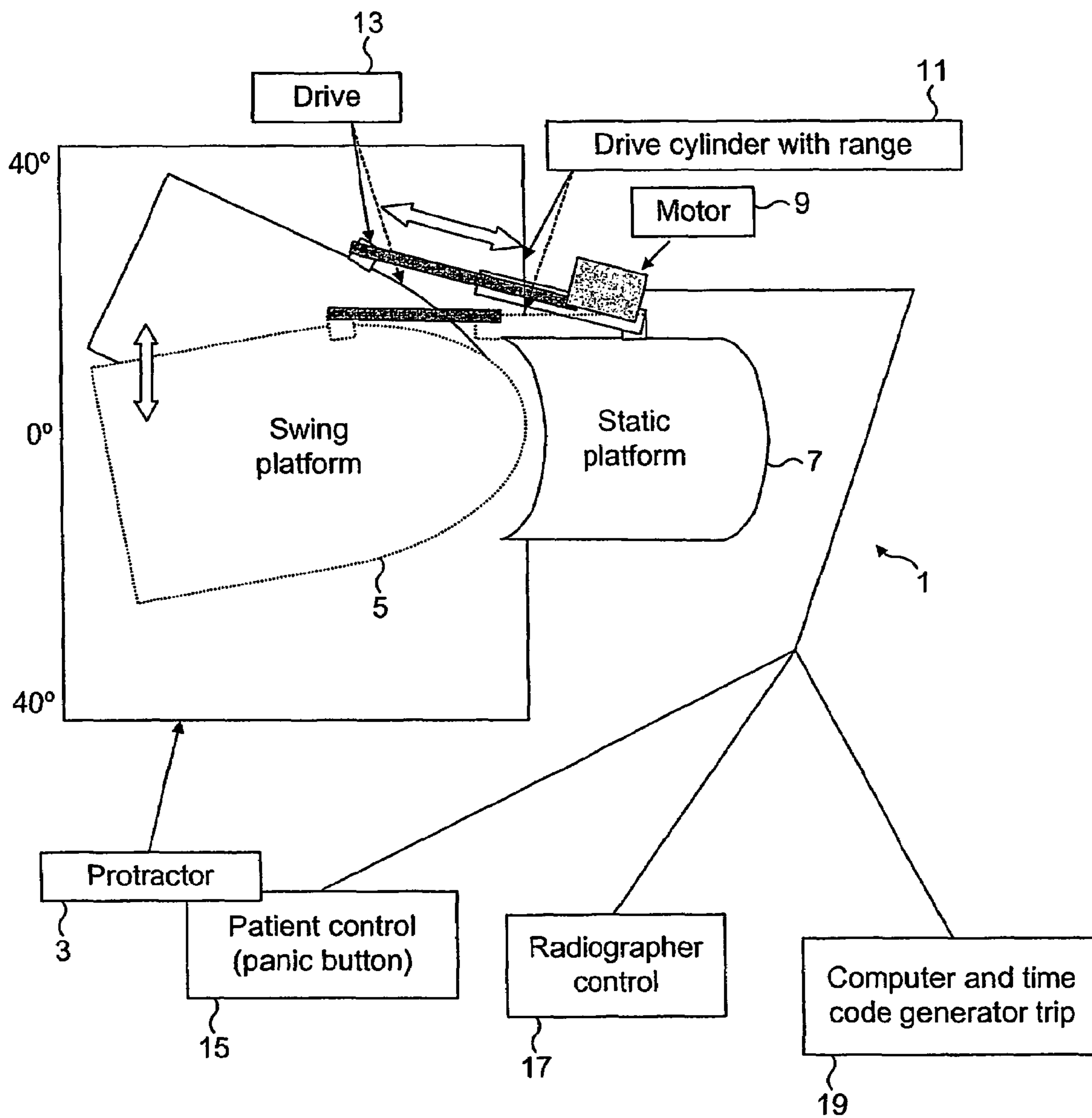
Passive Motion Platform - Top Elevation
