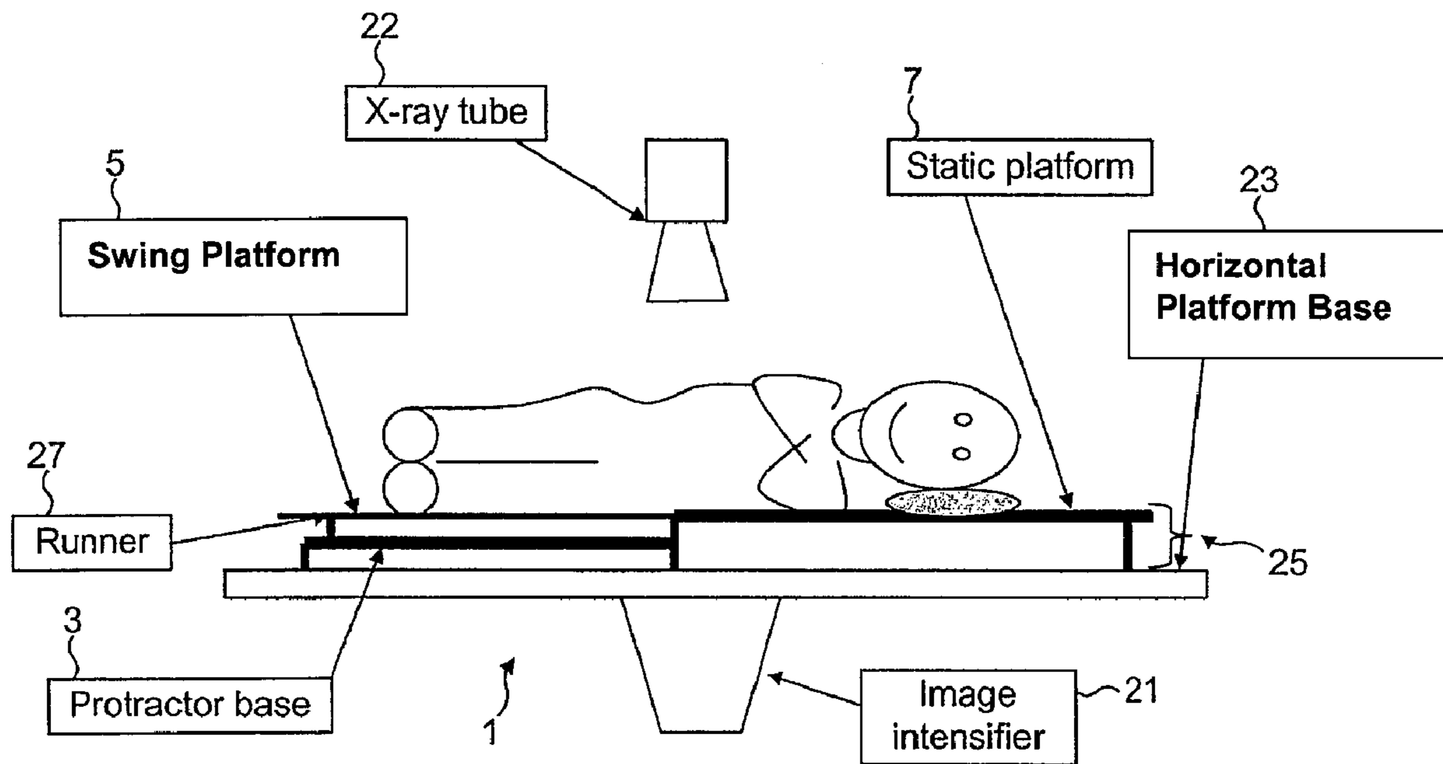
Passive Motion Platform - Side Elevation
