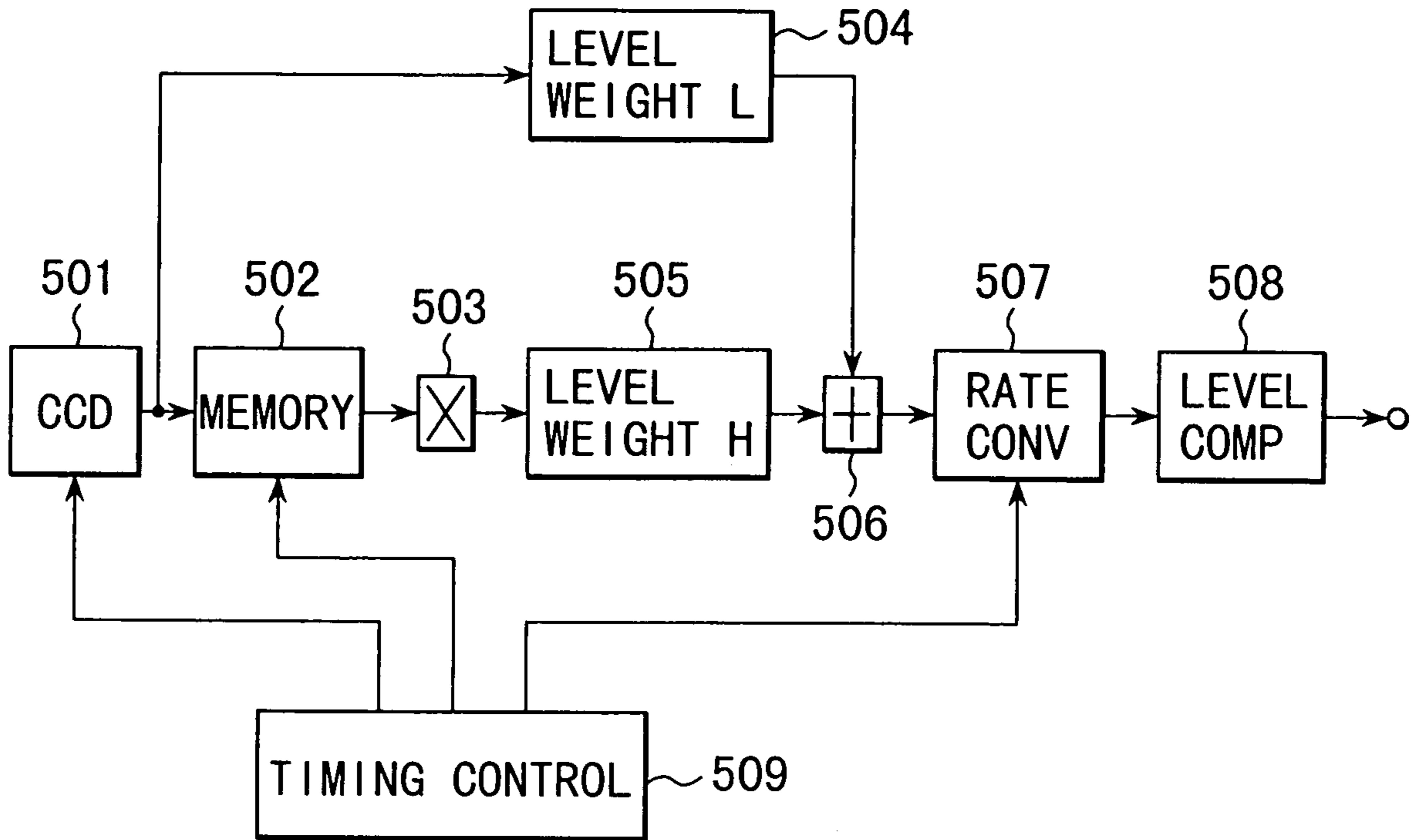
FIG. 1 PRIOR ART
