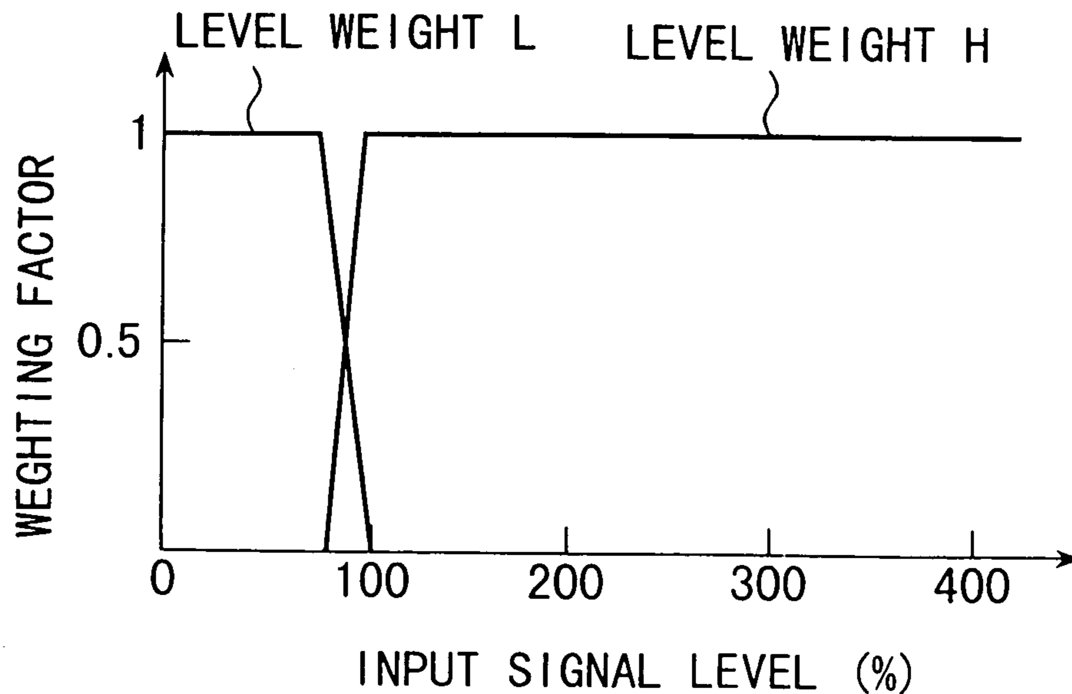
FIG. 2 PRIOR ART
