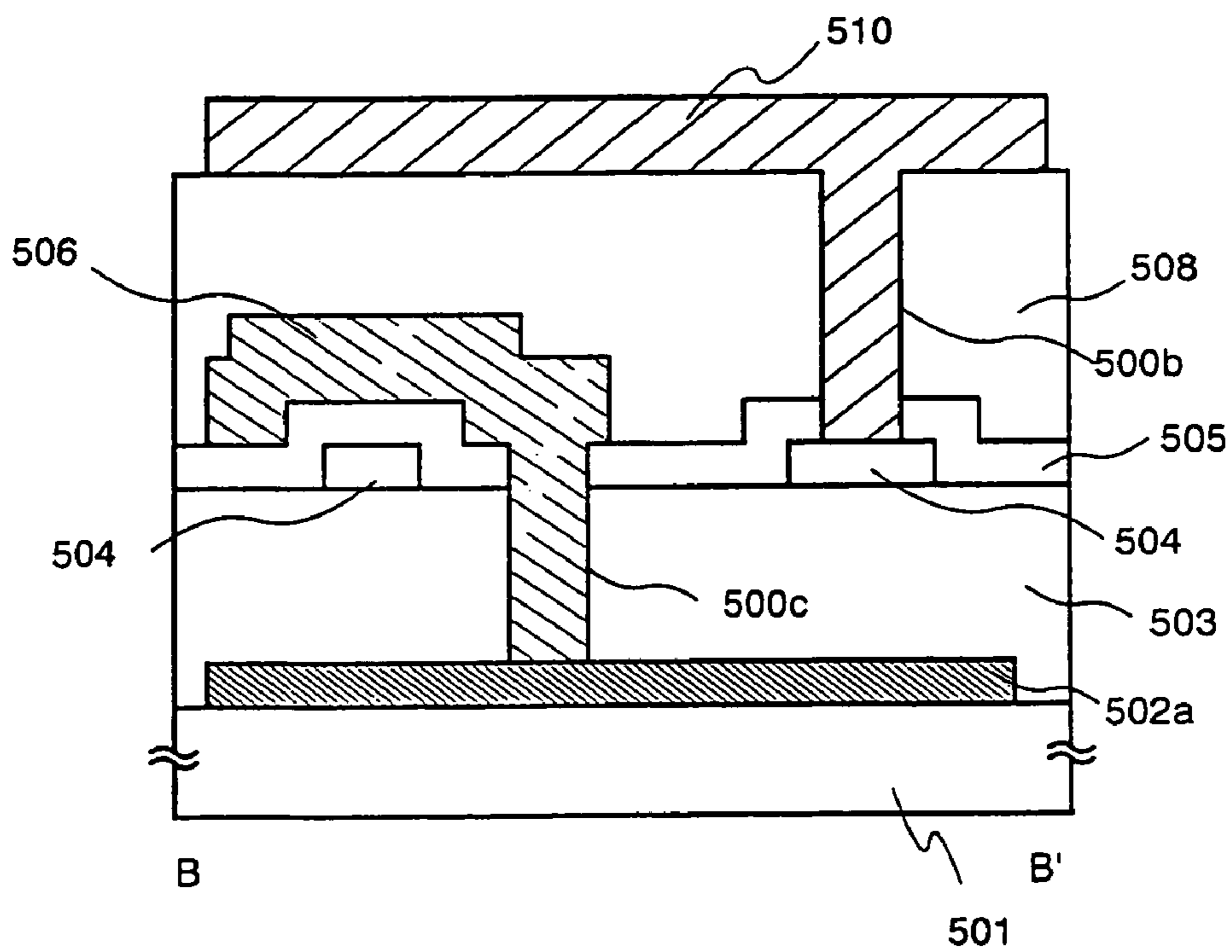
Fig. 15B B-B' Cross sectional view
