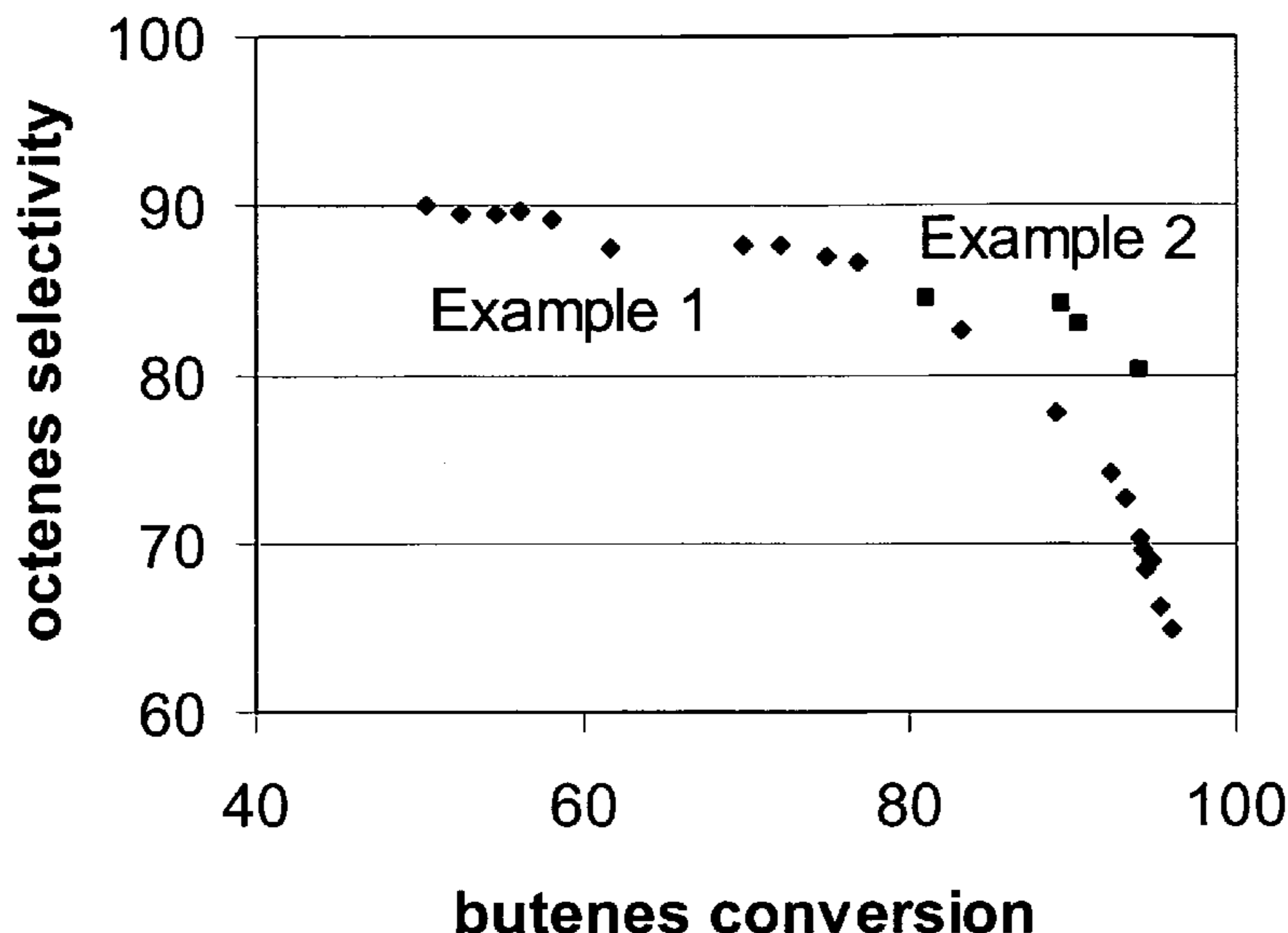
Octenes Selectivity vs. Conversion
