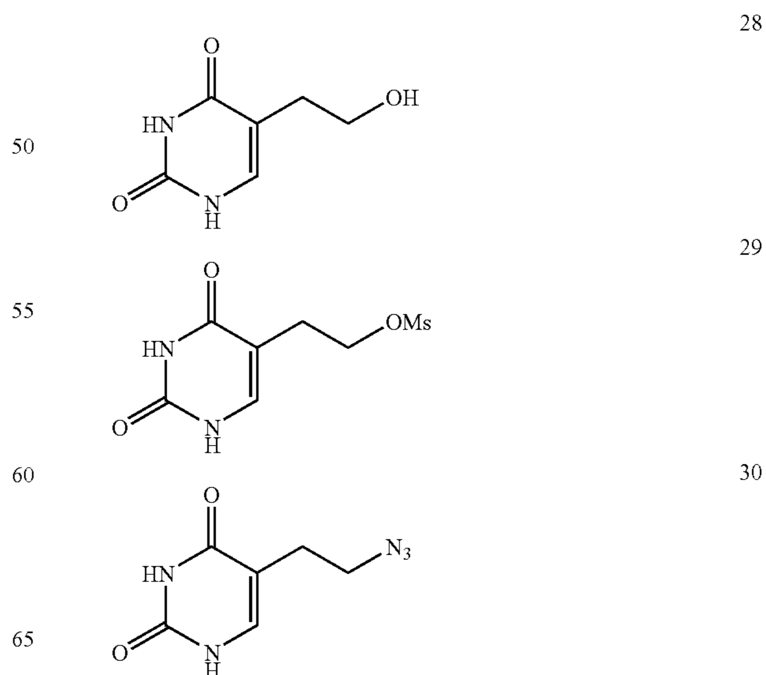
Scheme 5: Synthesis of N-phthaloylaminoethyluracil 32.
