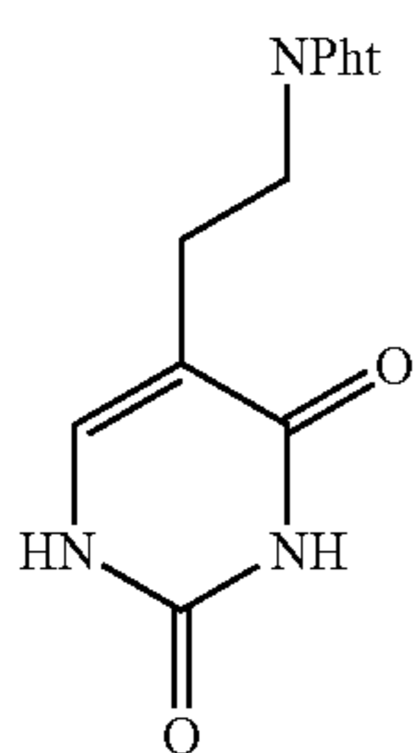
Scheme 6: Synthesis of the linker phosphoramidite 39.
