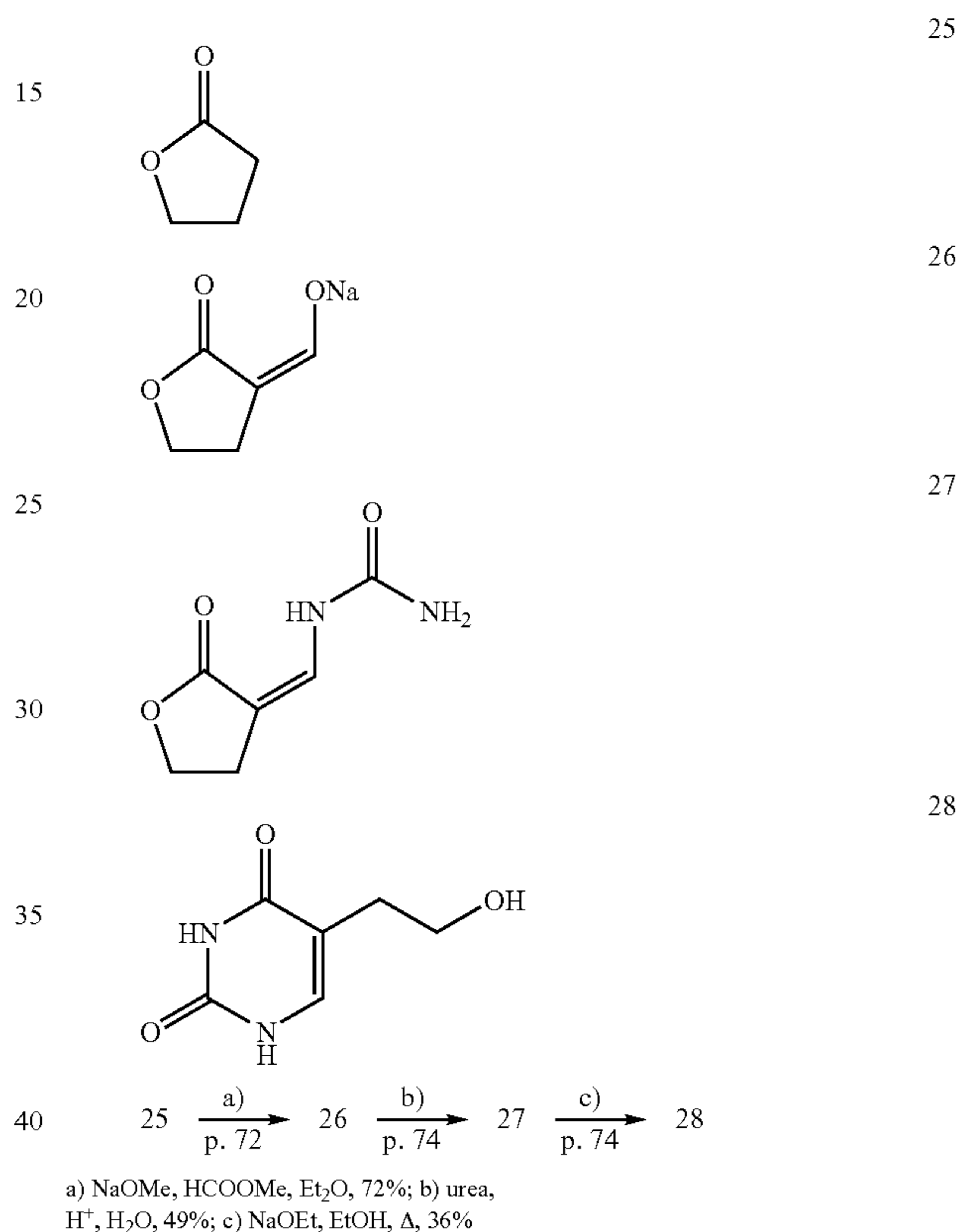
Scheme 4: Synthesis of hydroxyethyluracil 28.
