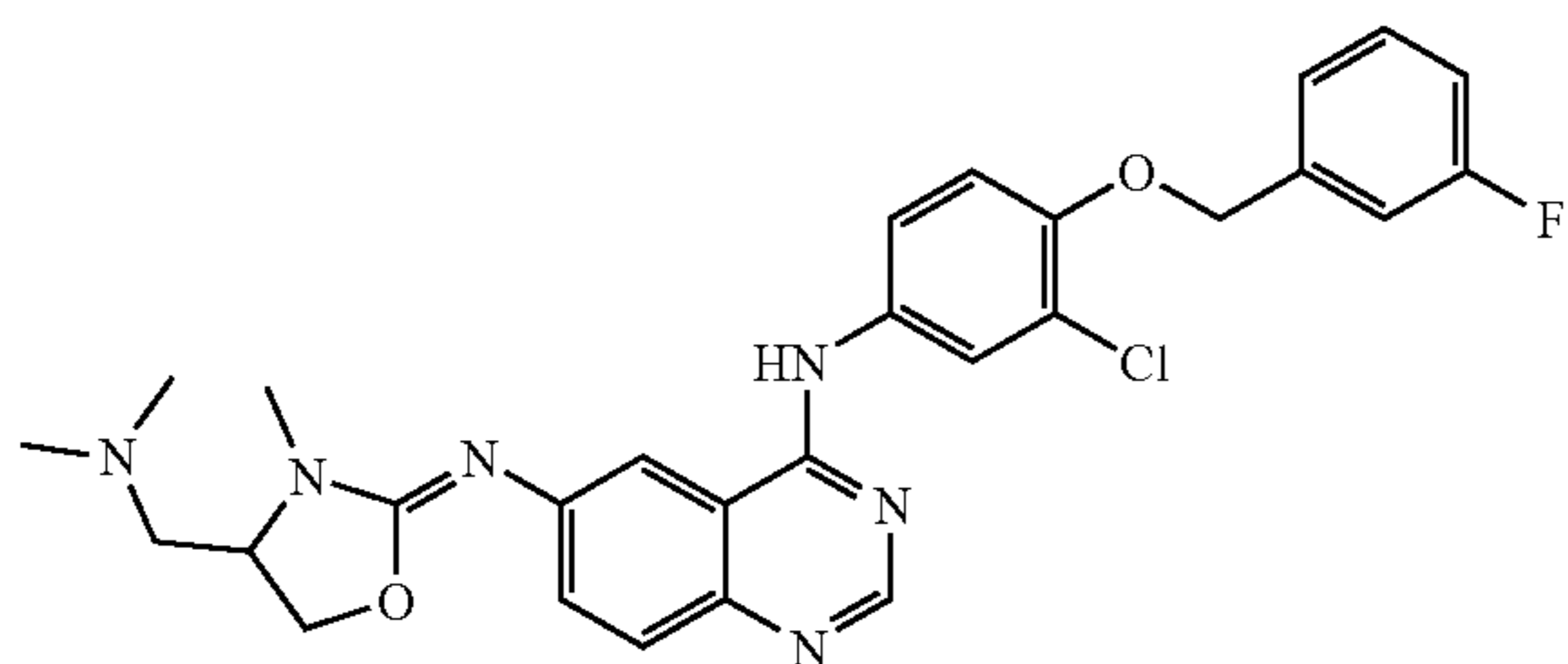
N-4-[3-Chloro-4-(3-fluoro-benzyloxy)-phenyl]-N6-(4-dimethylaminomethyl-3-methyl-oxazolidin-2-ylidene)-quinazoline-4,6-diamine
