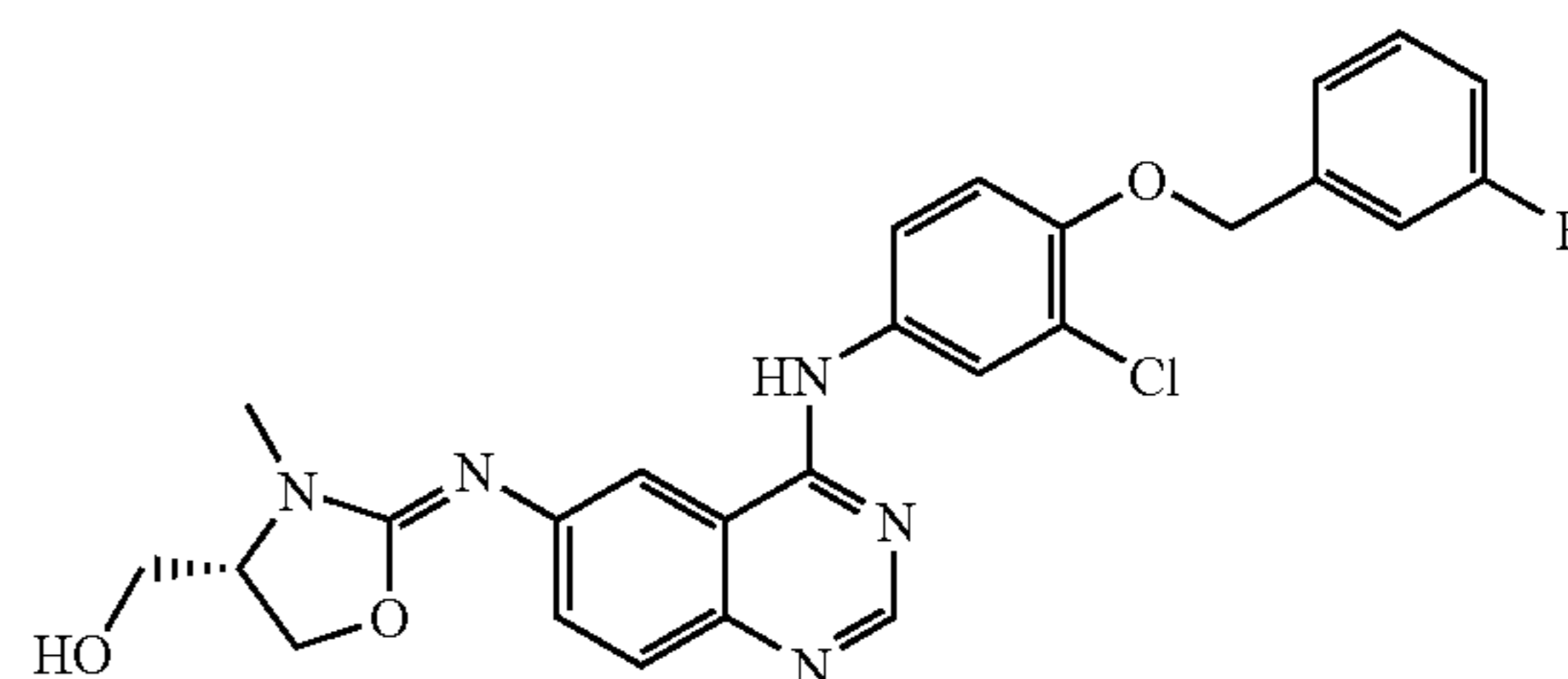
(S)-(2-{4-[3-Chloro-4-(3-fluoro-phenoxy)methyl]-phenylamino}-quinazolin-6-ylimino)-3-methyl-oxazolidin-4-yl)-methanol
