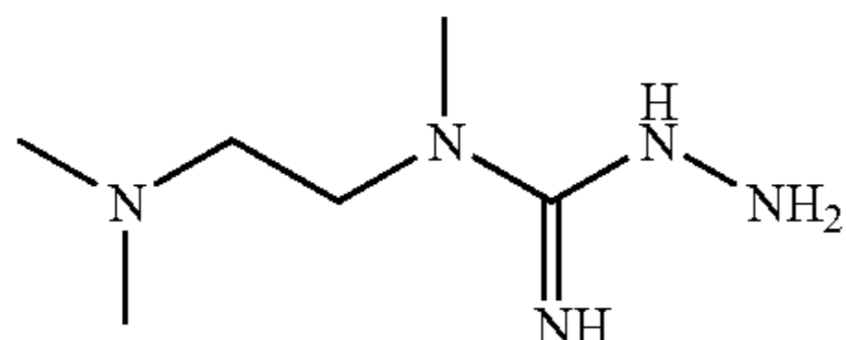
N-Methyl-N-(2-dimethylamino-ethyl) hydrazinecarboximidamide
