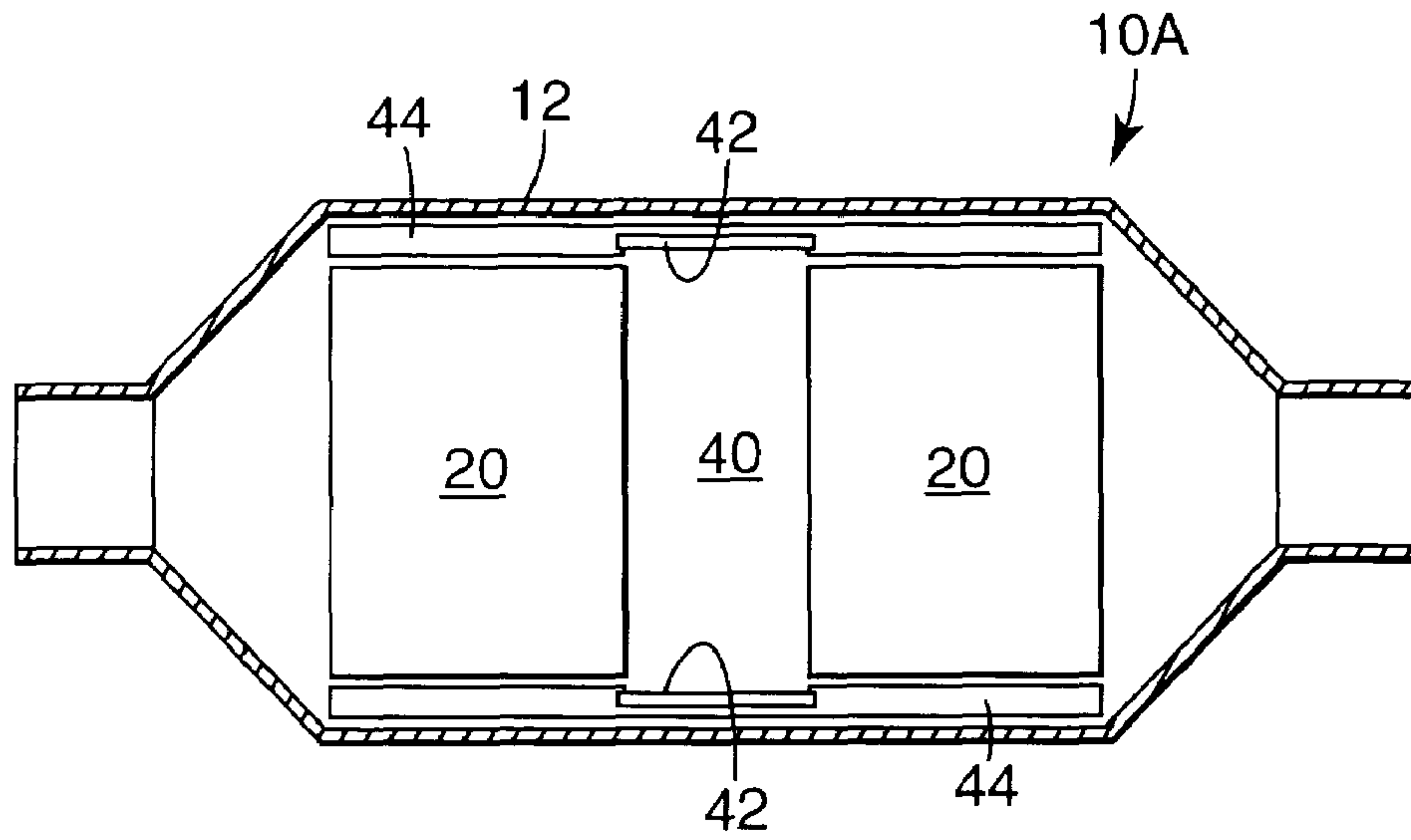
Fig. 9 (PRIOR ART)
