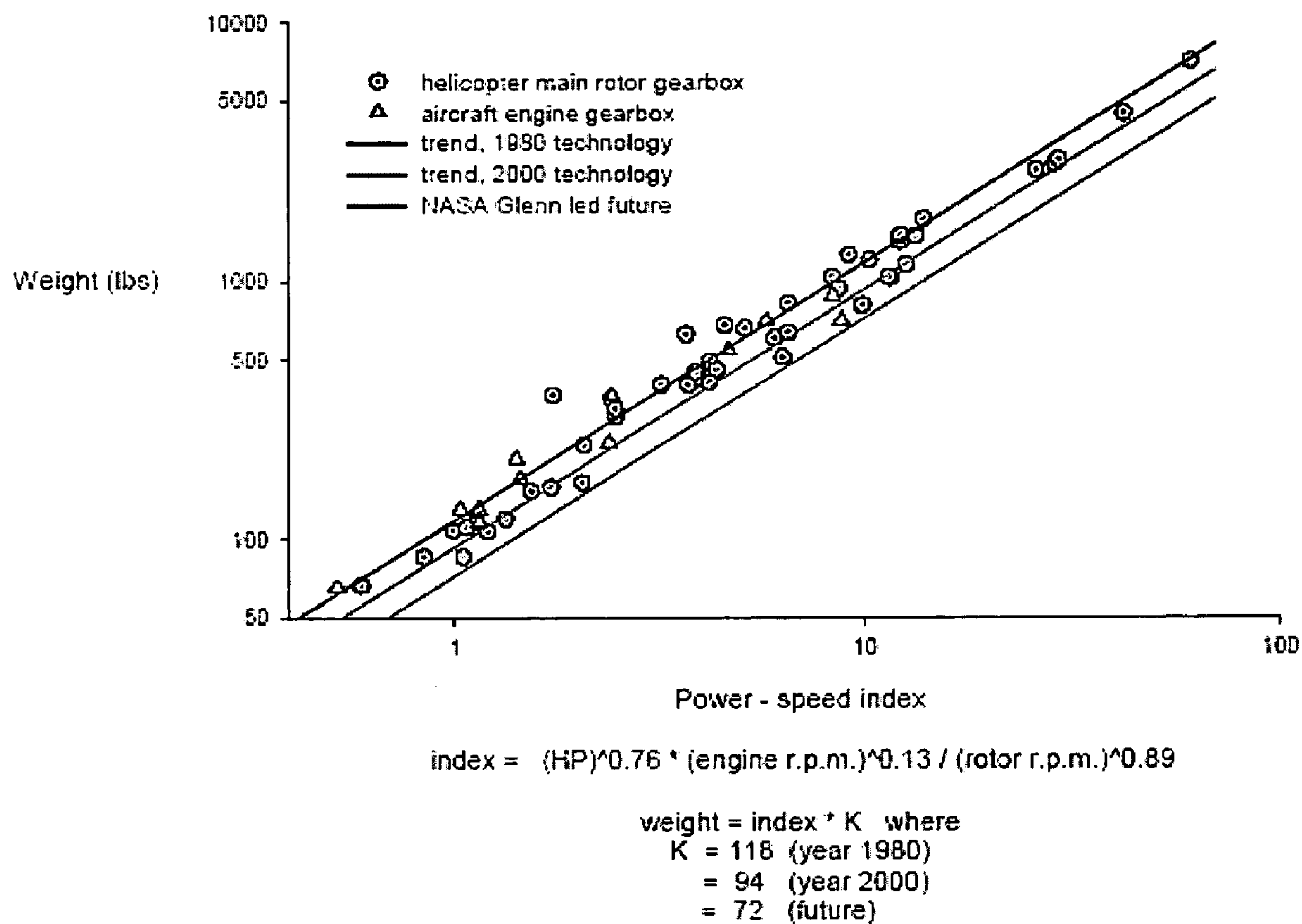
Historic and future gearbox weight trends (based on 49 single-rotor helicopter and 12 aircraft engine gearboxes)
