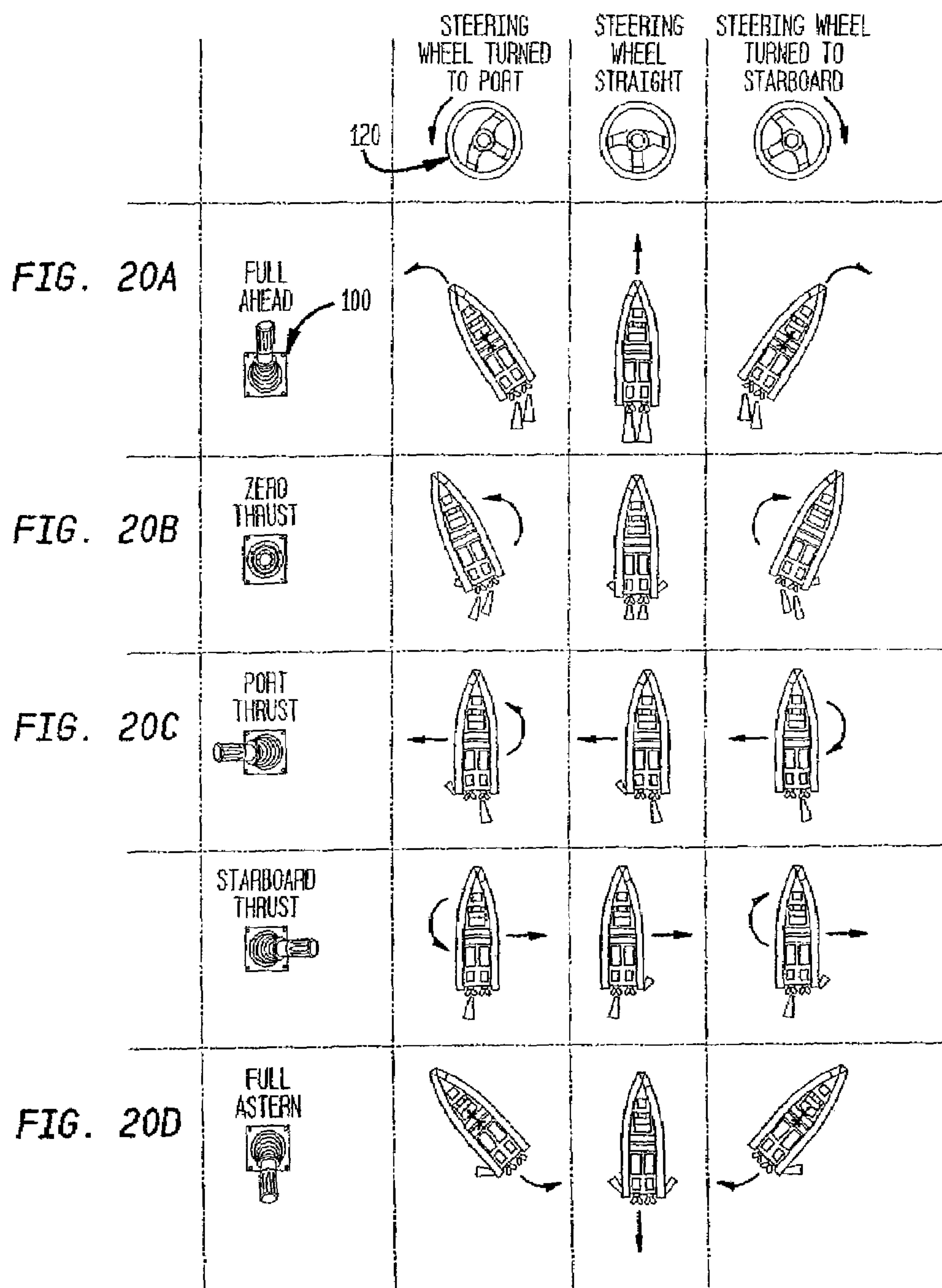
DUAL WATERJET MOTION DIAGRAM
