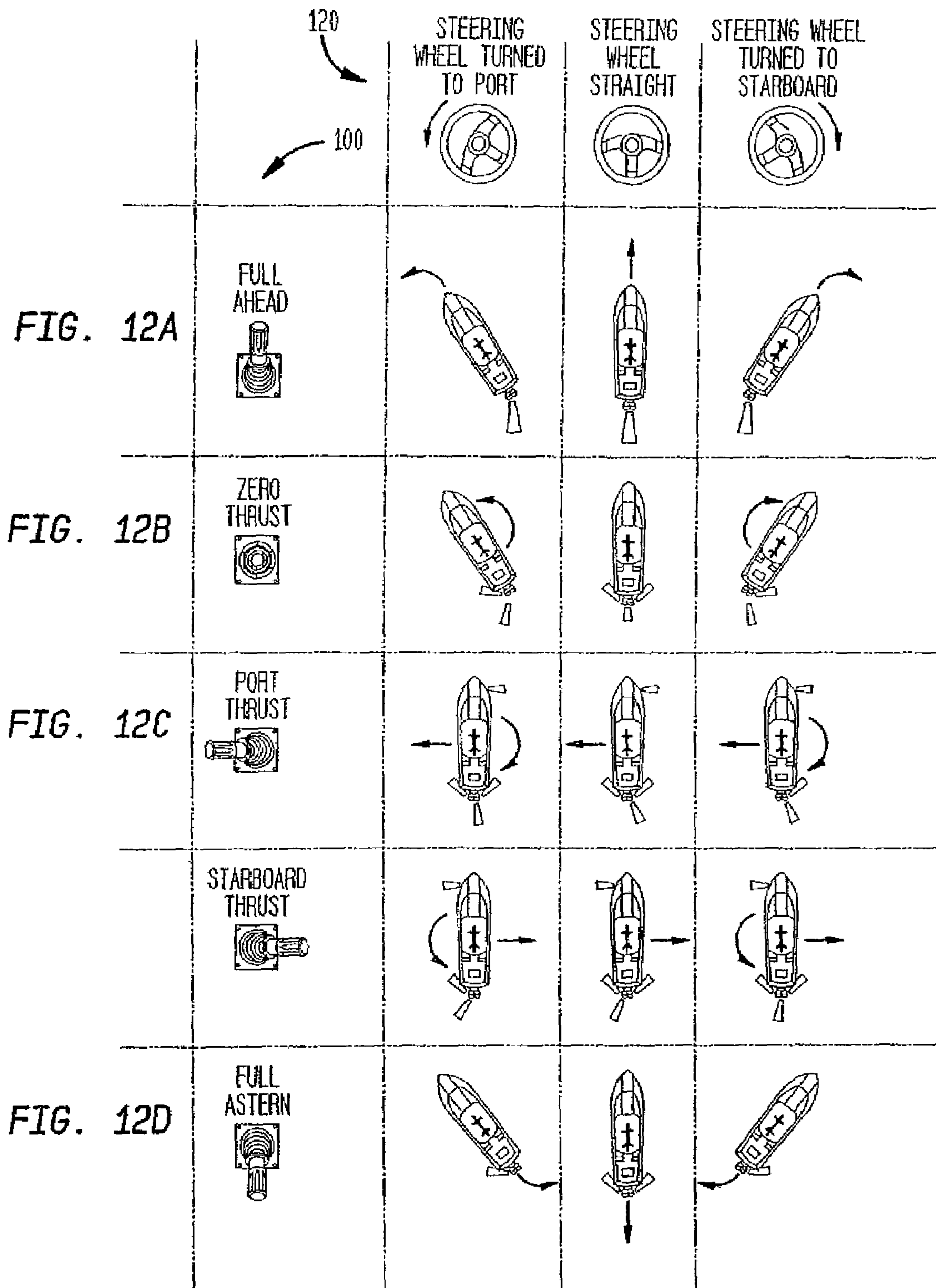
SINGLE WATERJET MOTION DIAGRAM
