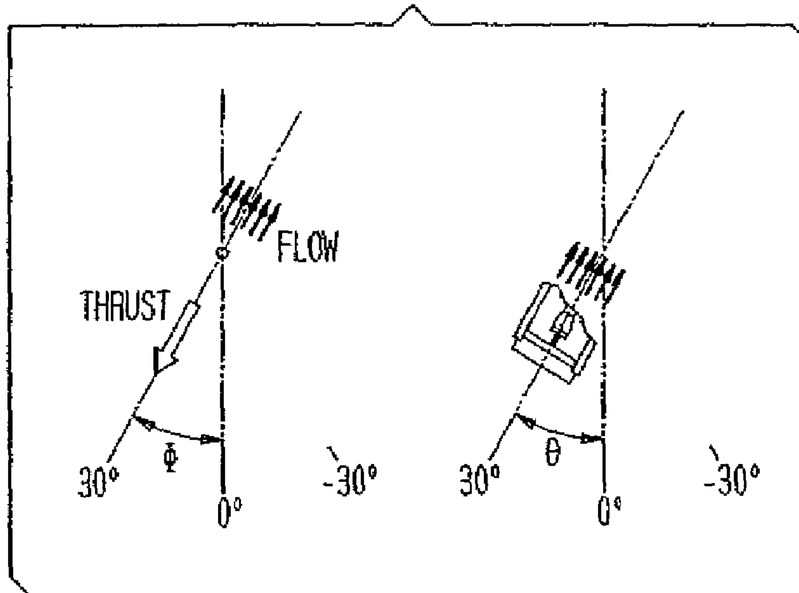
FIG. 22B FULL REVERSE BUCKET
