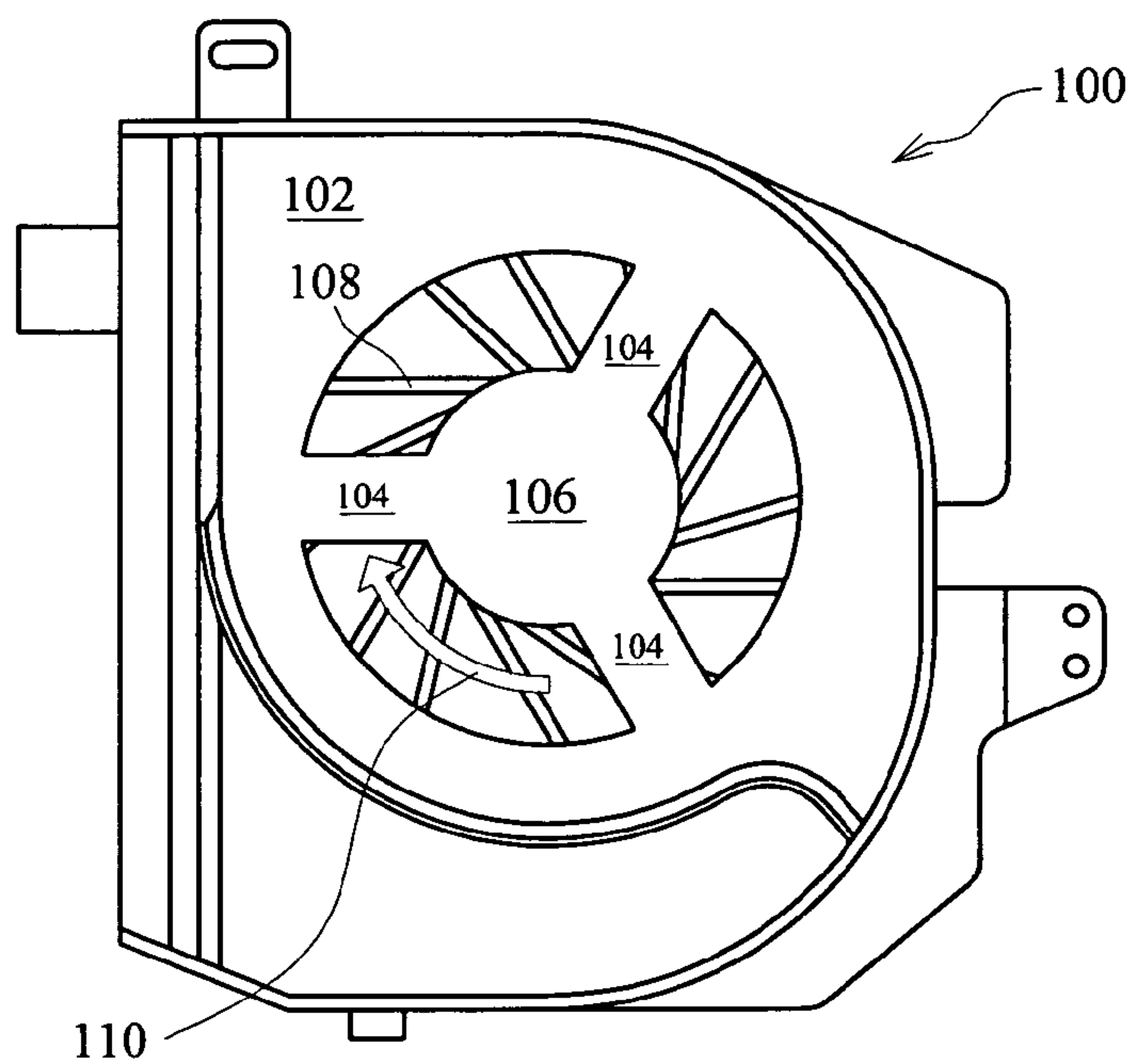
Fig. 1 (PRIOR ART)
