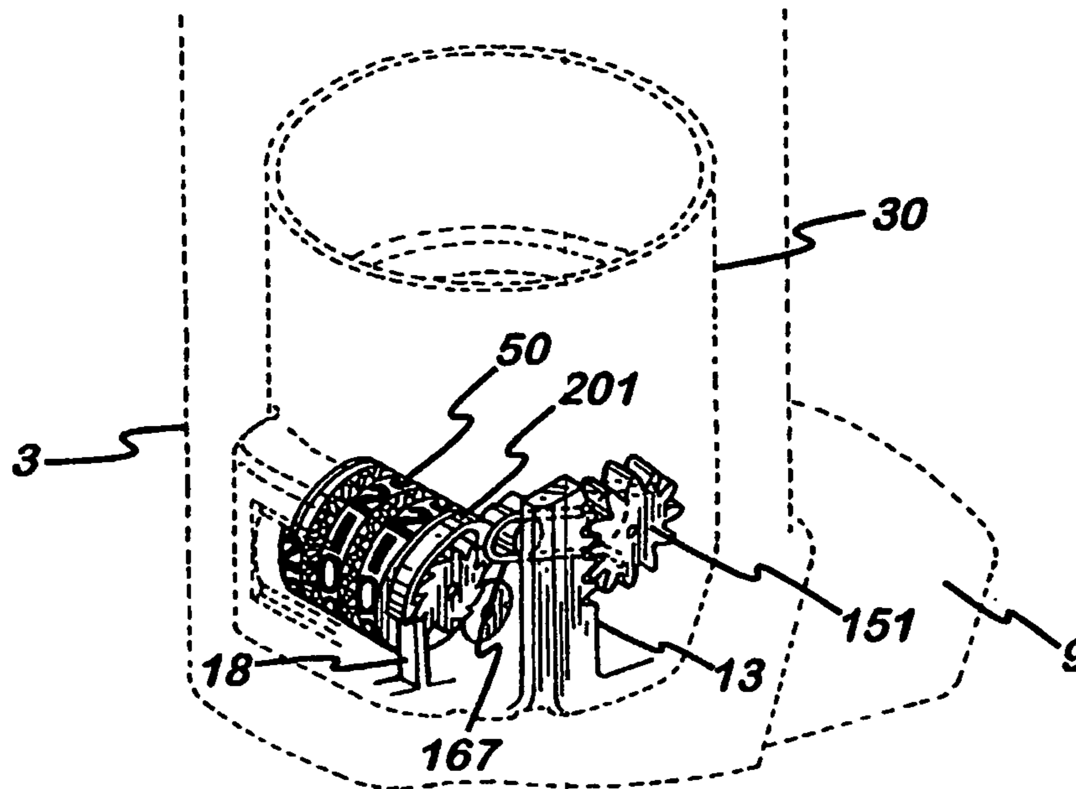
Fig. 12B Bottom of downstroke
