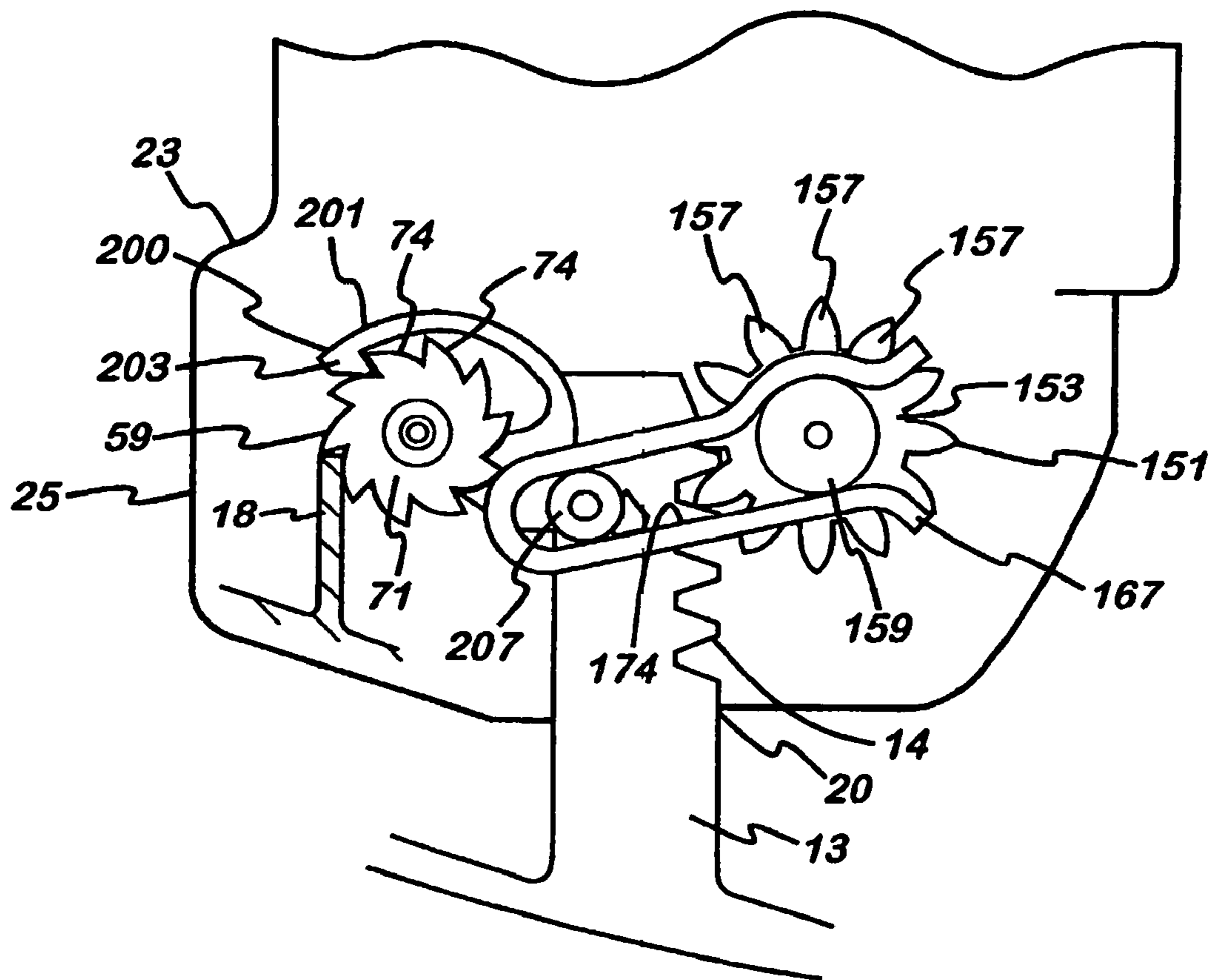
Fig. 10A Mechanism at rest
