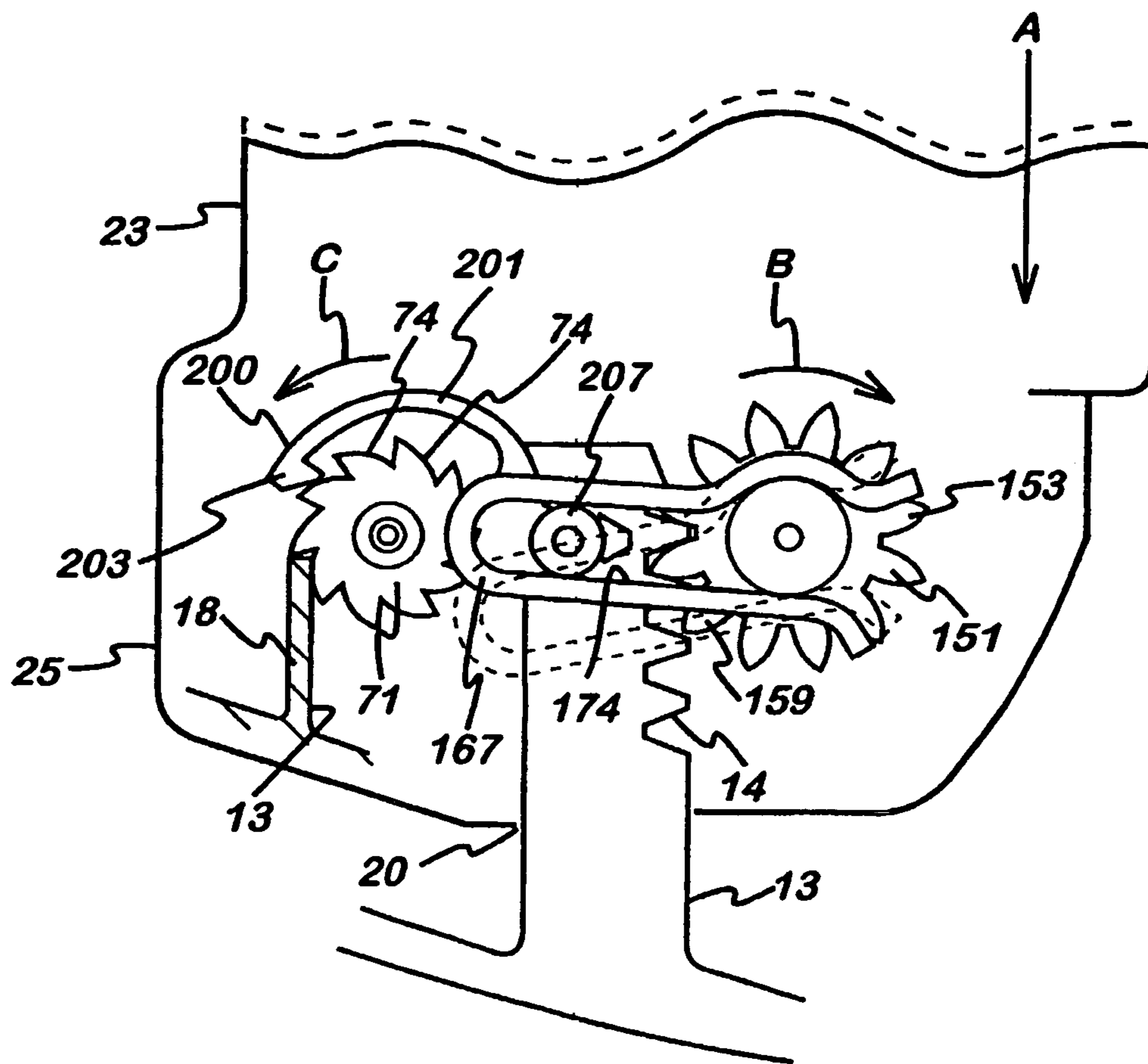
Fig. 11A Start of downstroke
