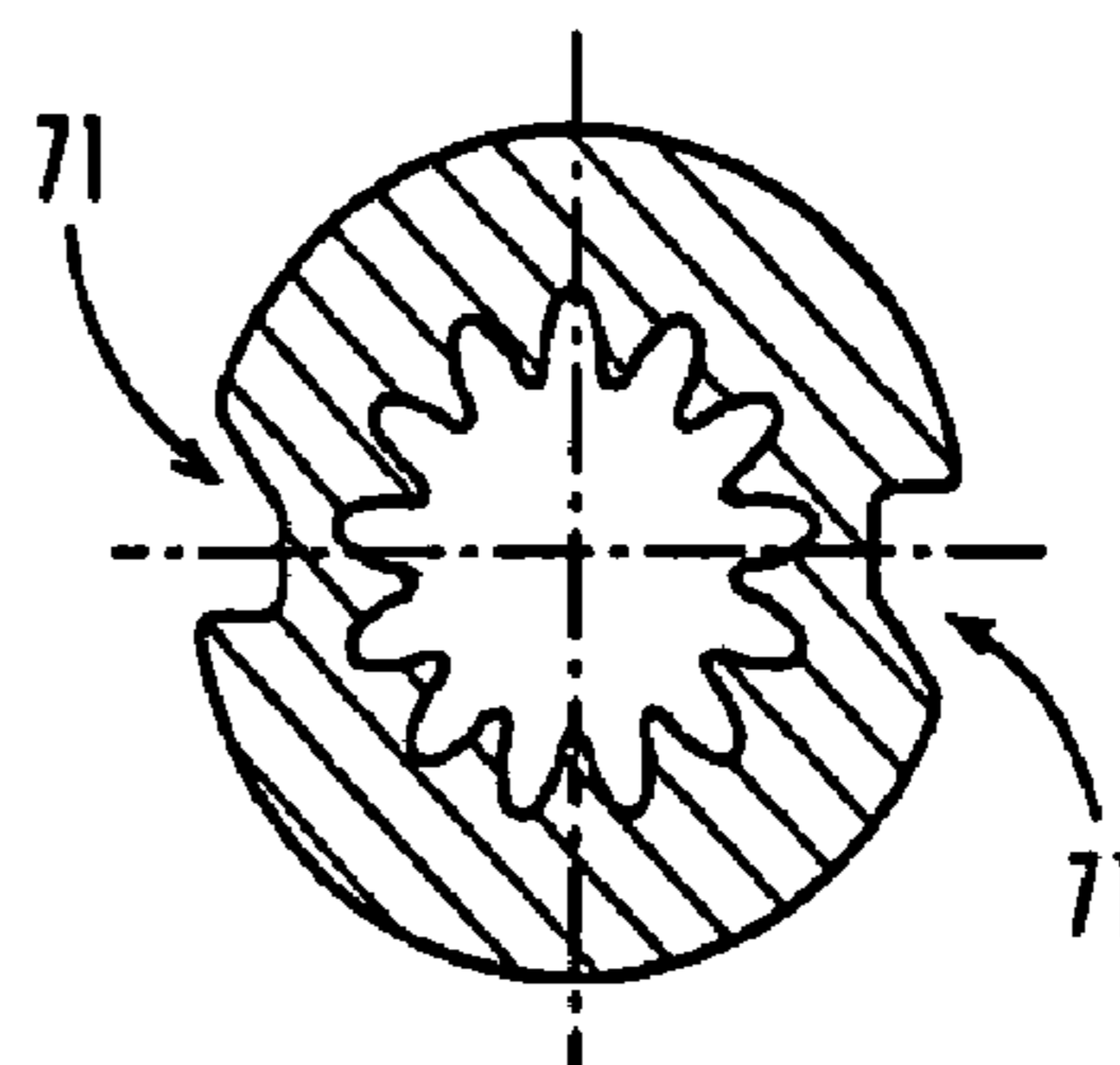
Fig. 7D (Section 7D - 7D)
