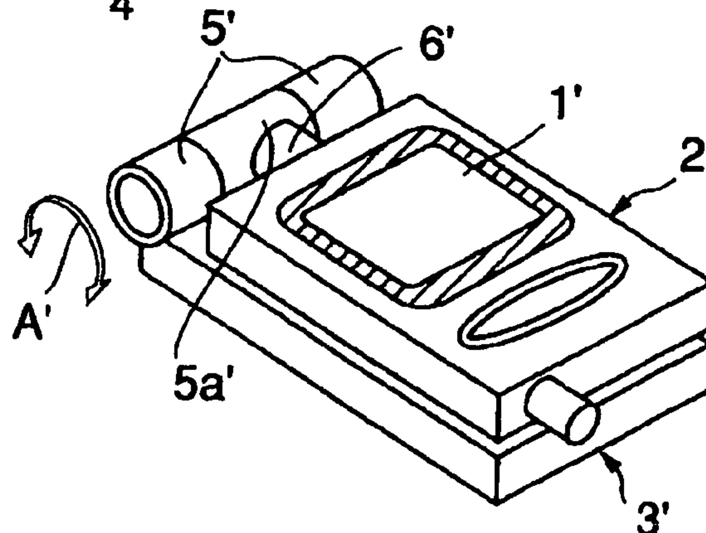
FIG.2C (PRIOR ART)
