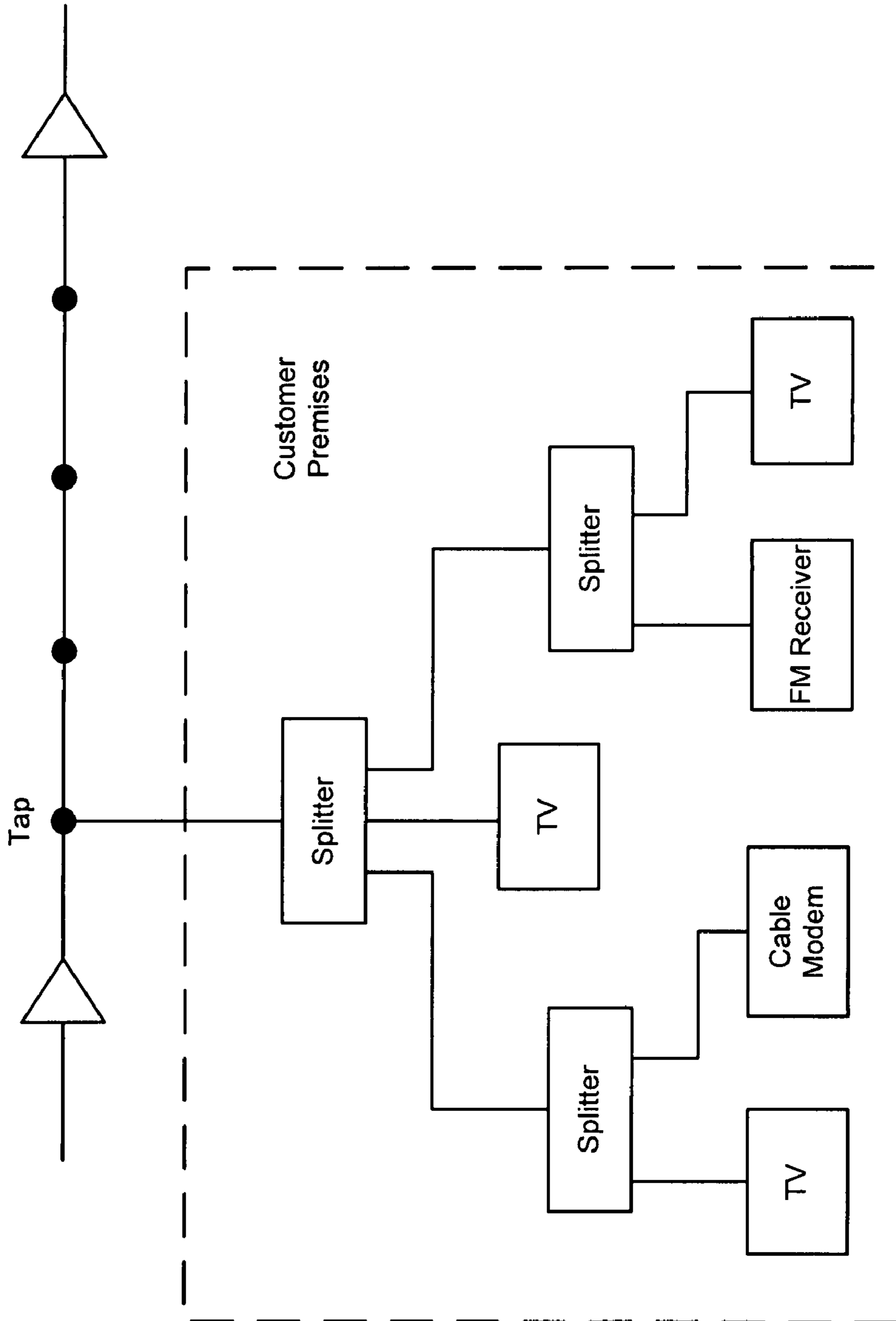
Fig. 1 Prior Art
