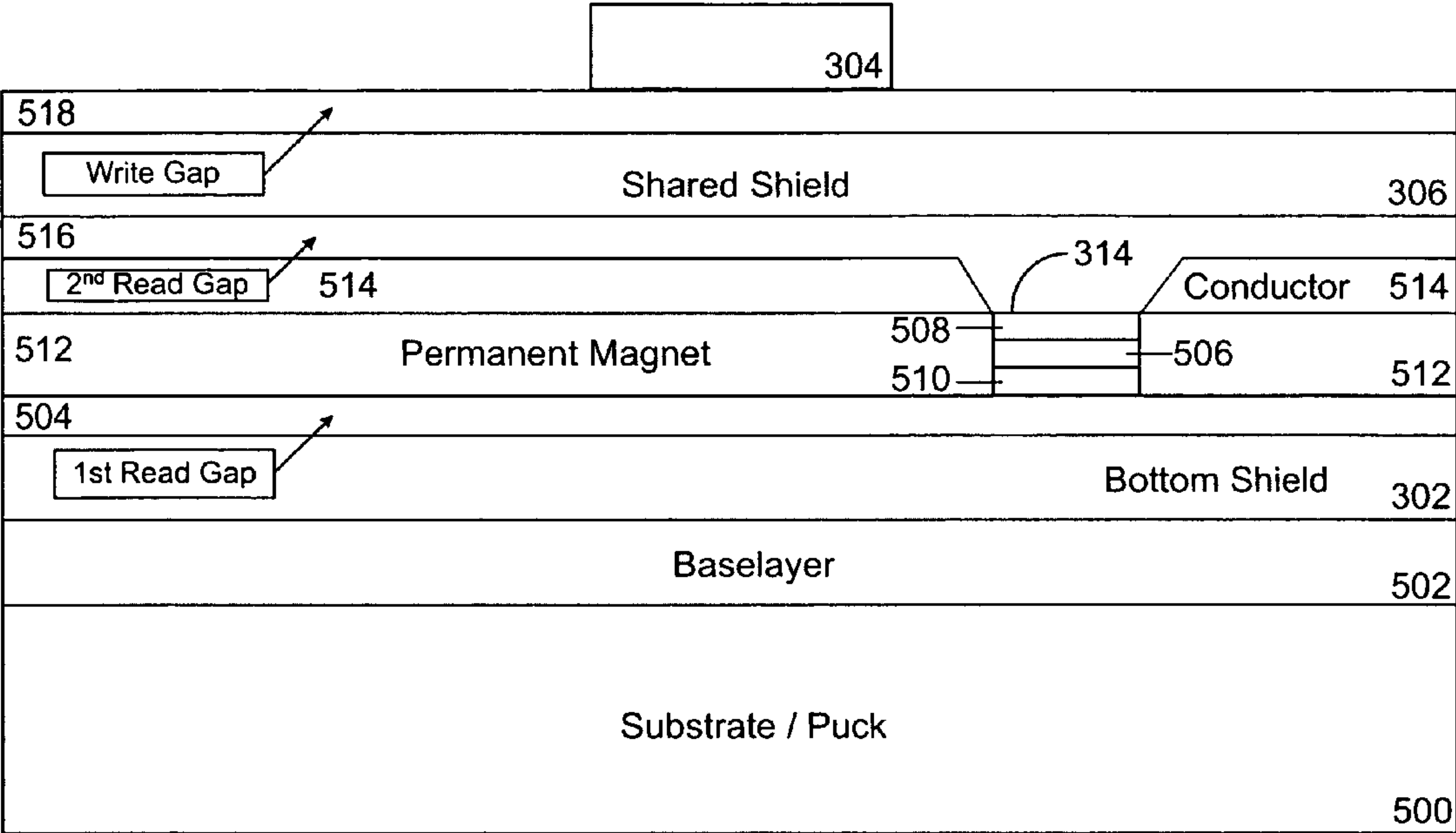
Tape Bearing Surface View
