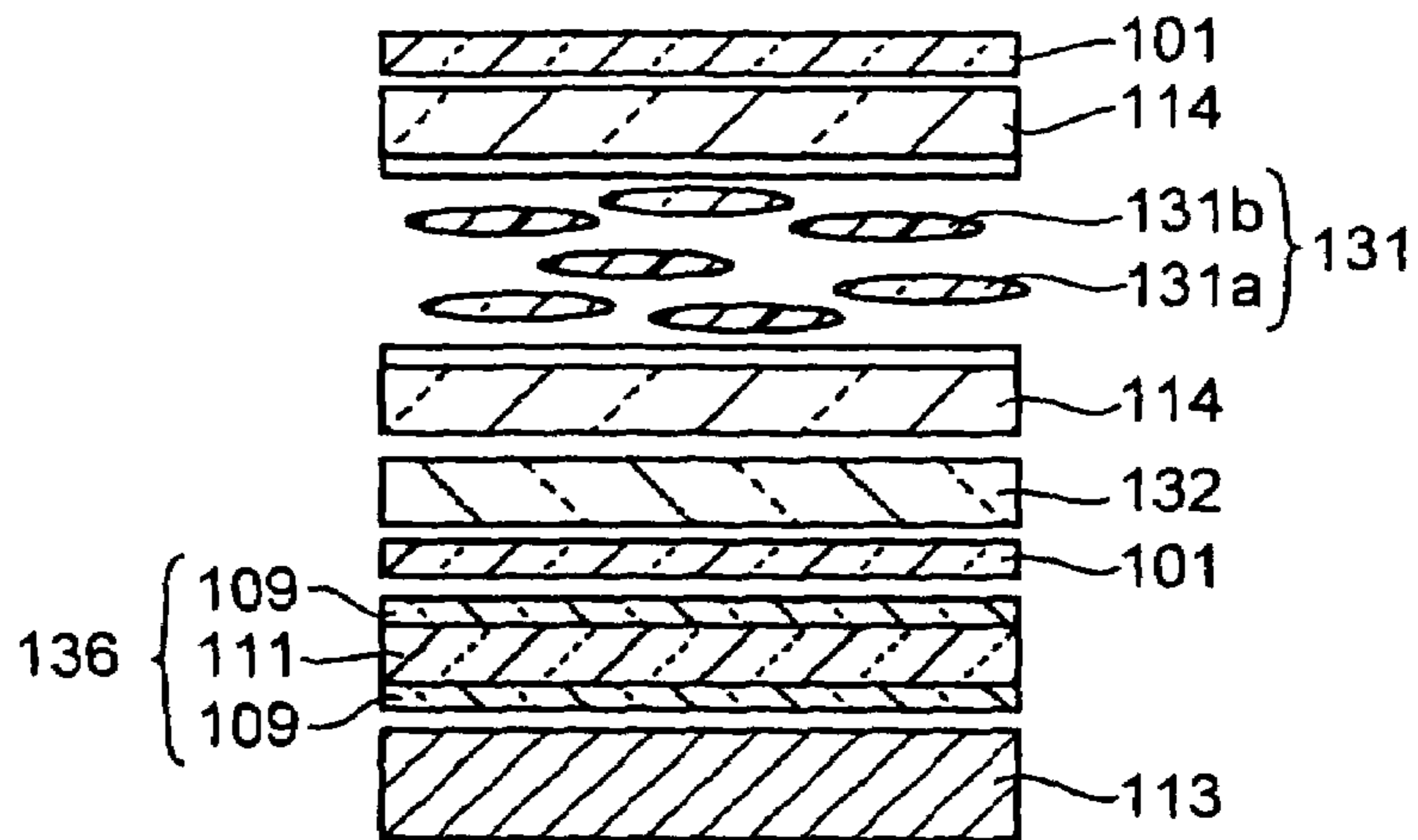
FIG. 25 PRIOR ART
