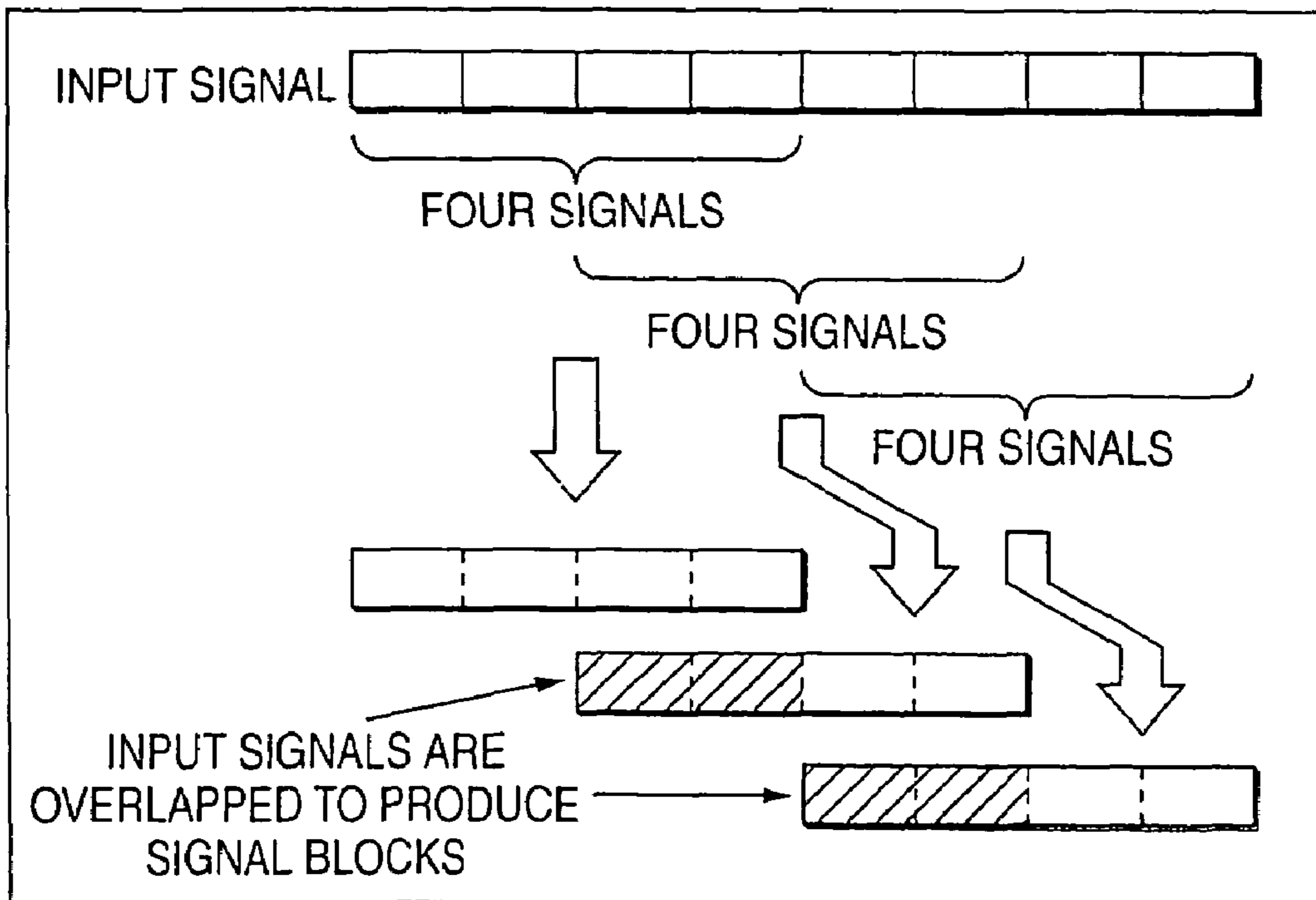
WAVELET TRANSFORMATION (IN CASE OF DIVISION NUMBER = 2, OVERLAPPING DEGREE = 2)
