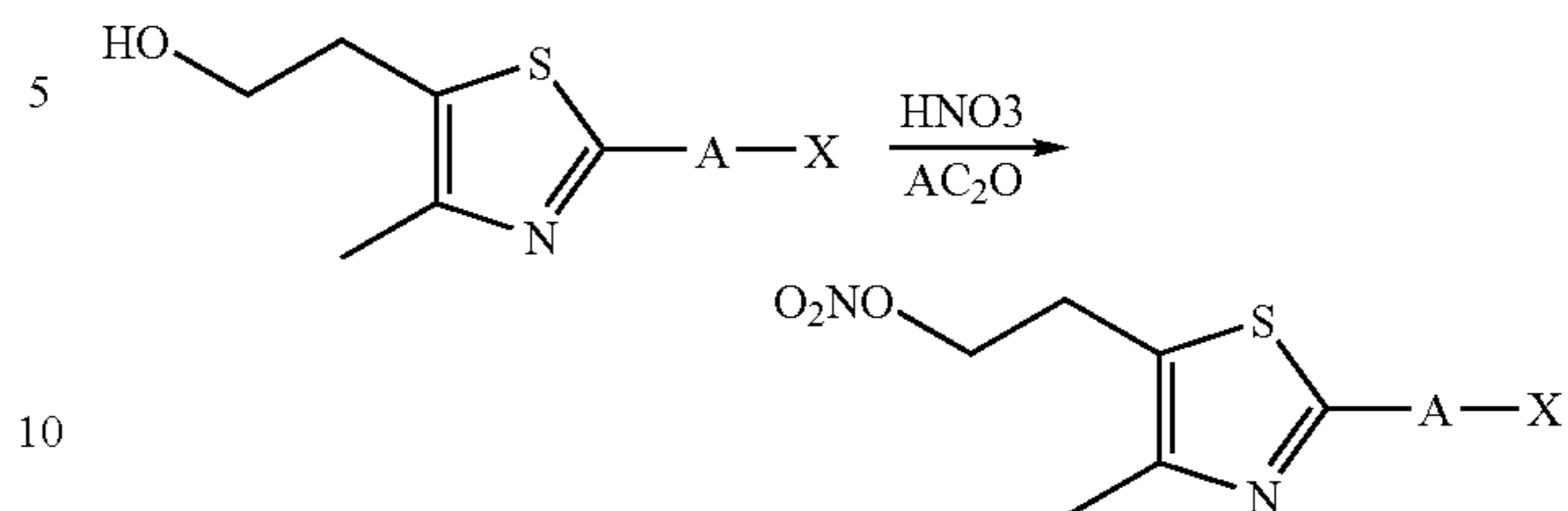
Scheme 11
