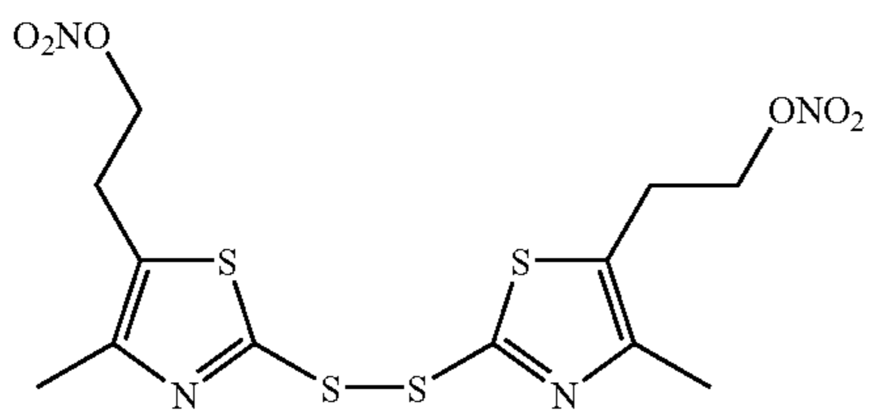
Bis-[4-methyl-5-(2-nitrooxy-ethyl)-thiazol-2-yl]-disulfide (Pet-54);
