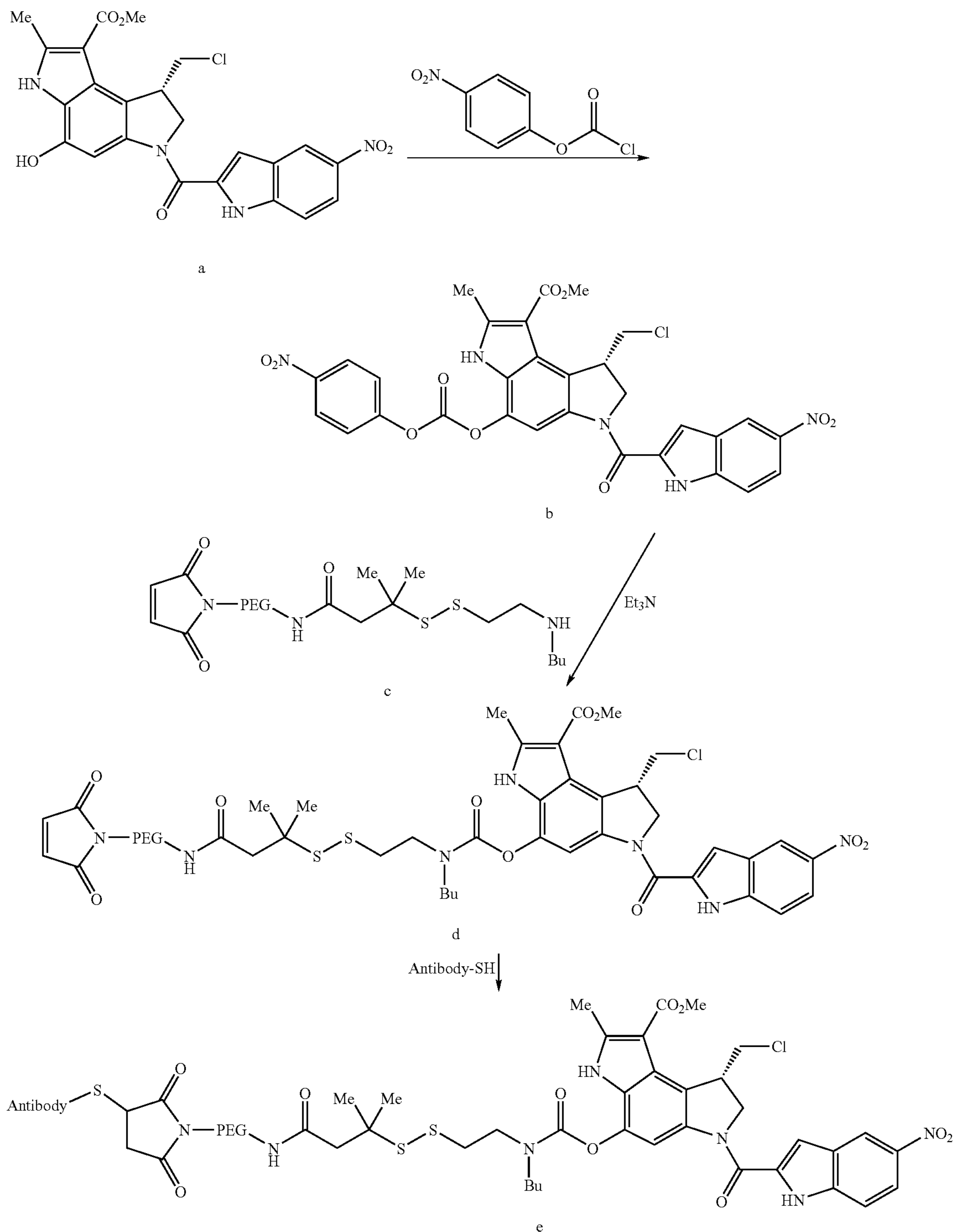
Scheme 7
