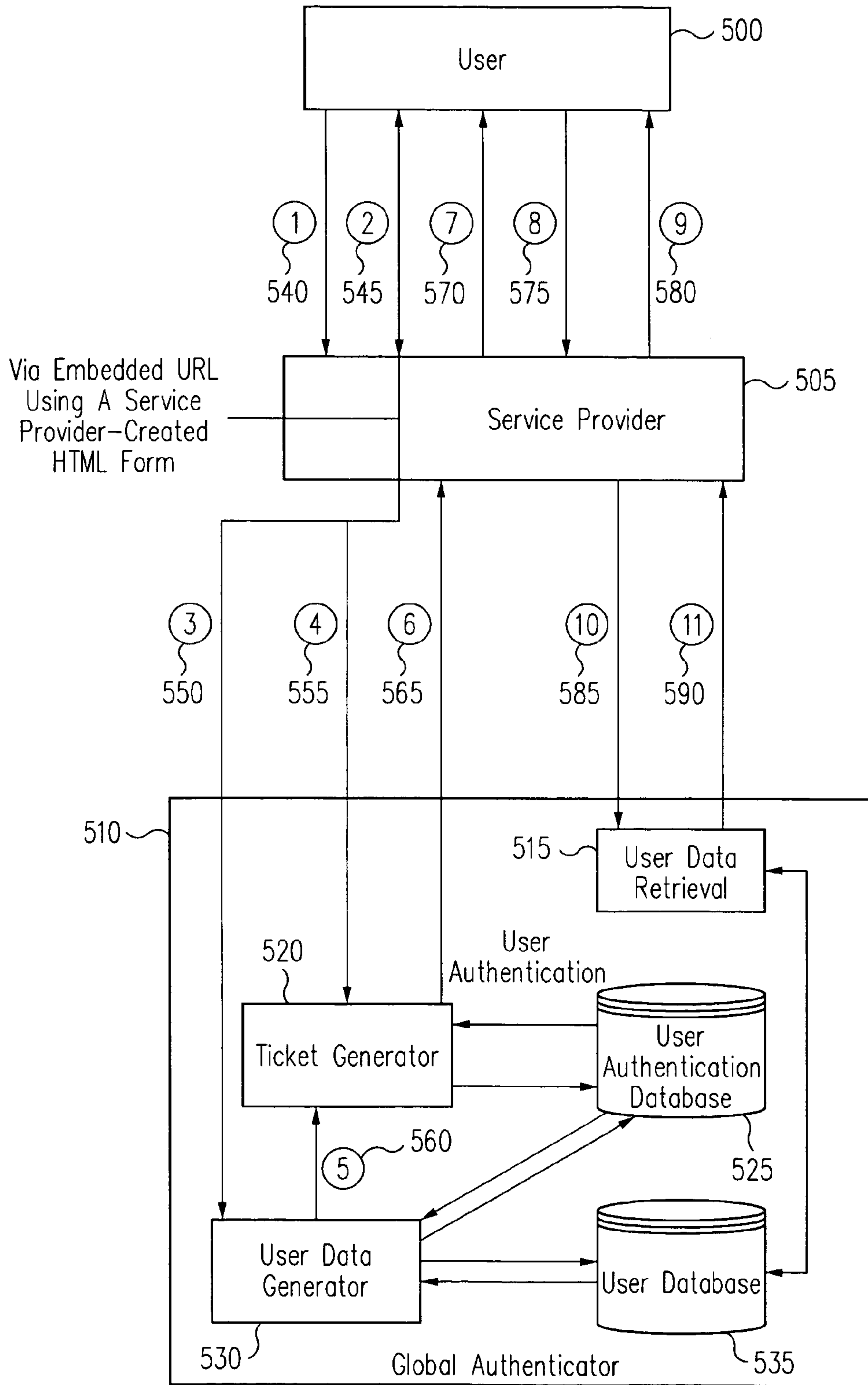
FIG. 5 (PRIOR ART)
