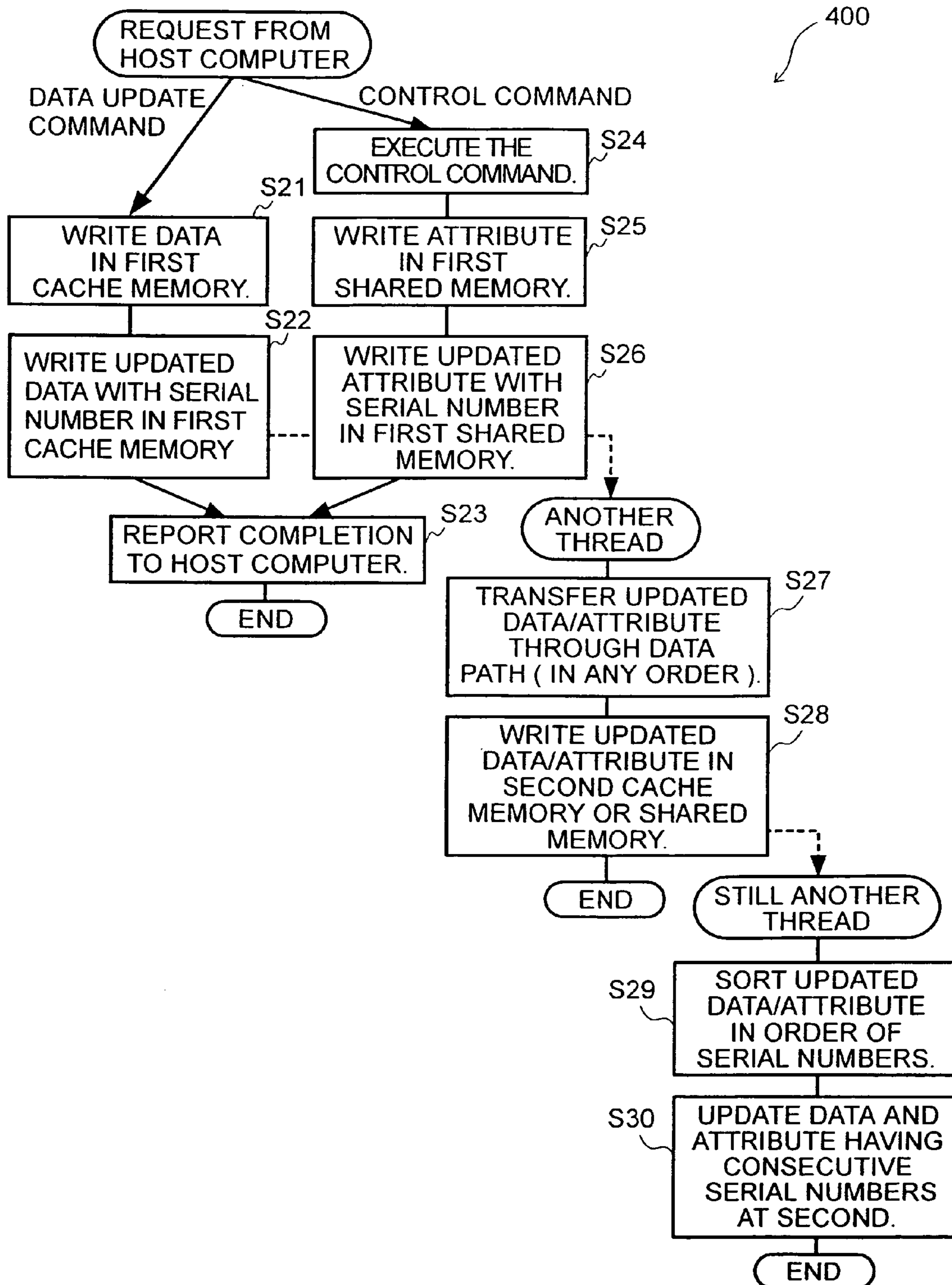
ASYNCHRONOUS TRANSFER FLOWCHART
