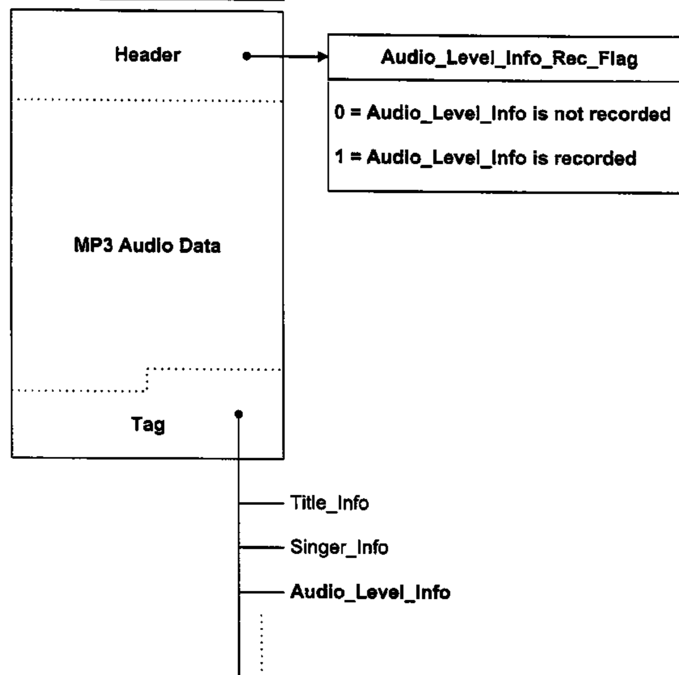
MP3 Audio File Structure
