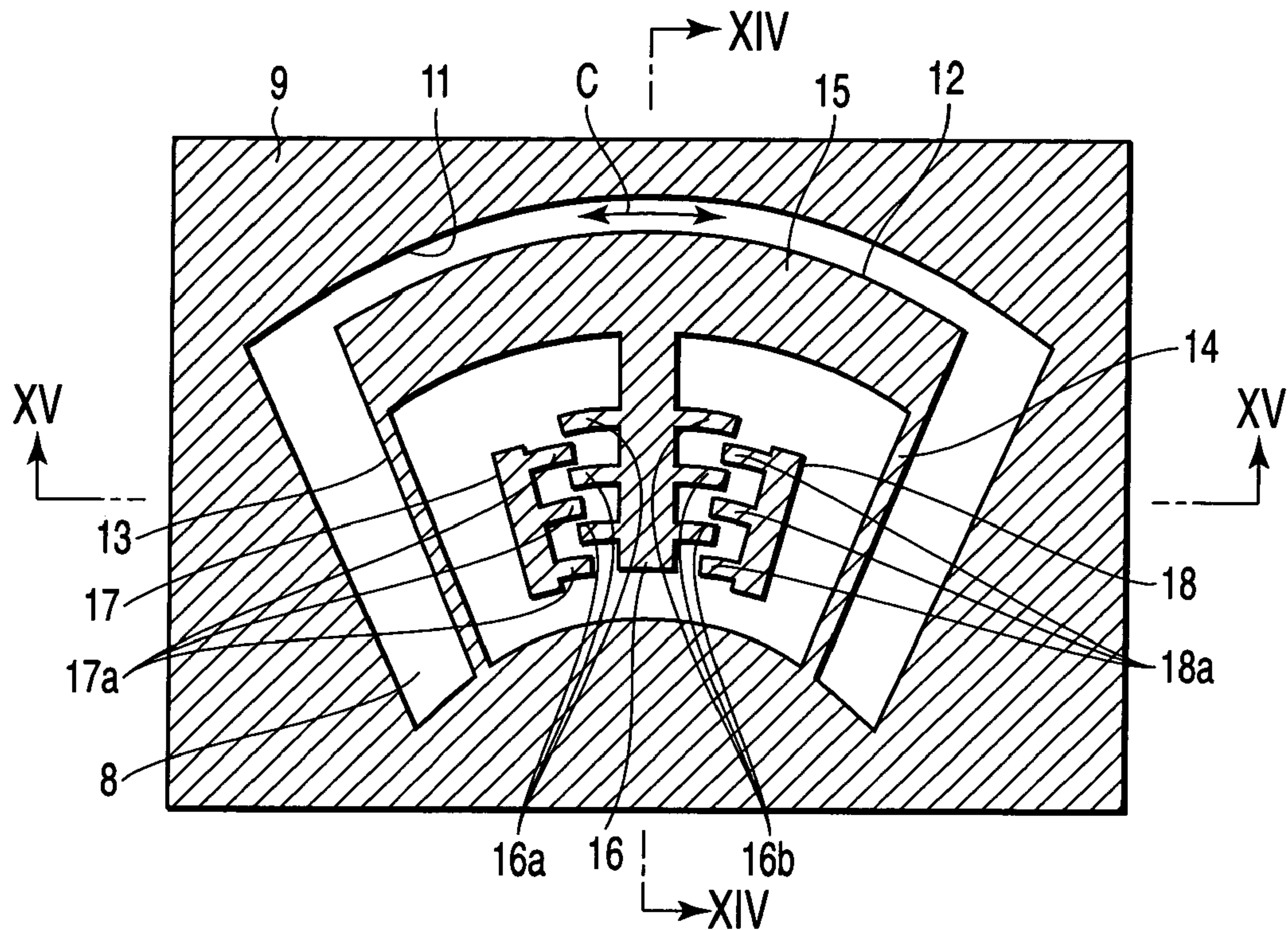
FIG. 13 PRIOR ART
