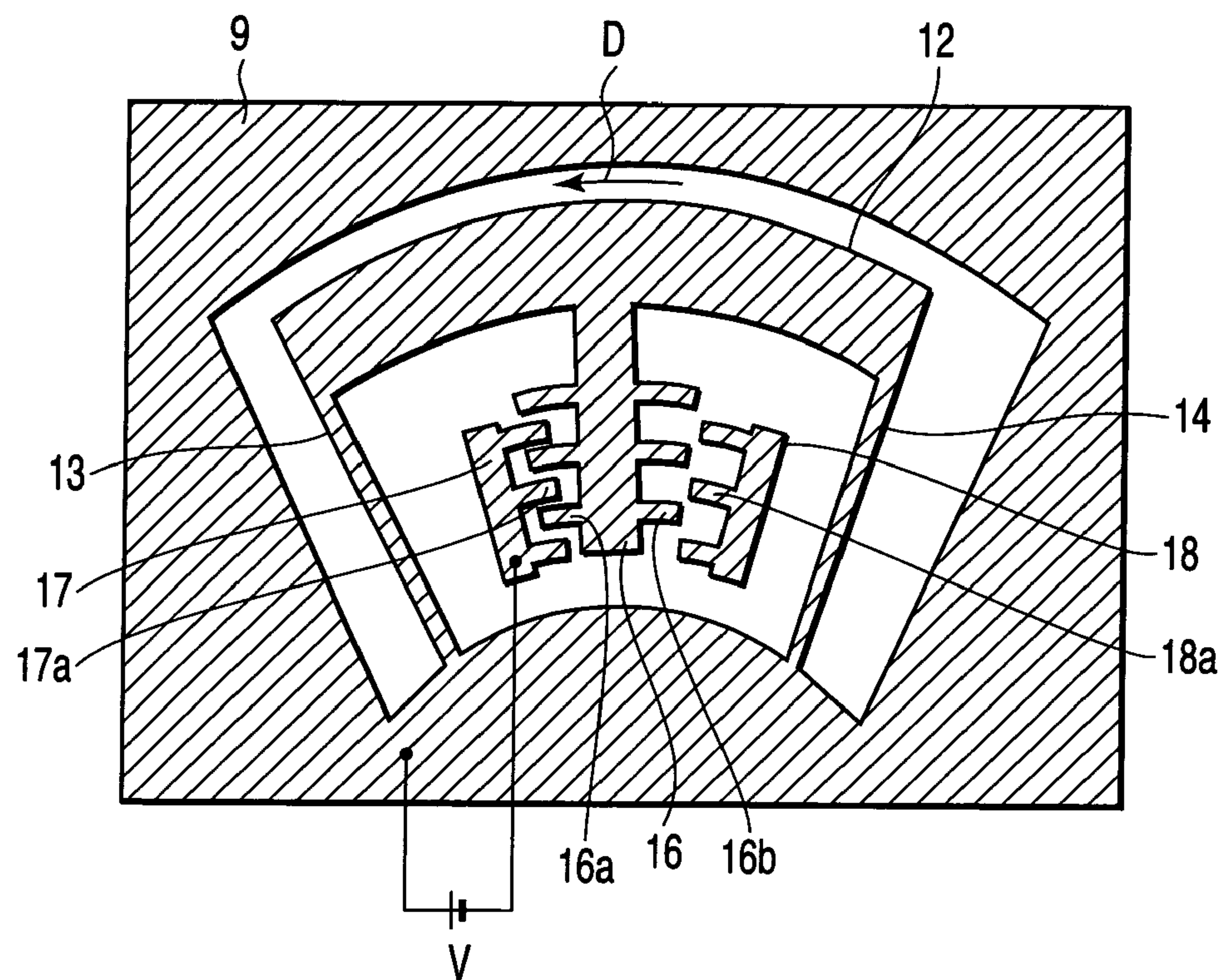
FIG. 16 PRIOR ART
