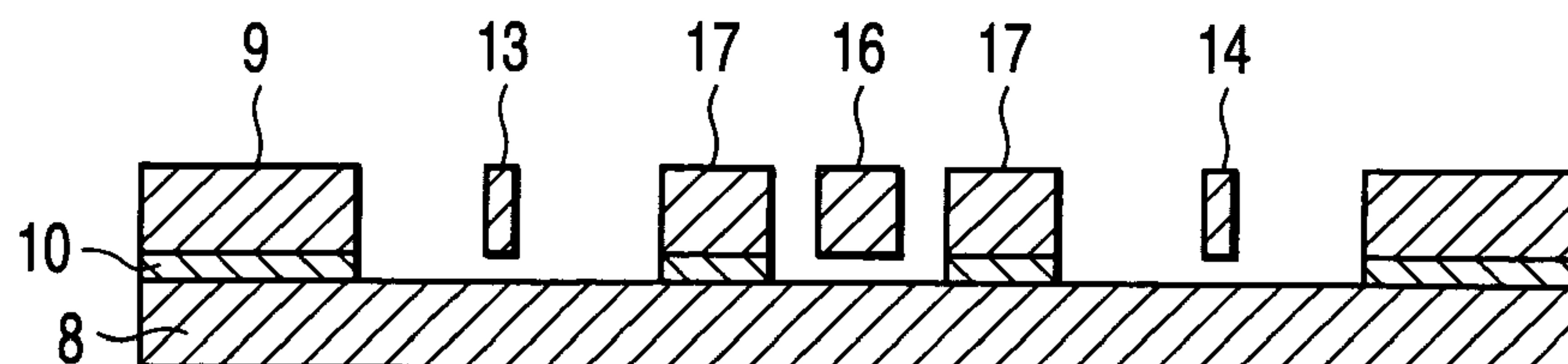
FIG. 15 PRIOR ART
