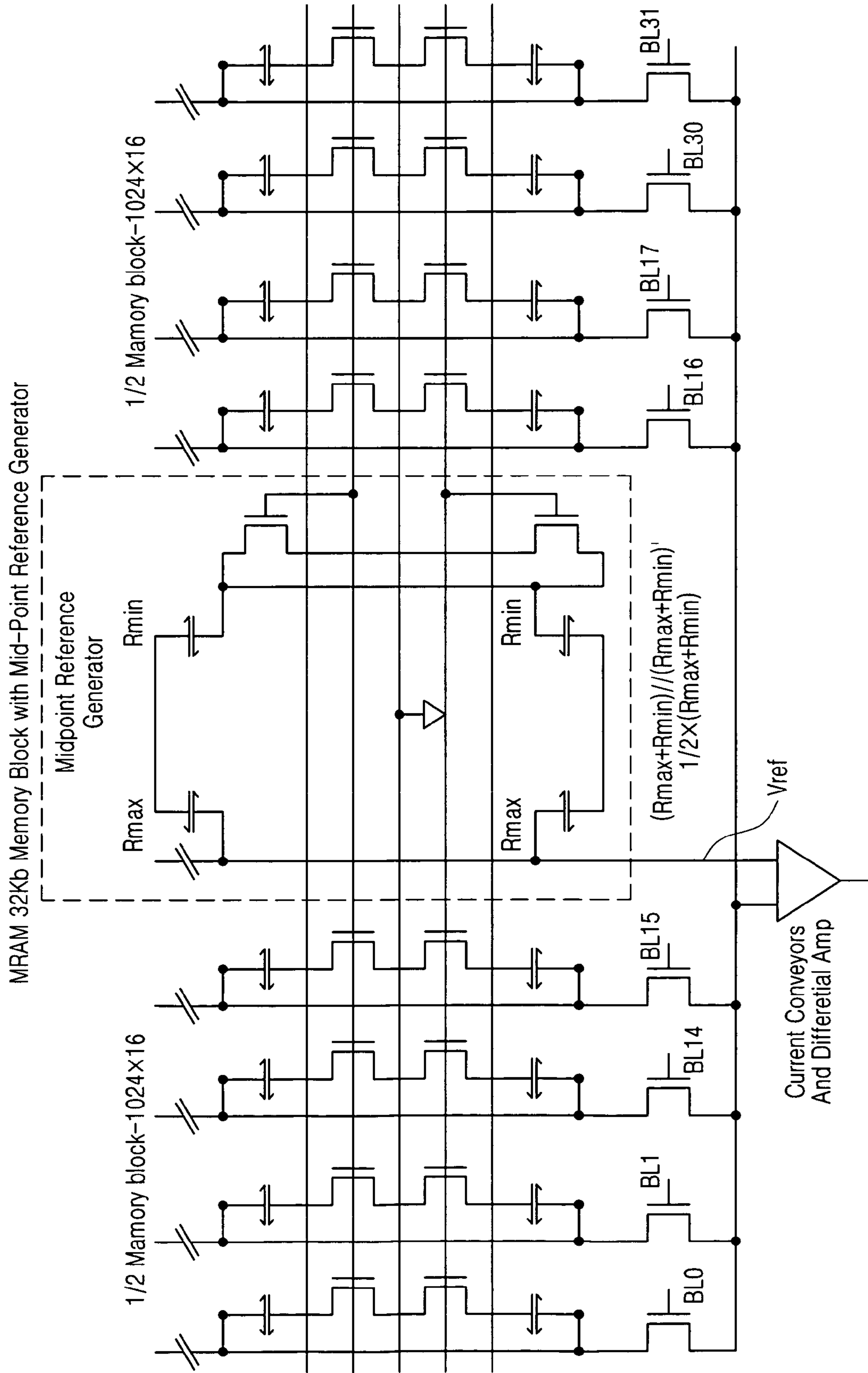
FIG. 2 (PRIOR ART)
