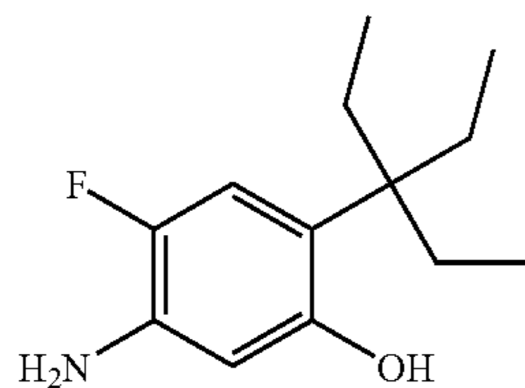
C-19; 5-Amino-2-(3-ethylpentan-3-yl)-4-fluorophenol
