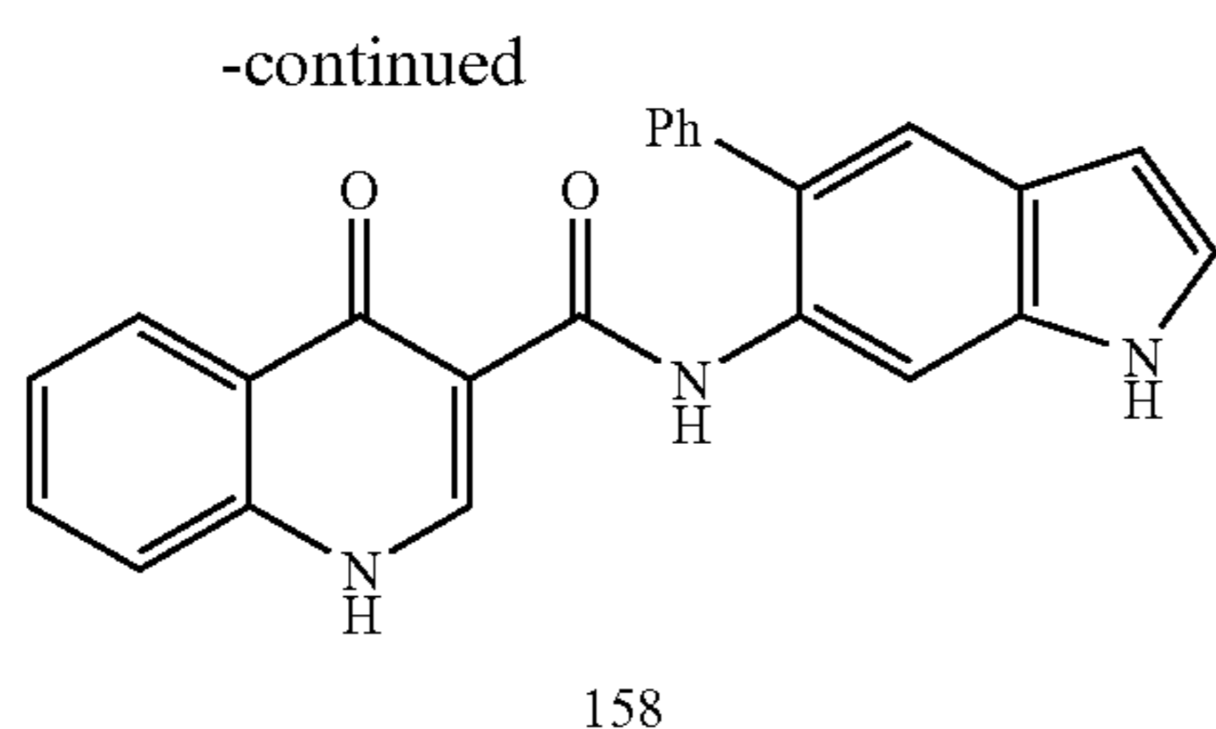
158; 4-Oxo-N-(5-phenyl-1H-indol-6-yl)-1H-quinoline-3-carboxamide
