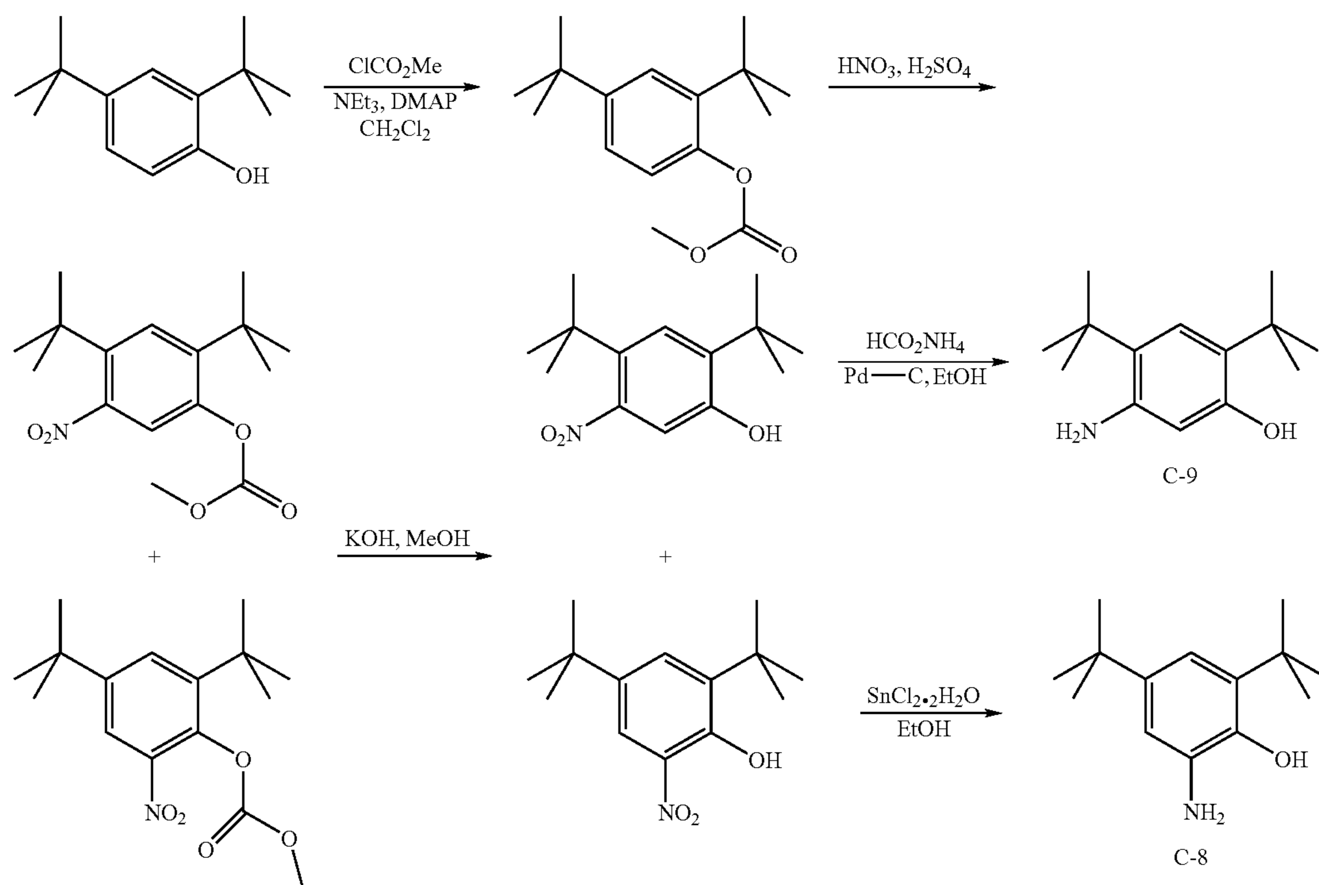
Carbonic acid 2,4-di-tert-butyl-phenyl ester methyl ester
