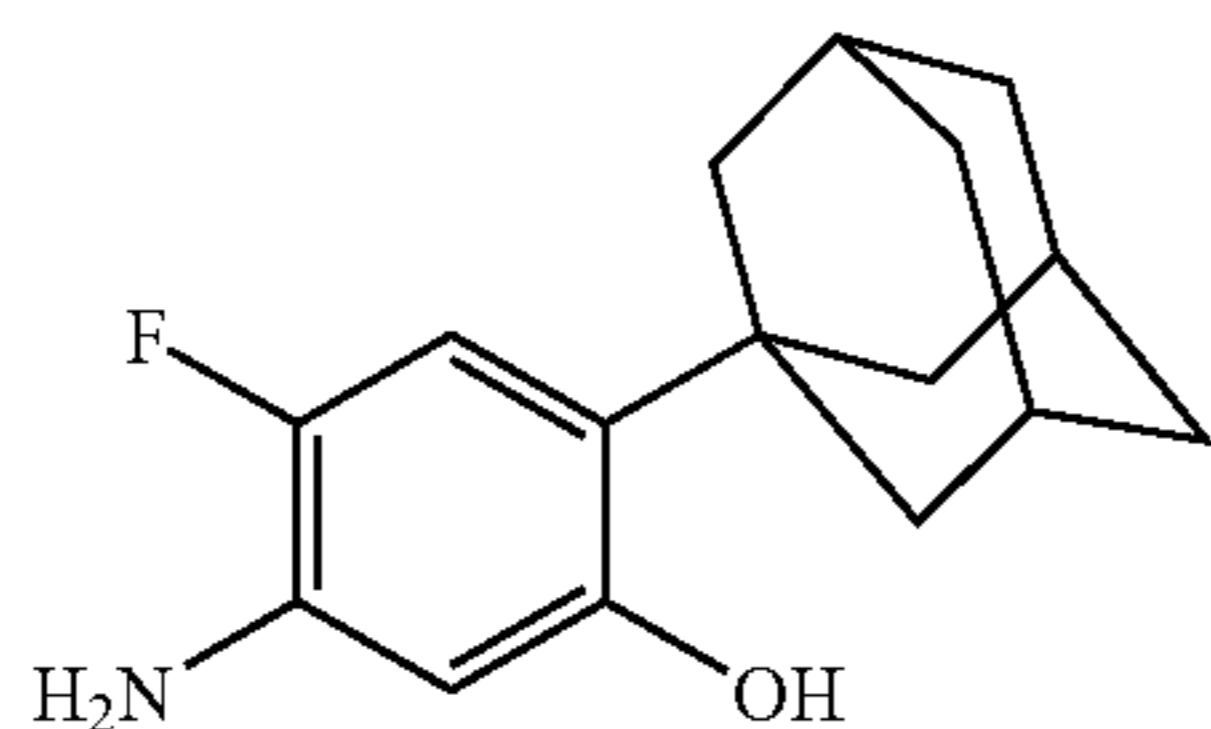
C-20; 2-Admantyl-5-amino-4-fluorophenol
