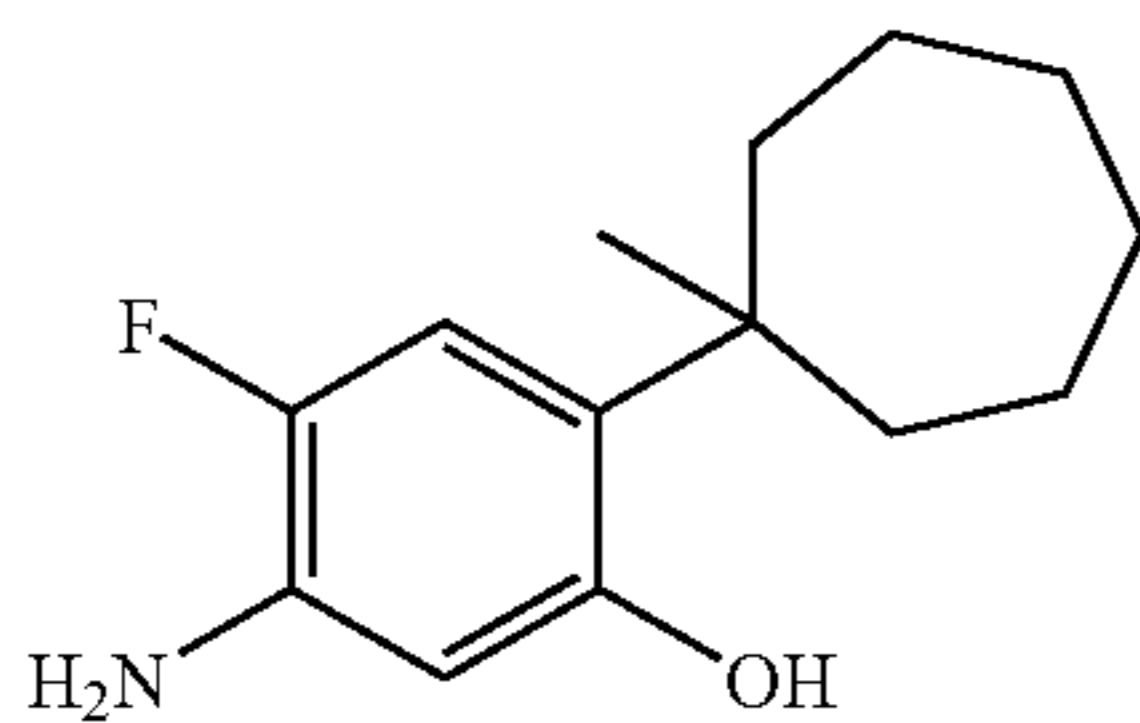
C-21; 5-Amino-4-fluoro-2-(1-methylcycloheptyl)phenol
