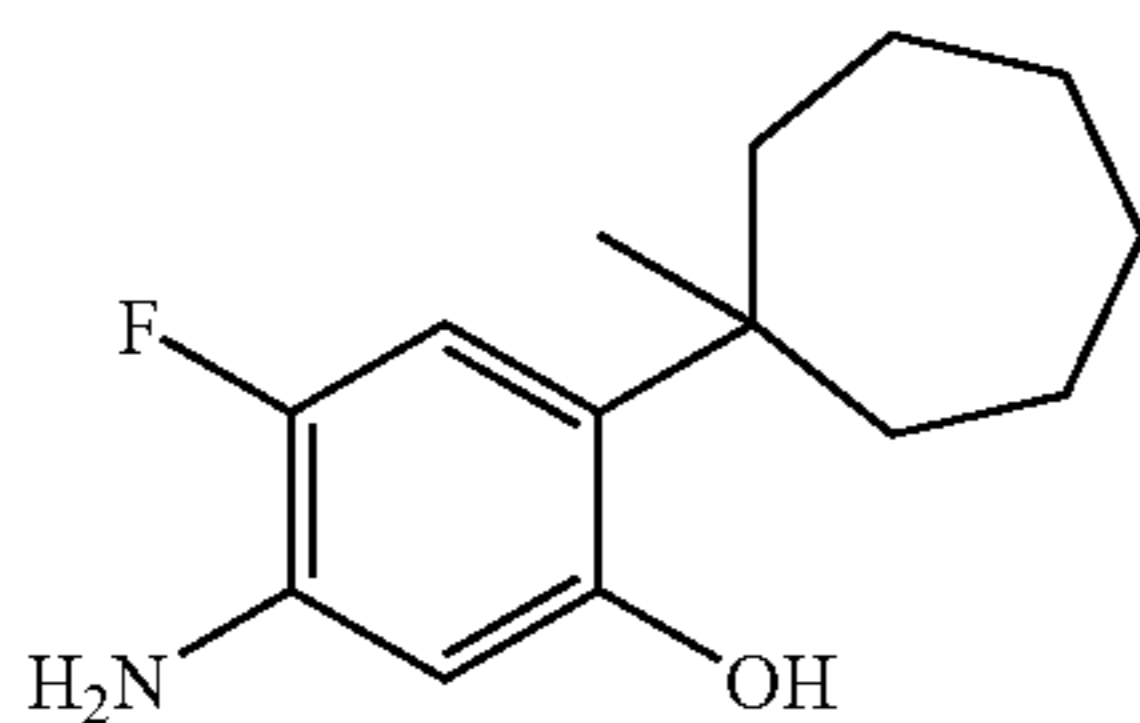
C-22; 5-Amino-4-fluoro-2-(1-methylcyclooctyl)phenol
