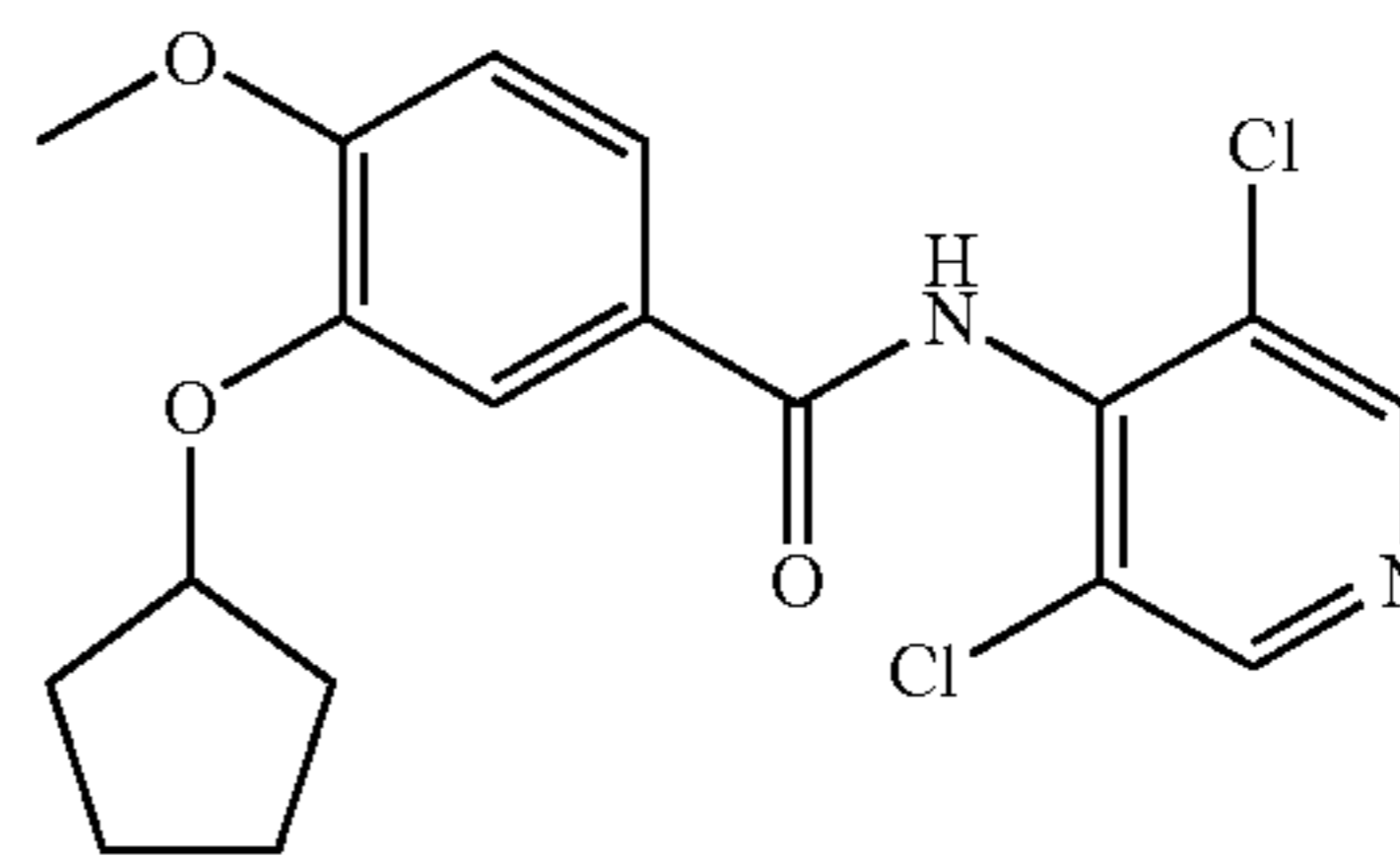
piclamilast
