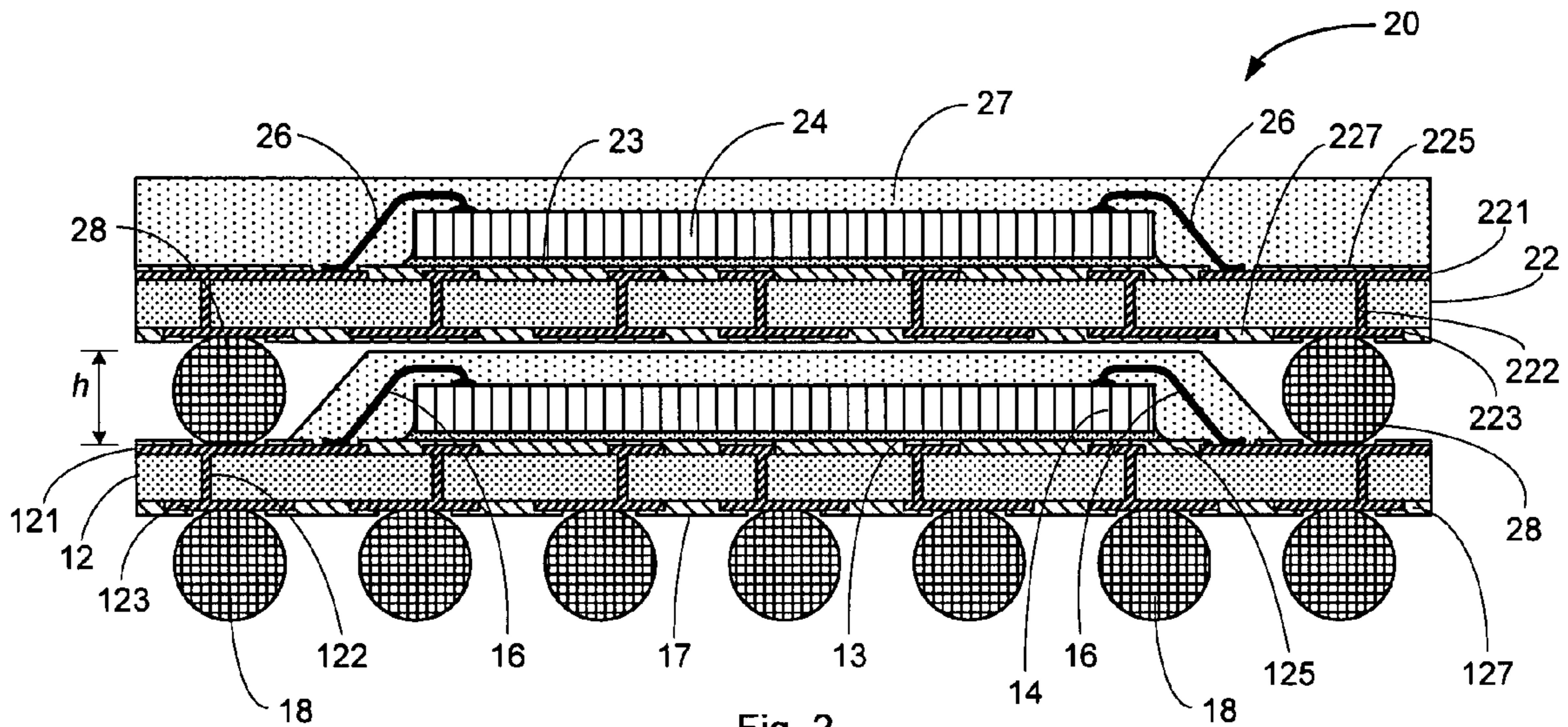
Fig. 2 PRIOR ART
