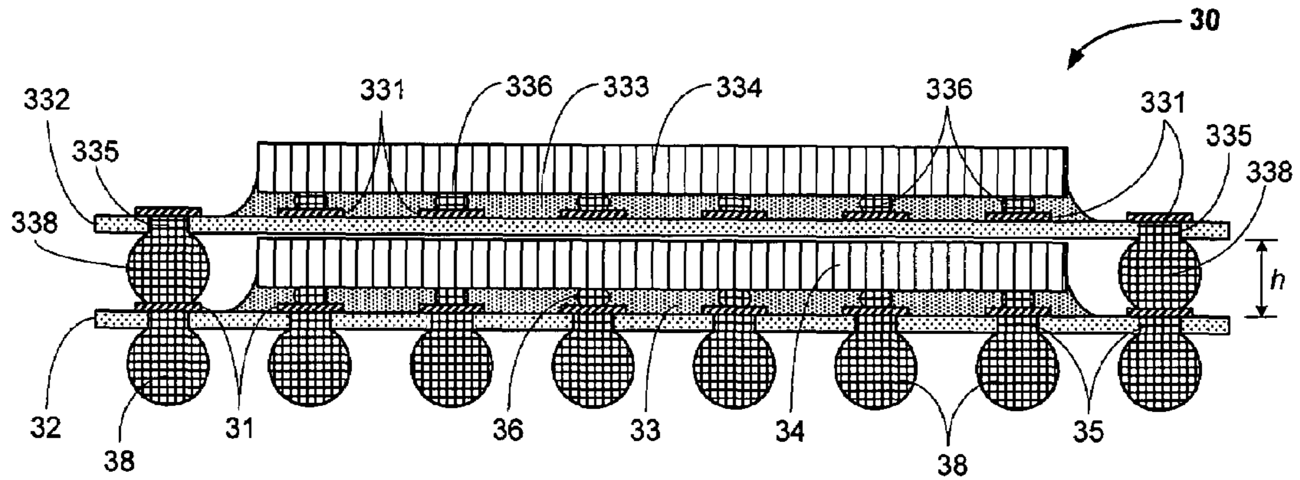
Fig. 3 PRIOR ART
