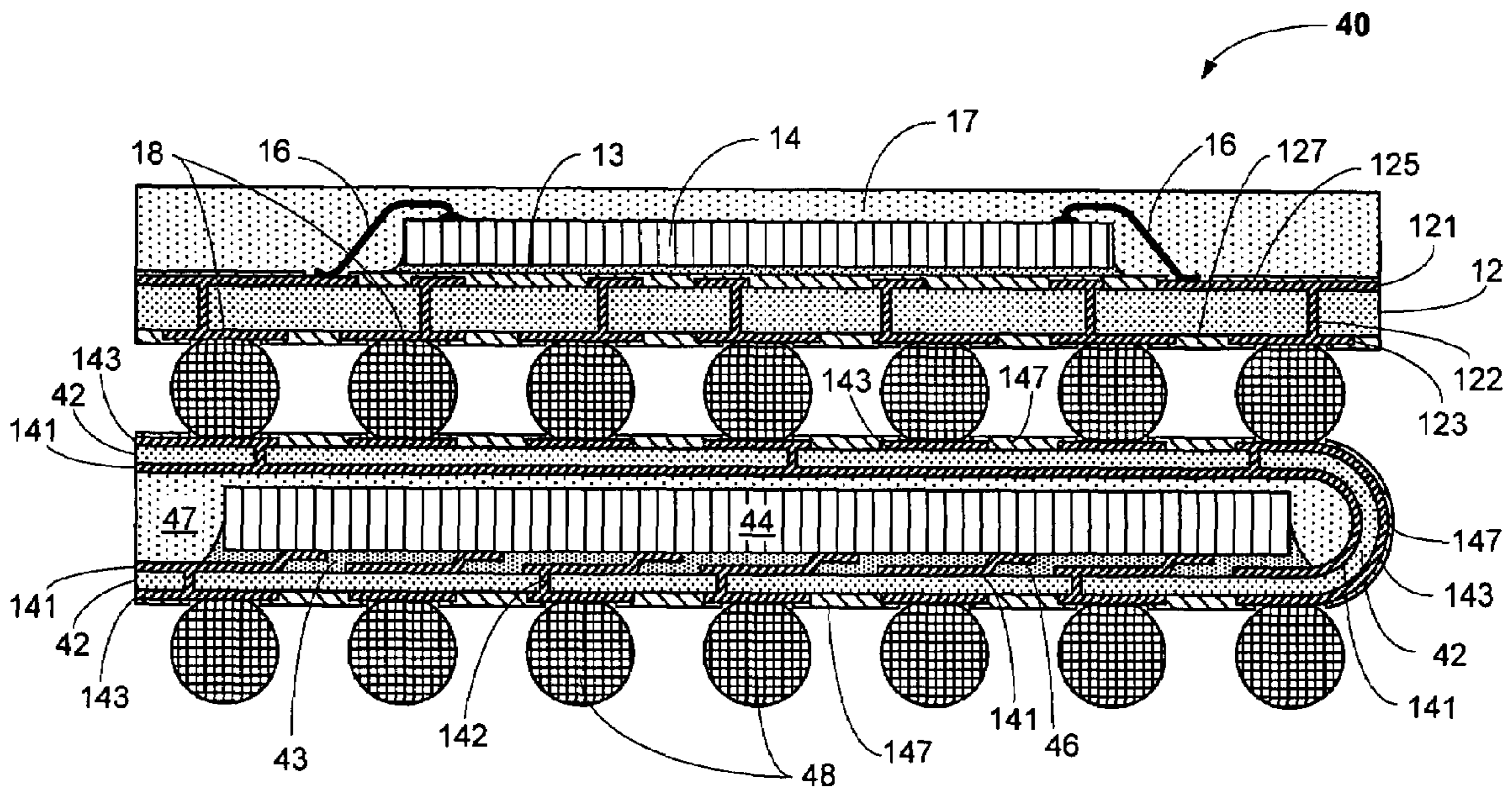
Fig. 4 PRIOR ART
