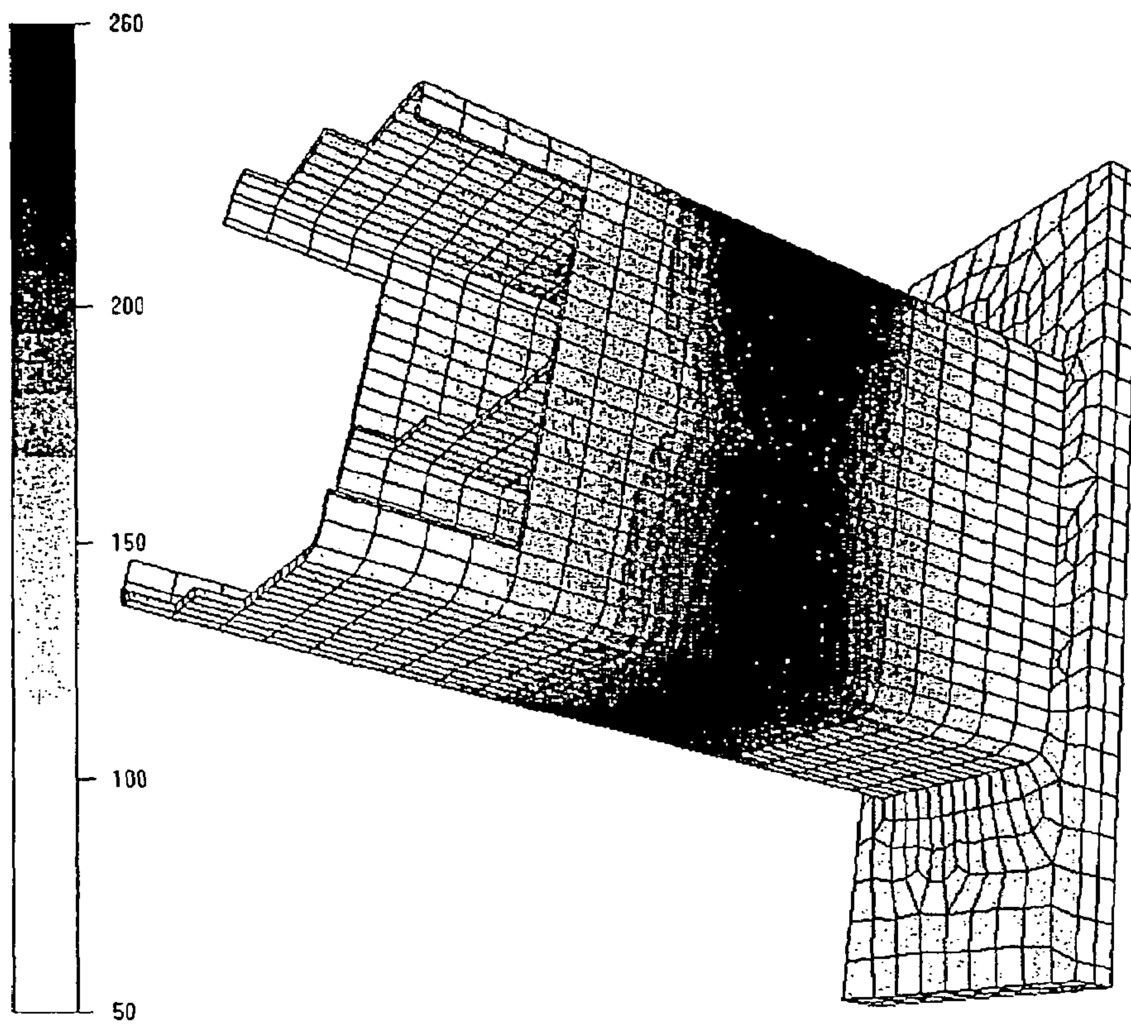
Temperature field [C°]
