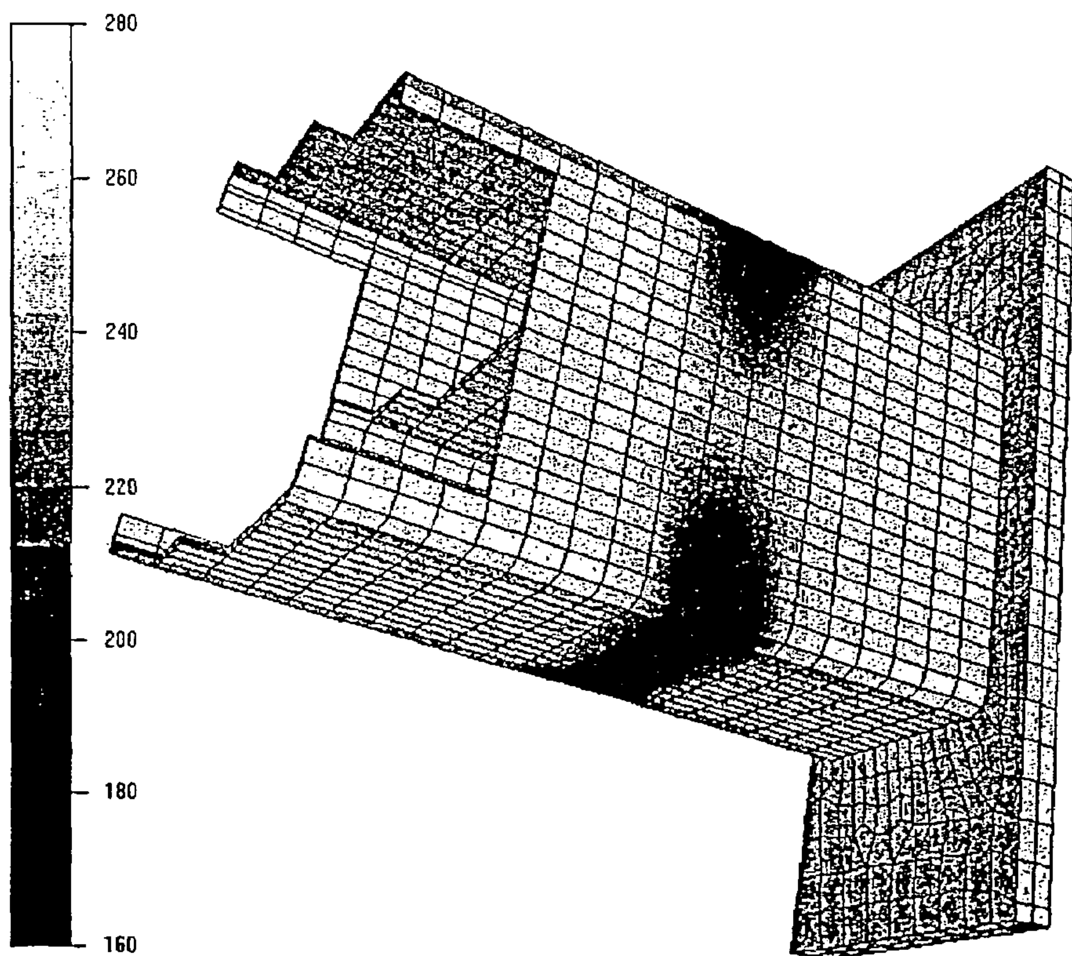
Yield stress [MPa]
