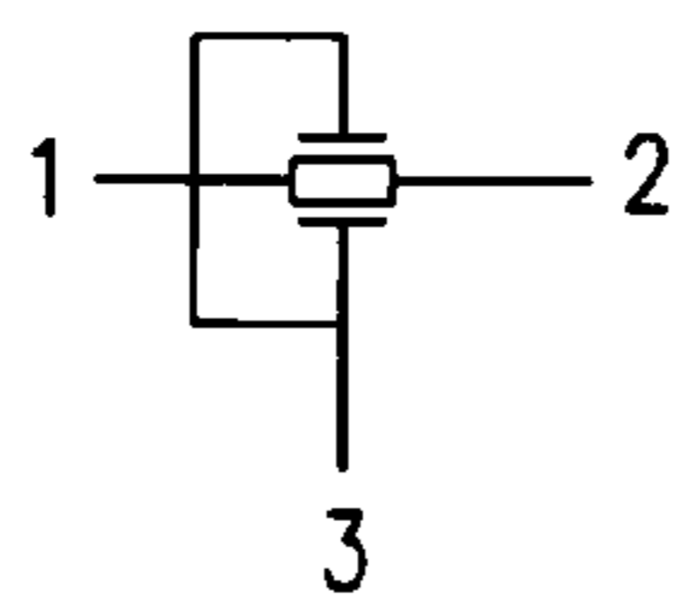
TRANSMISSION GATE STYLE SWITCH (S)
