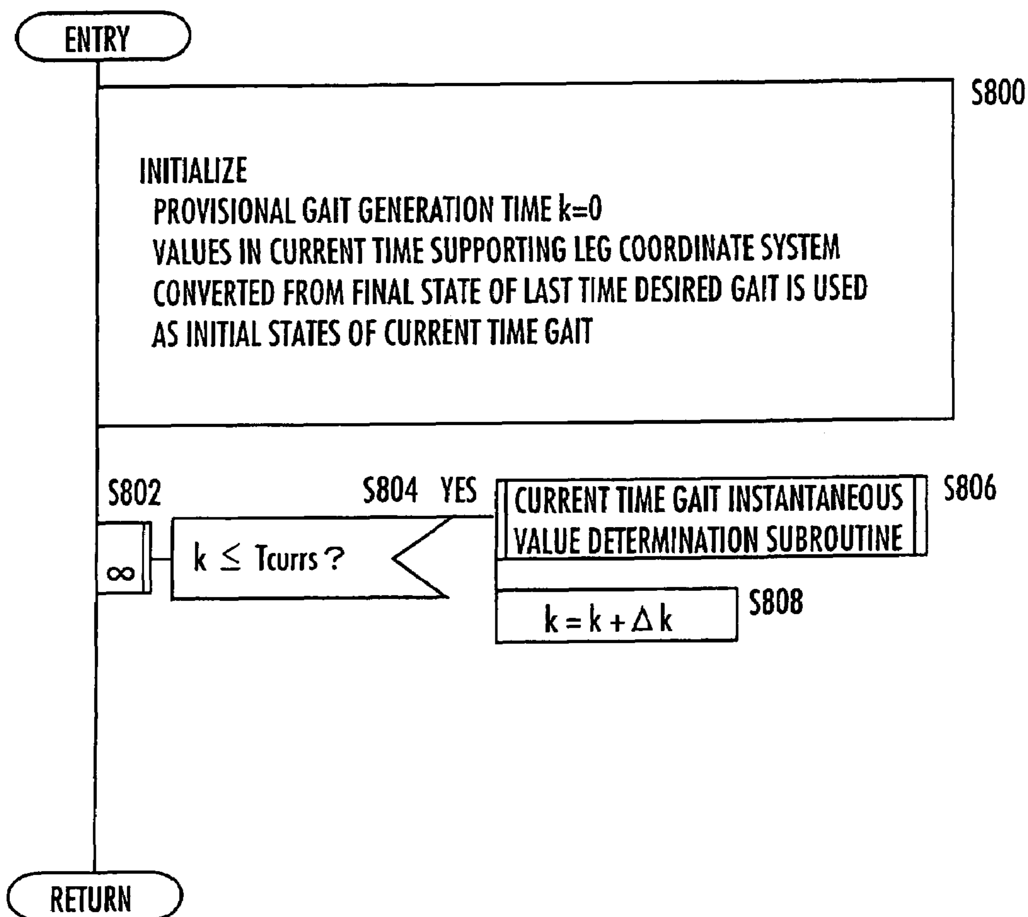
FIG.35 ( PROCESS OF GENERATING PROVISIONAL CURRENT TIME GAIT )
