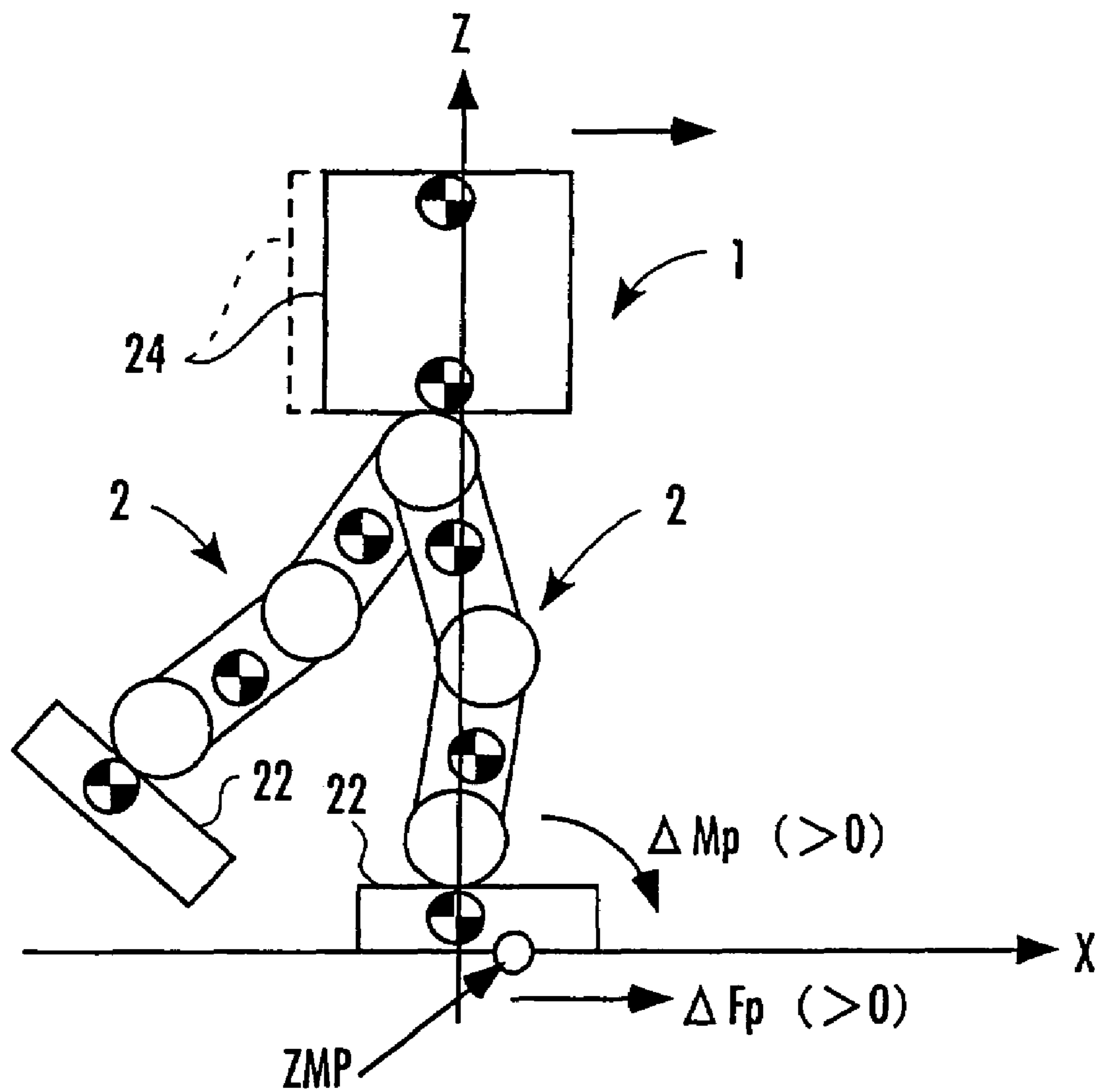
FIG.8 ( BODY TRANSLATION MODE )
