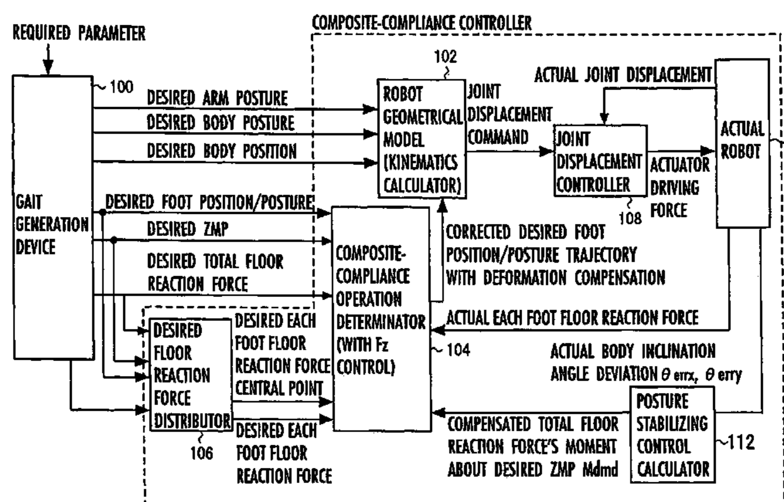
(FUNCTIONAL BLOCK DIAGRAM OF LEGGED MOBILE ROBOT)
