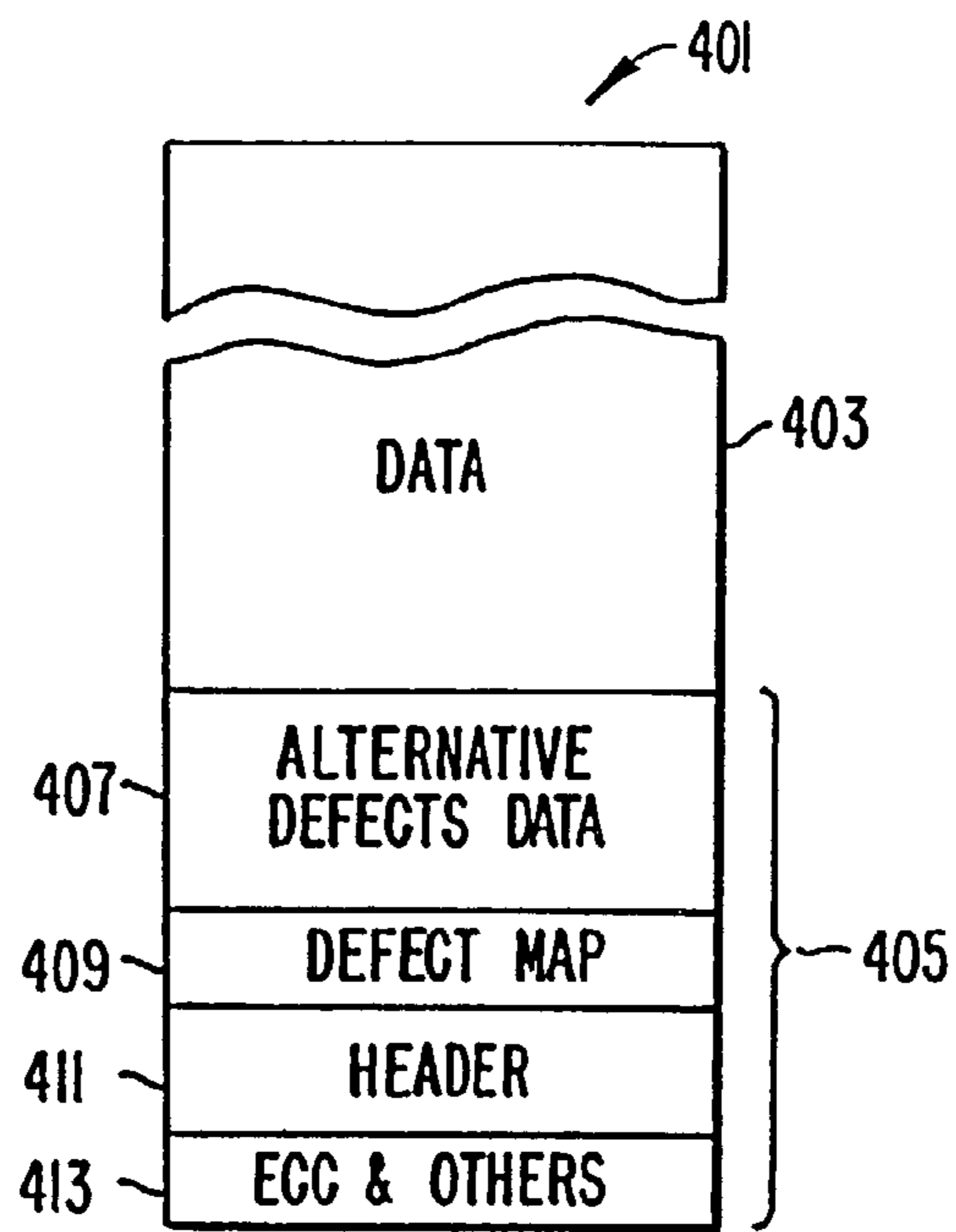
SECTOR PARTITION FIG. 5.
