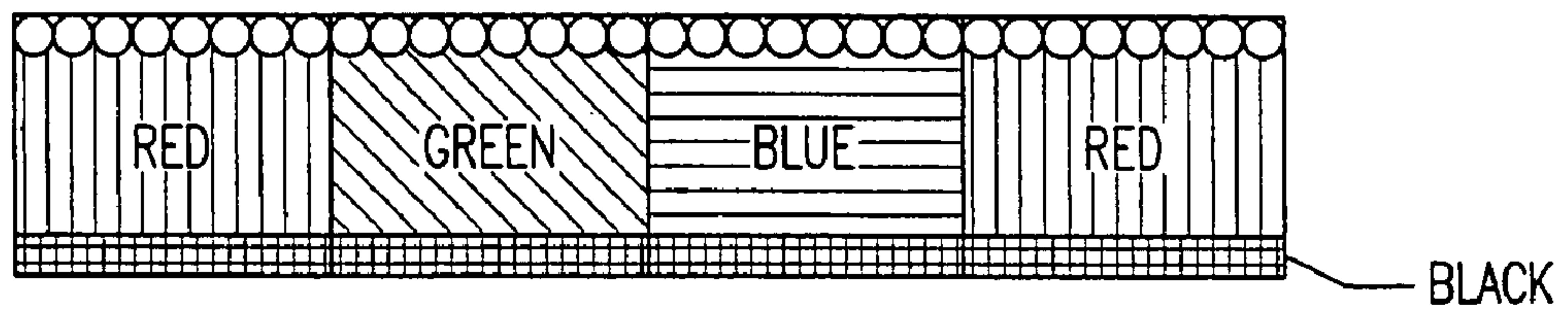
SIDE VIEW FIG. 7A
