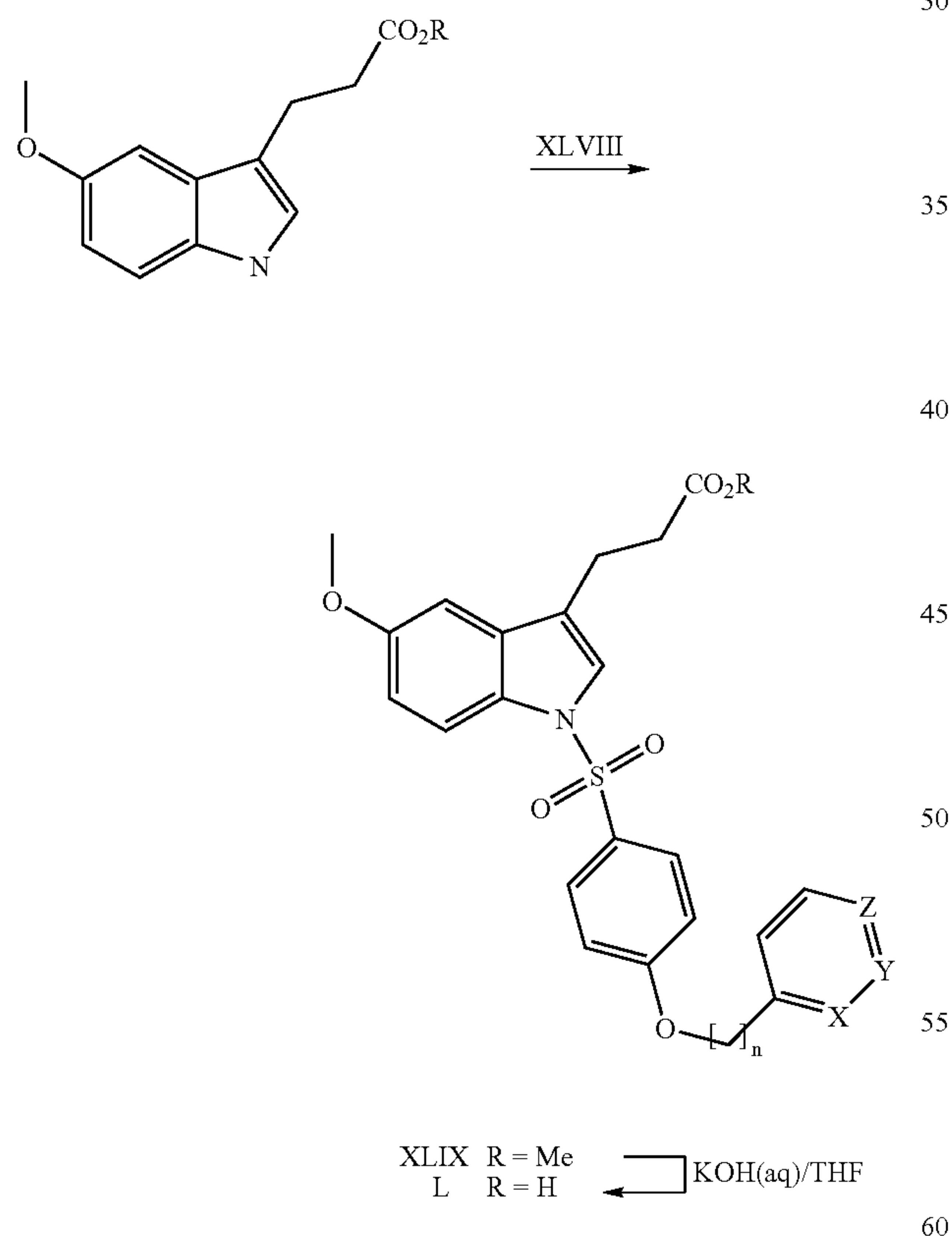
Scheme 23b- Preparation of Compound of Formula L
