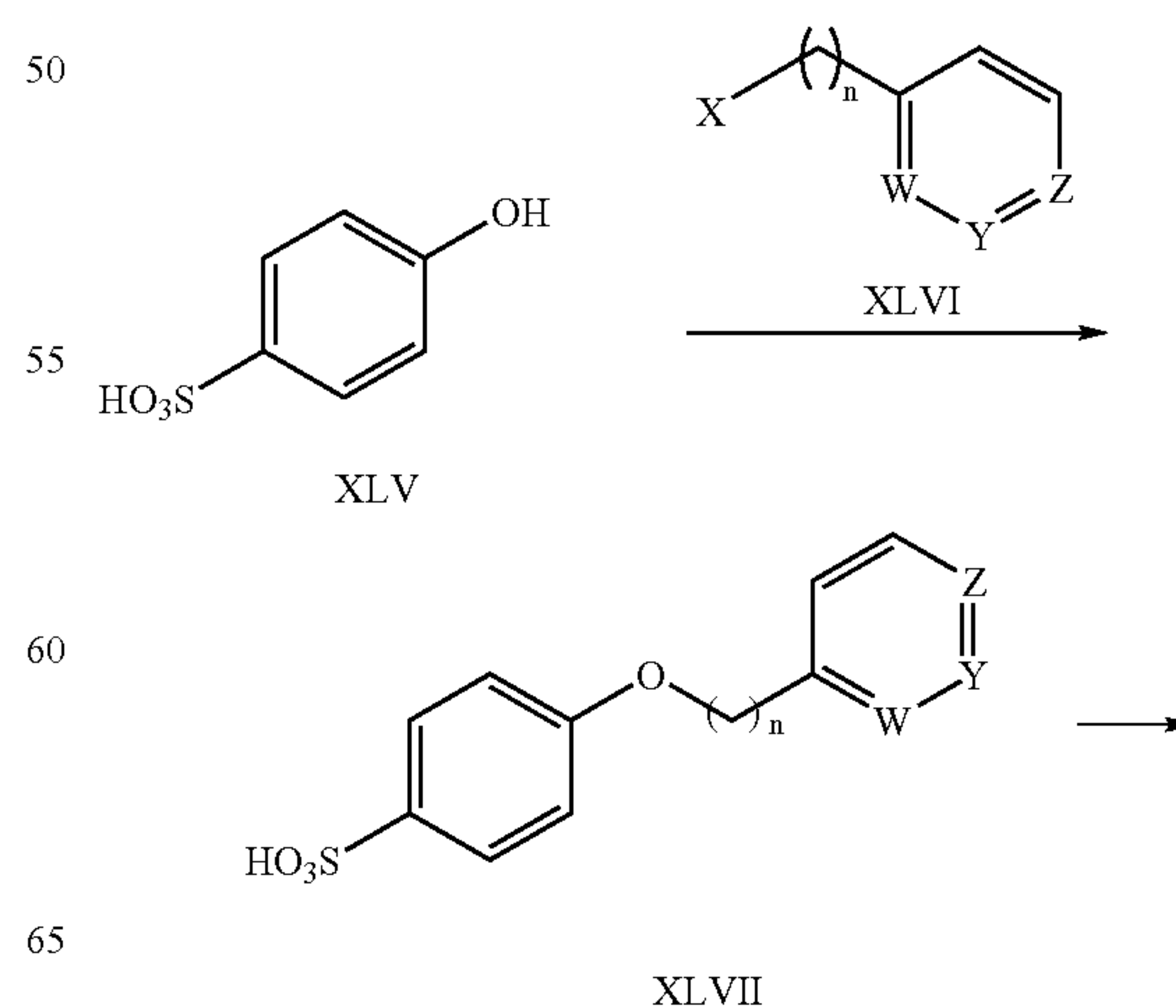
Scheme 23a- Preparation of sulfonyl chloride XLVIII:
