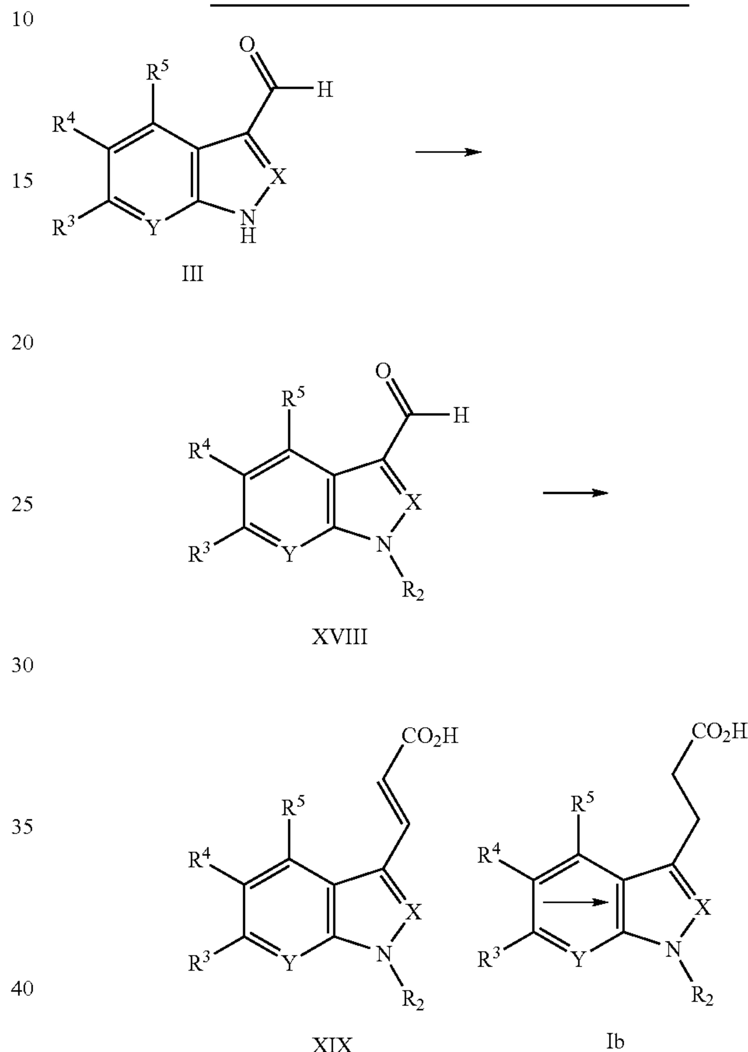
Scheme 11: Alternative synthesis methodology for Compounds of Formula Ib
