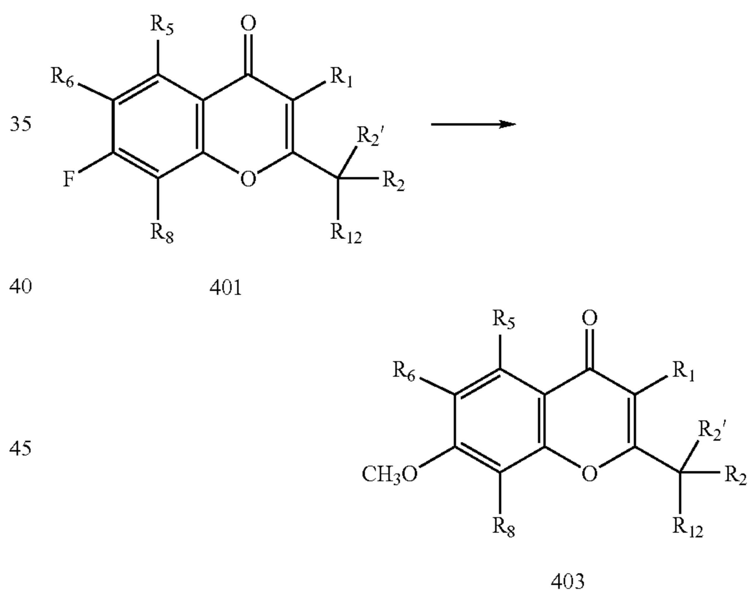
Reaction Scheme 4
