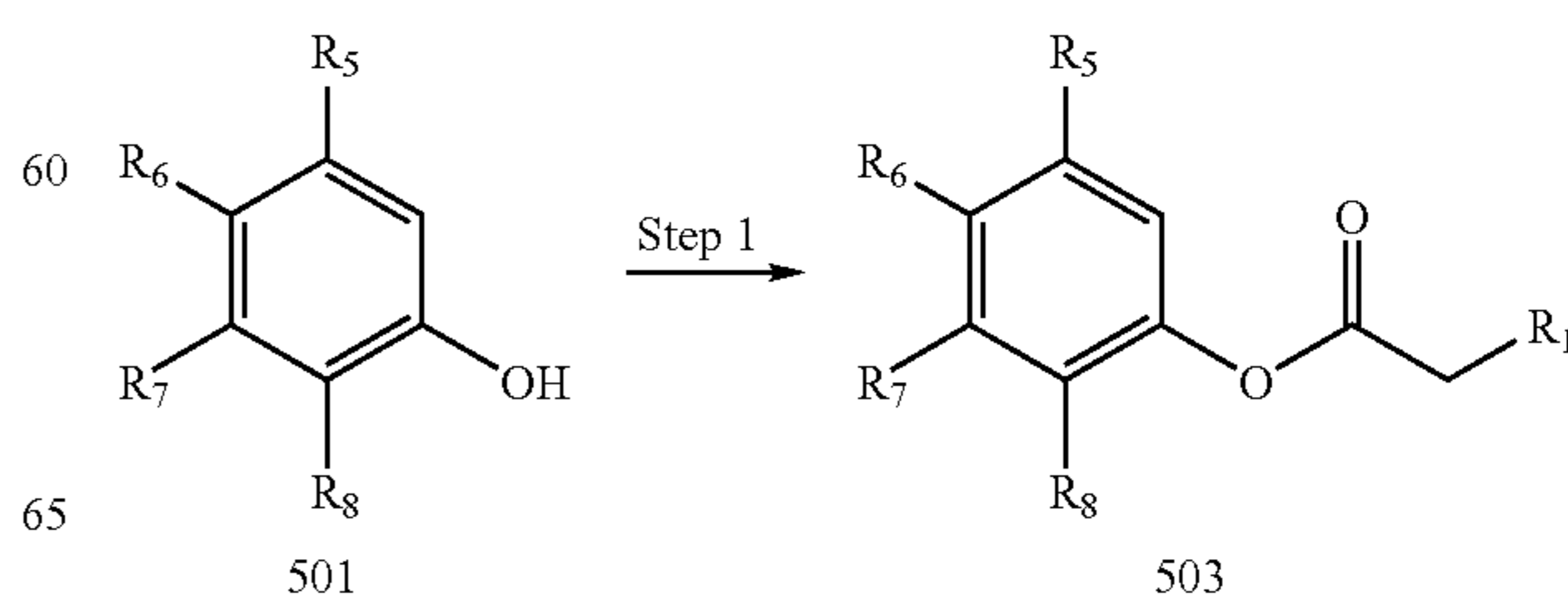
Reaction Scheme 5
