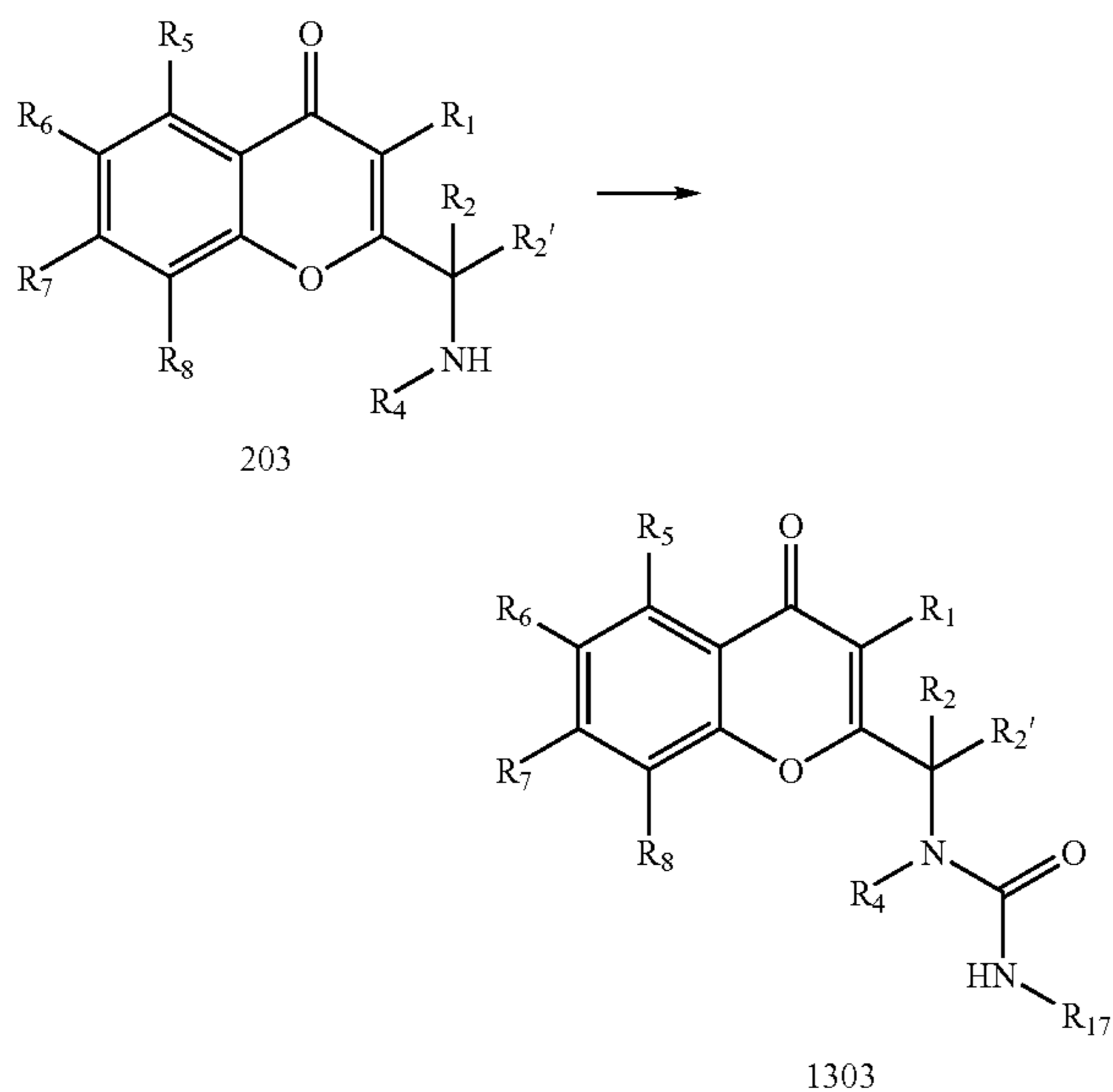
Reaction Scheme 13
