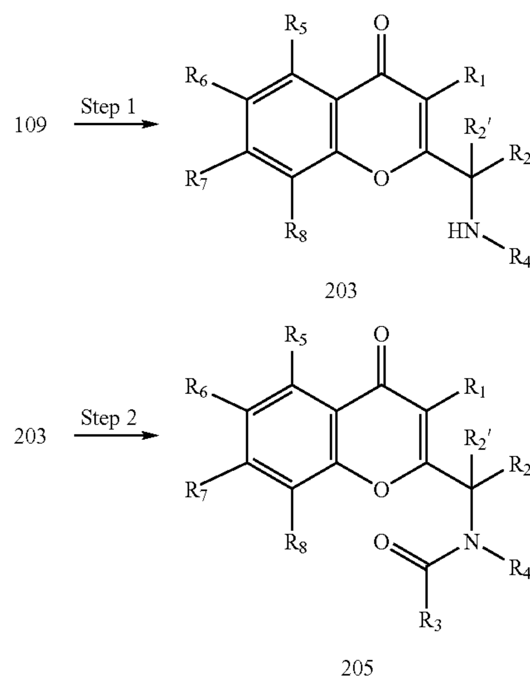
Reaction Scheme 2
