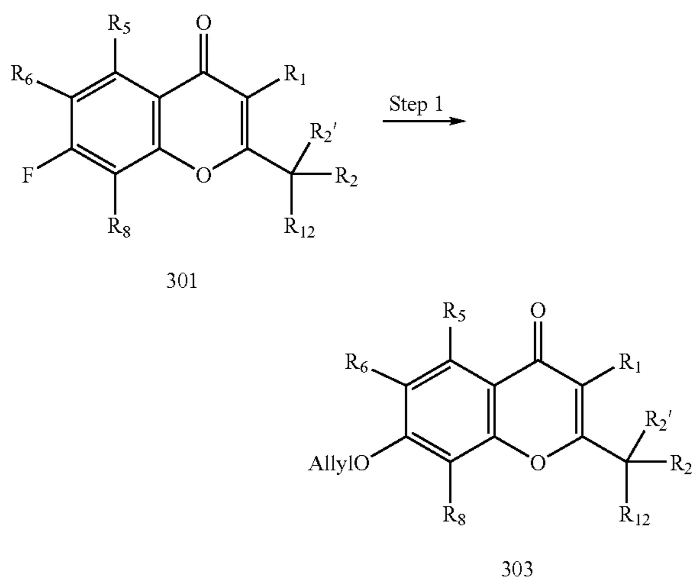
Reaction Scheme 3
