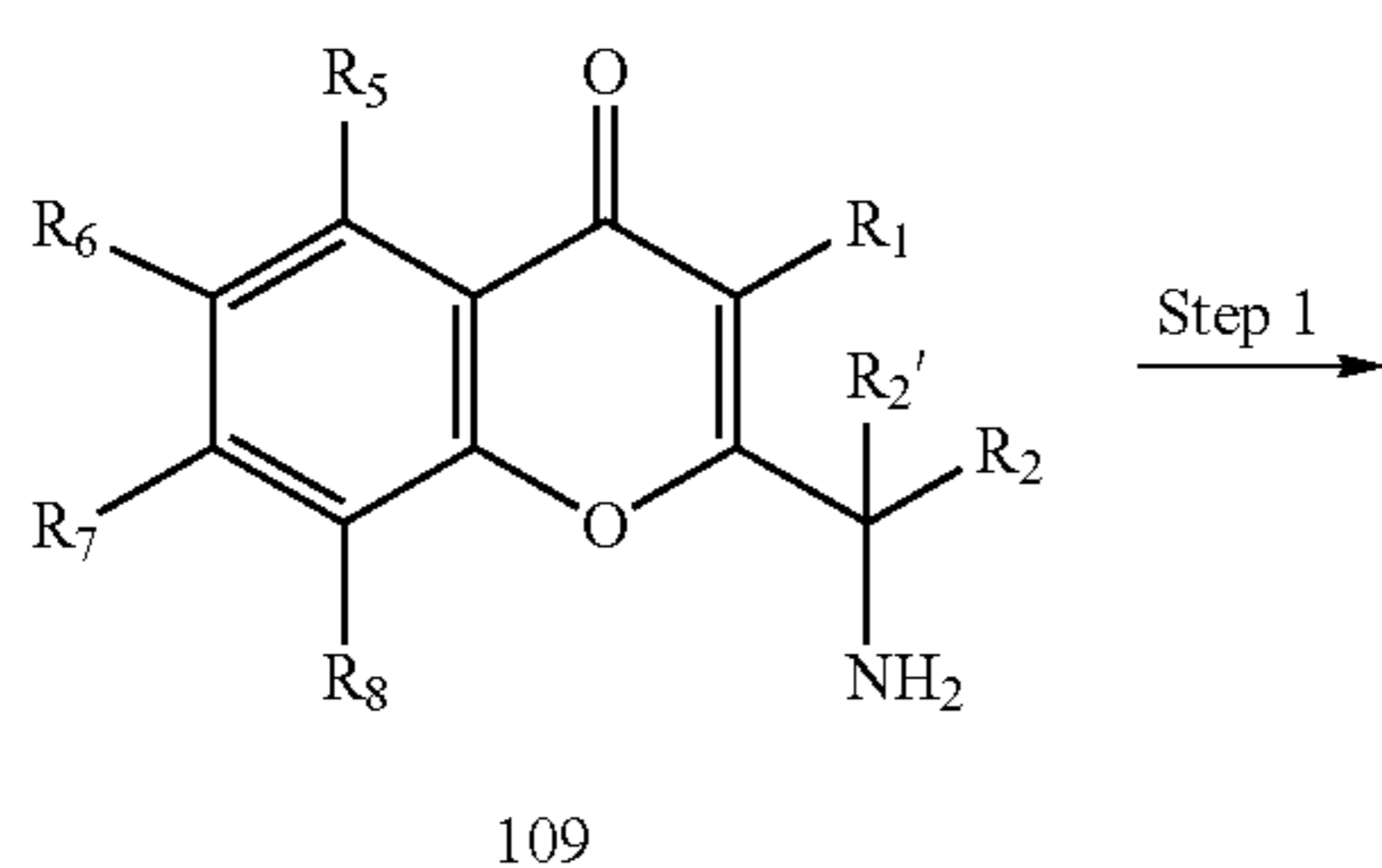
Reaction Scheme 8
