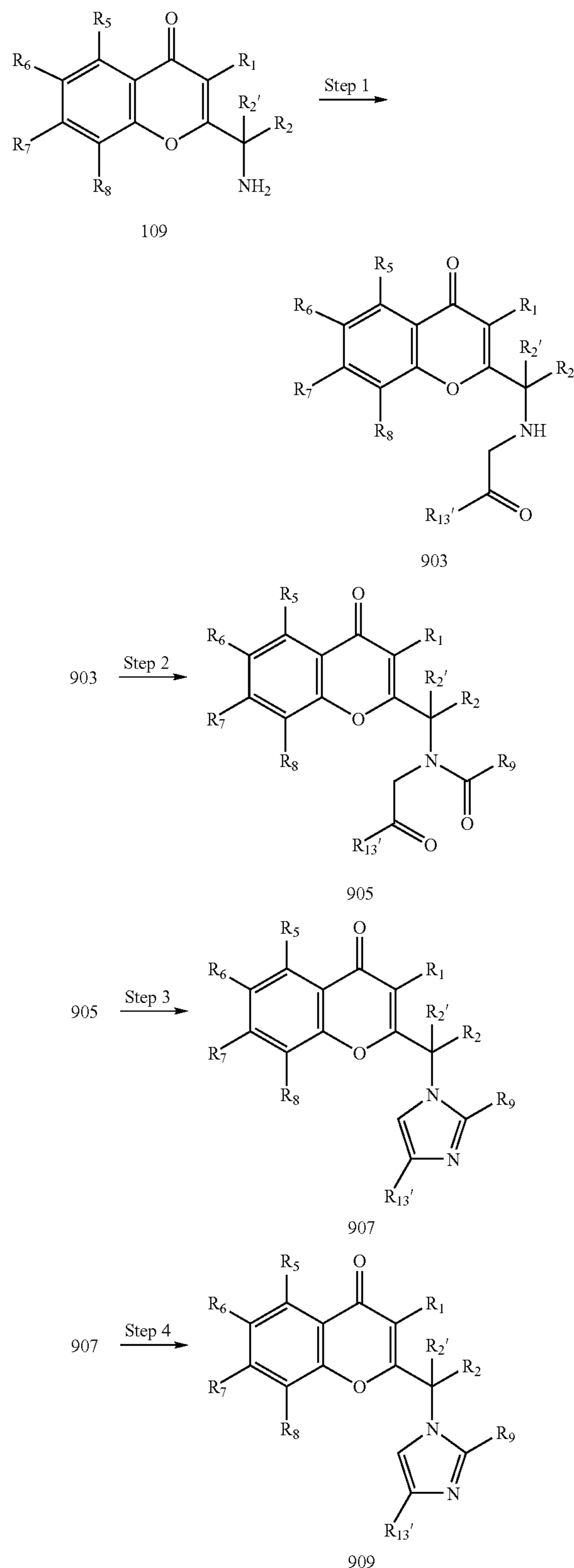
Reaction Scheme 9
