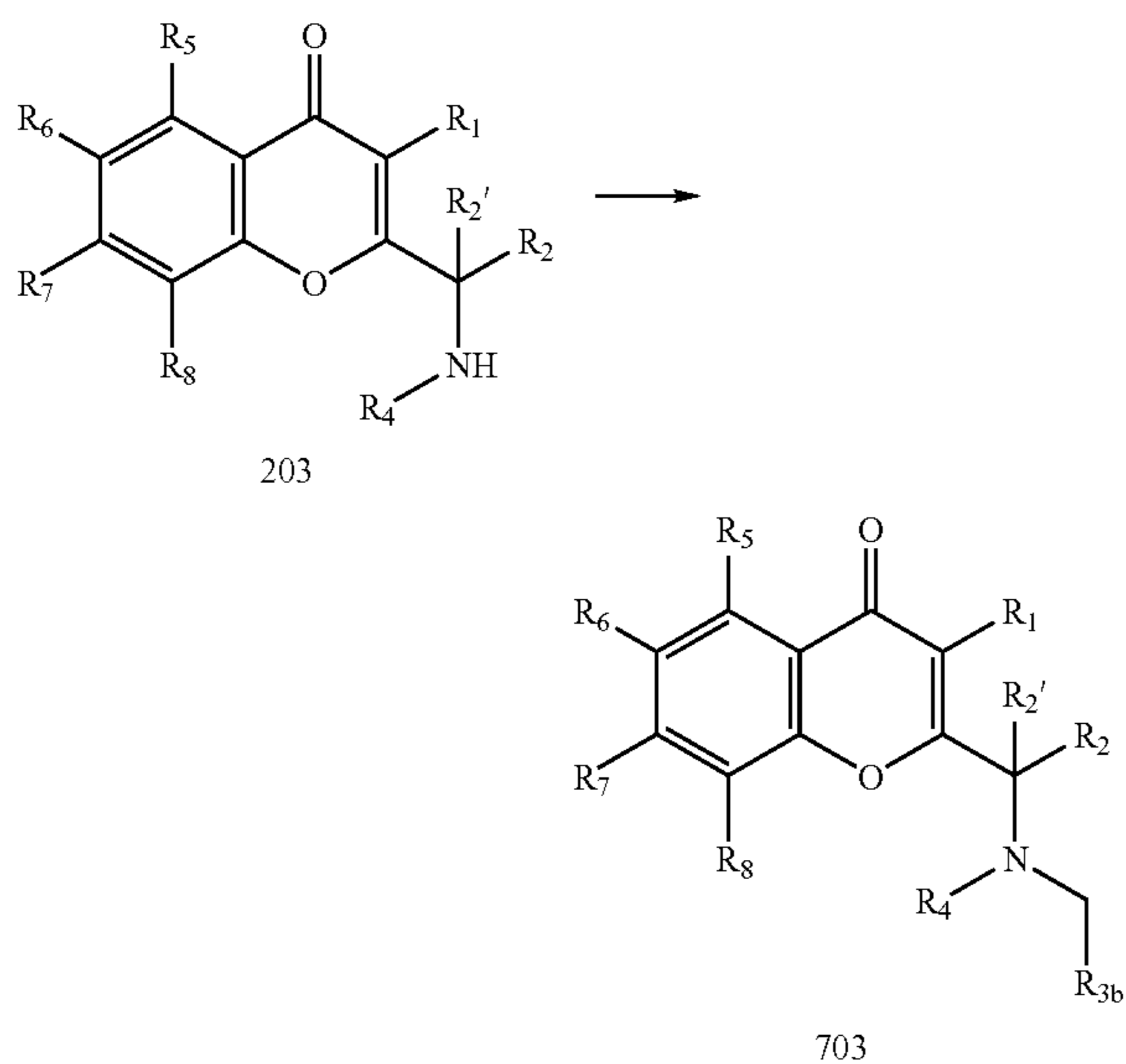
Reaction Scheme 7
