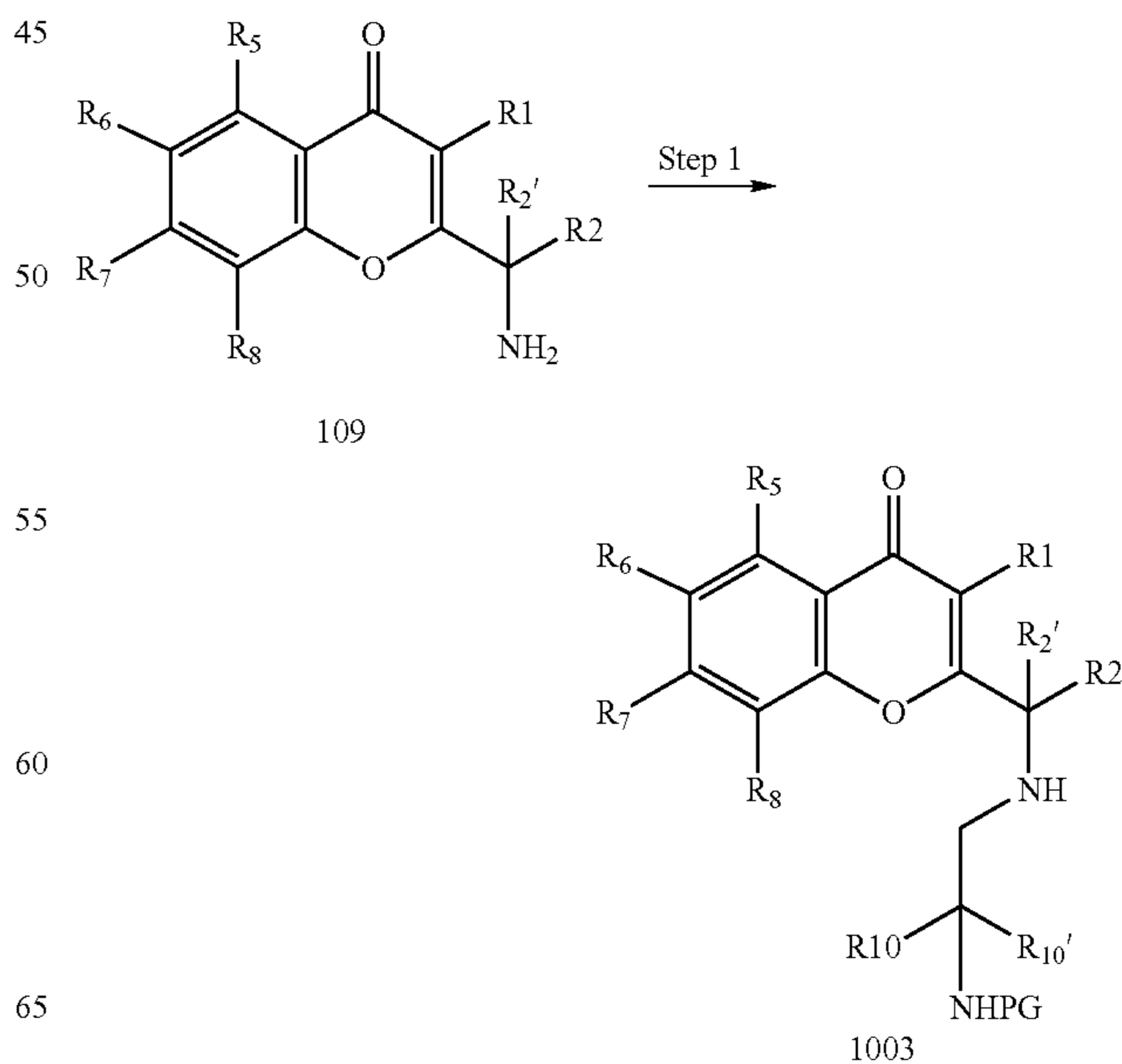
Reaction Scheme 10
