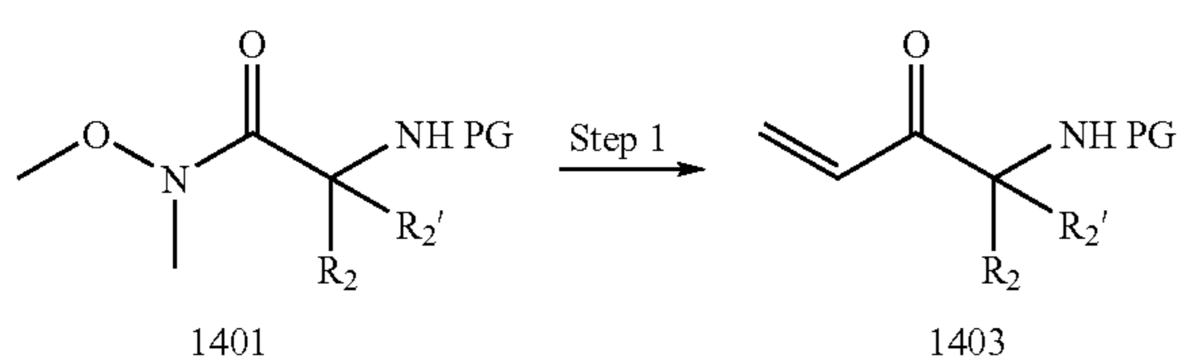
Reaction Scheme 14
