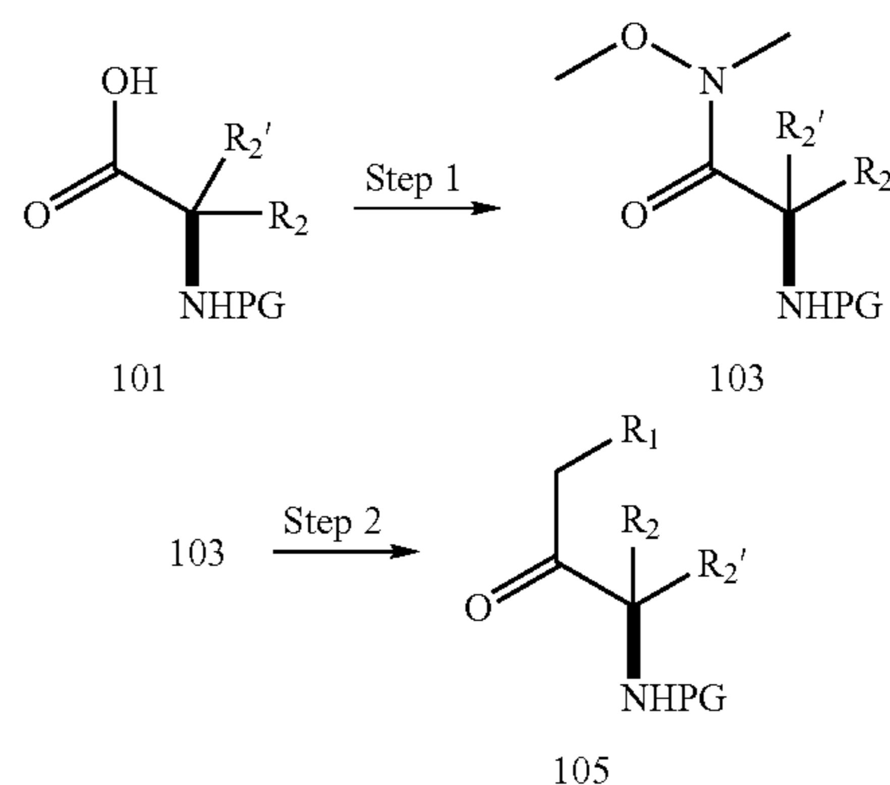
Reaction Scheme 1
