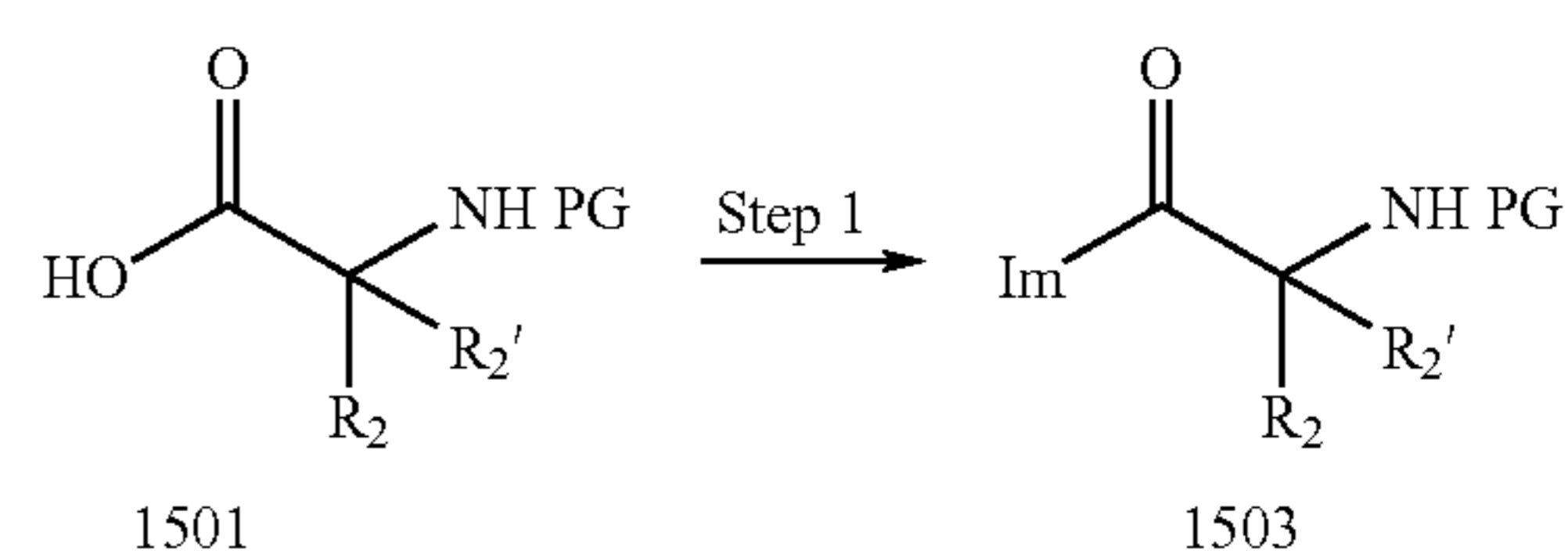
Reaction Scheme 15
