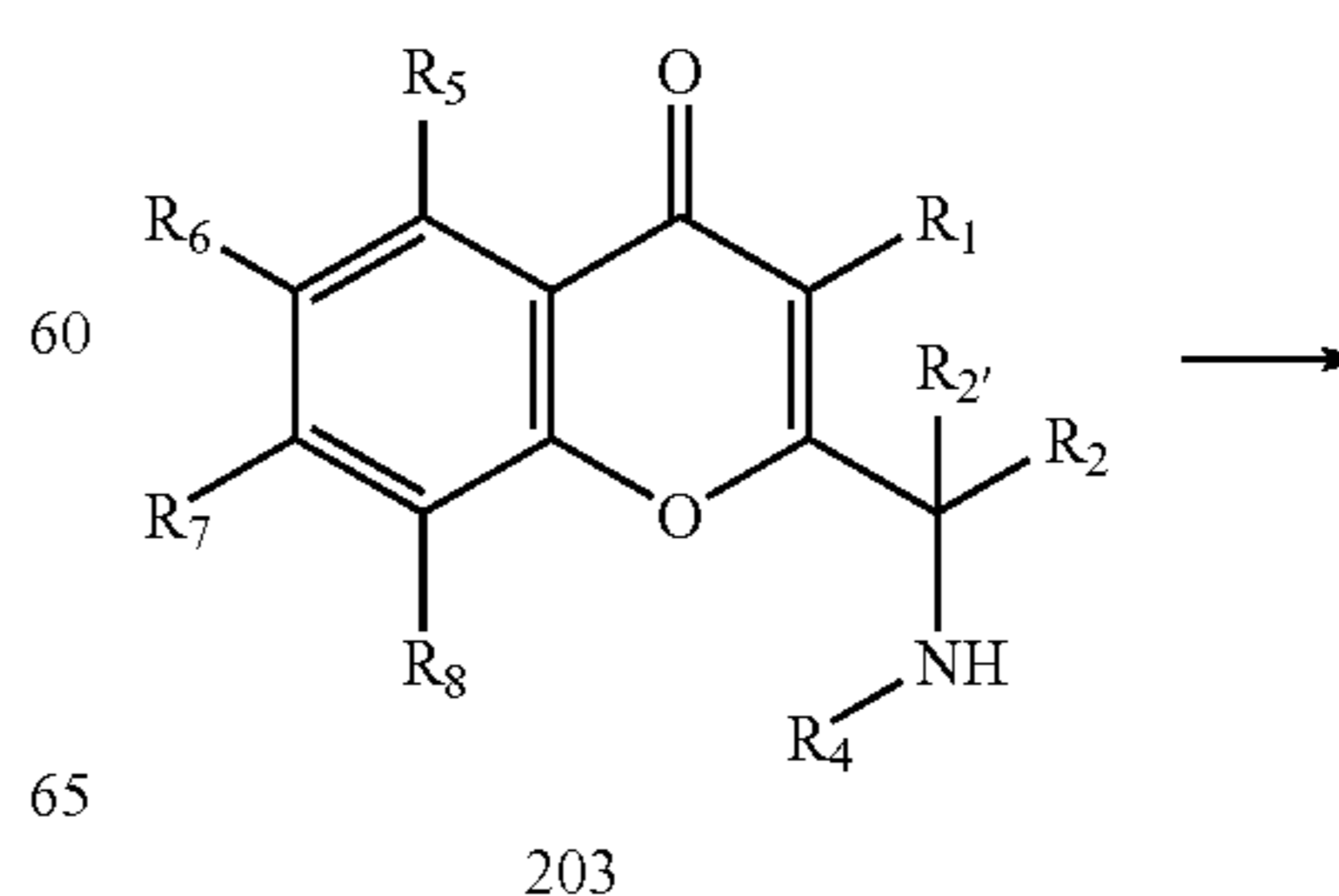
Reaction Scheme 6
