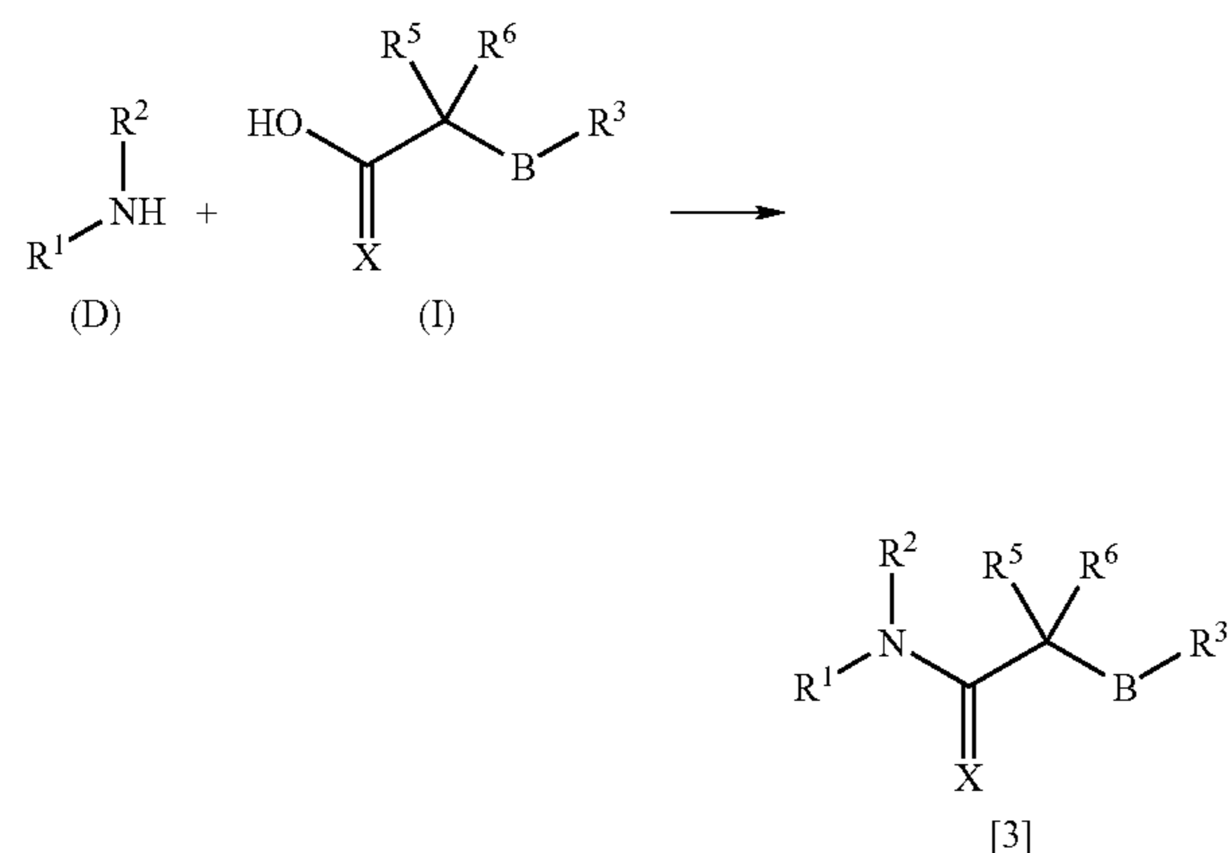
Reaction route 2
