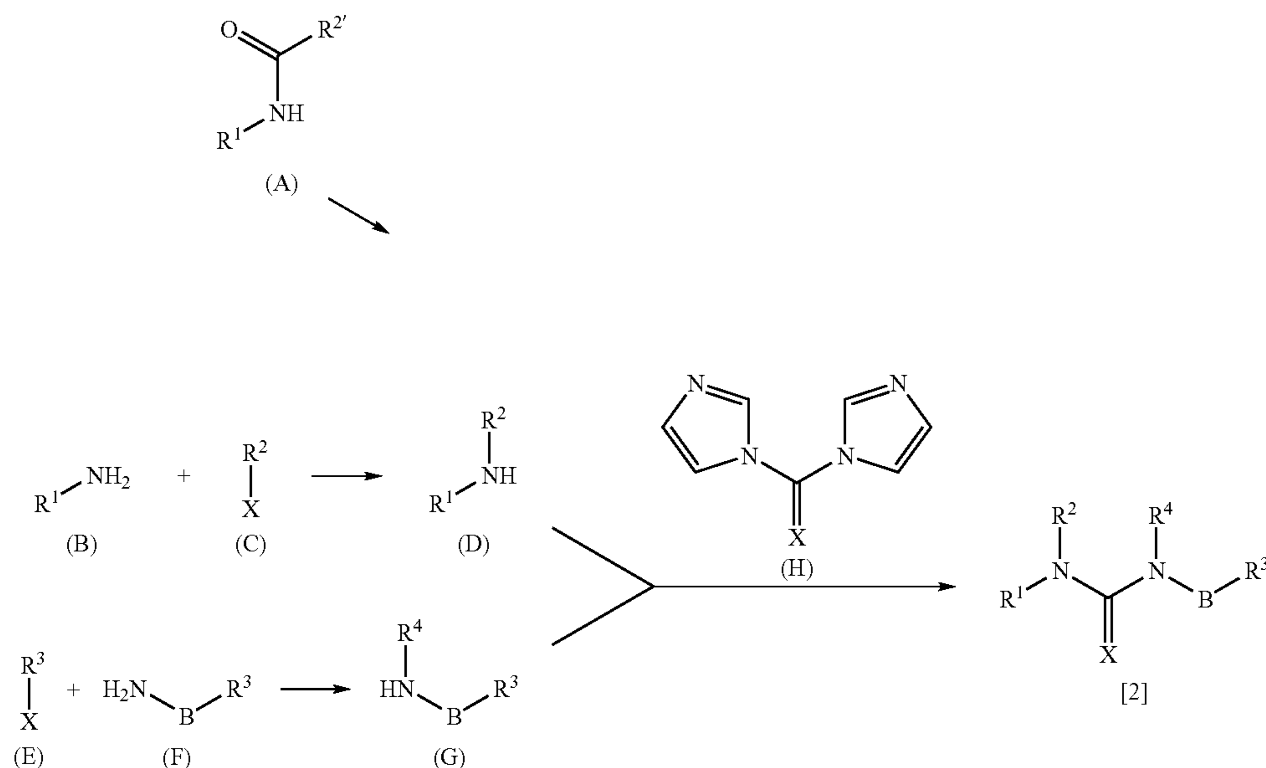
Reaction route 1
