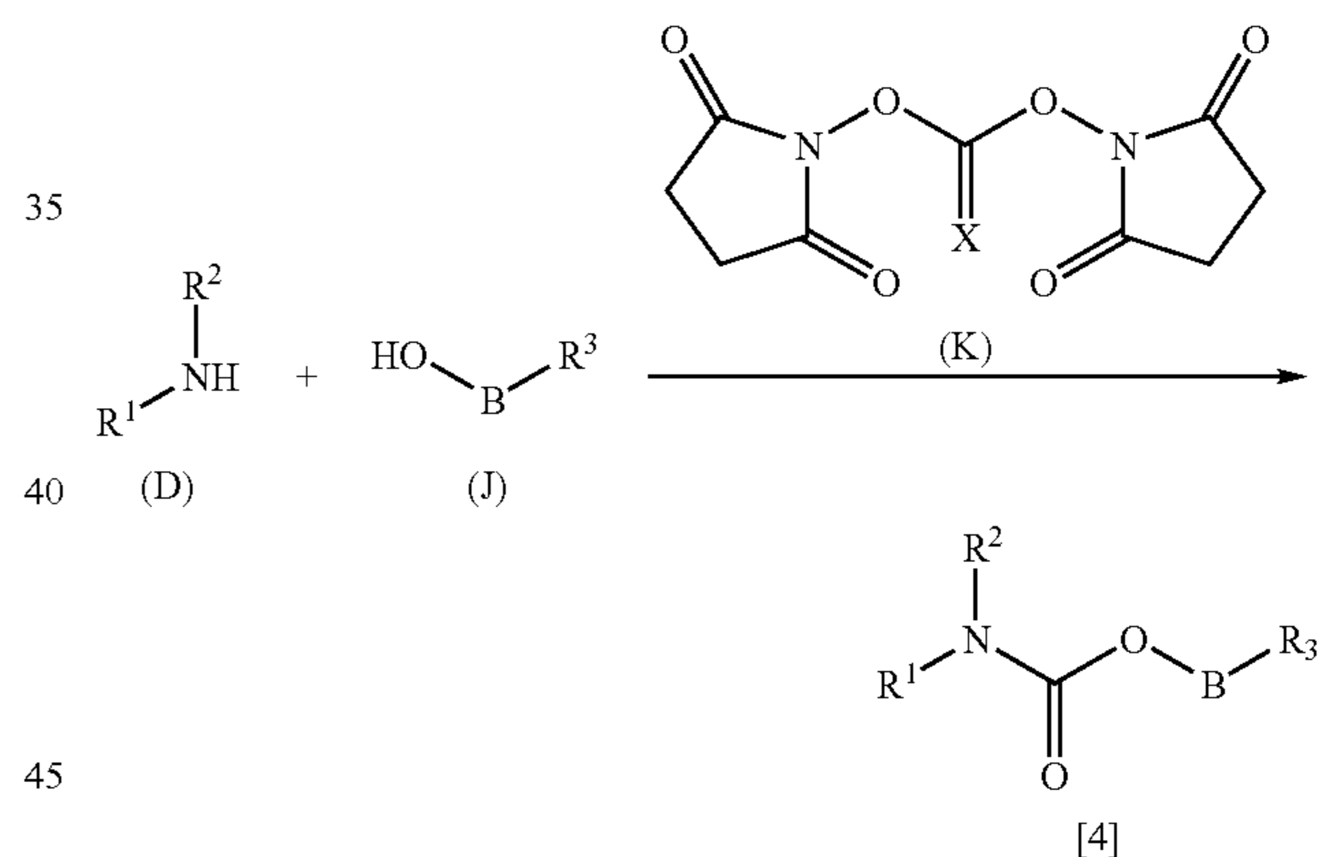
Reaction route 3
