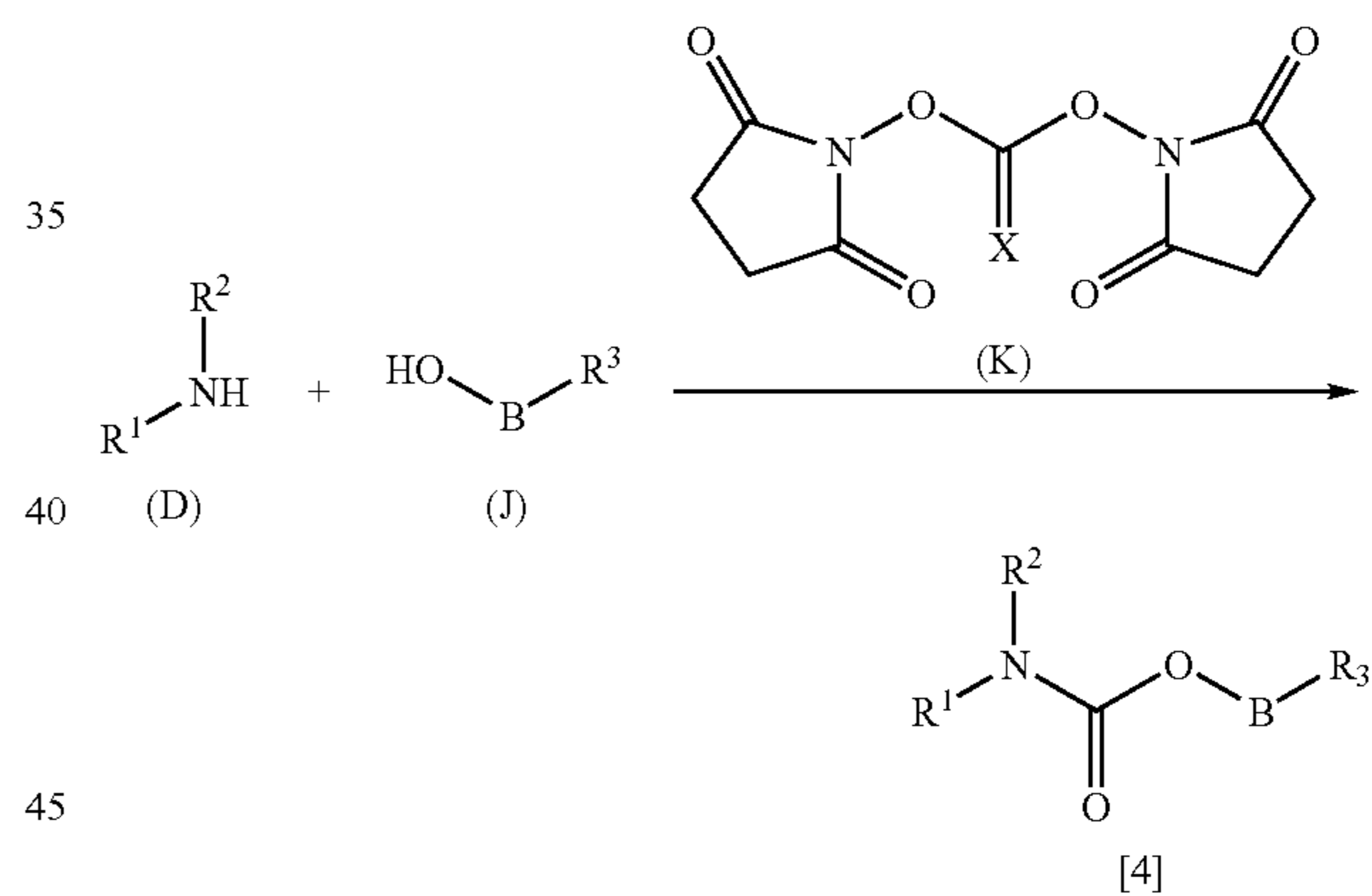
Reaction route 3
