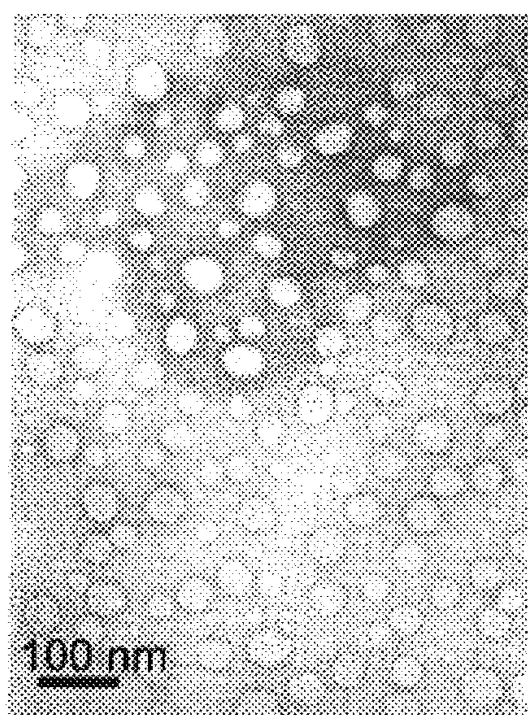
Phg-Phg+1M NaOH
