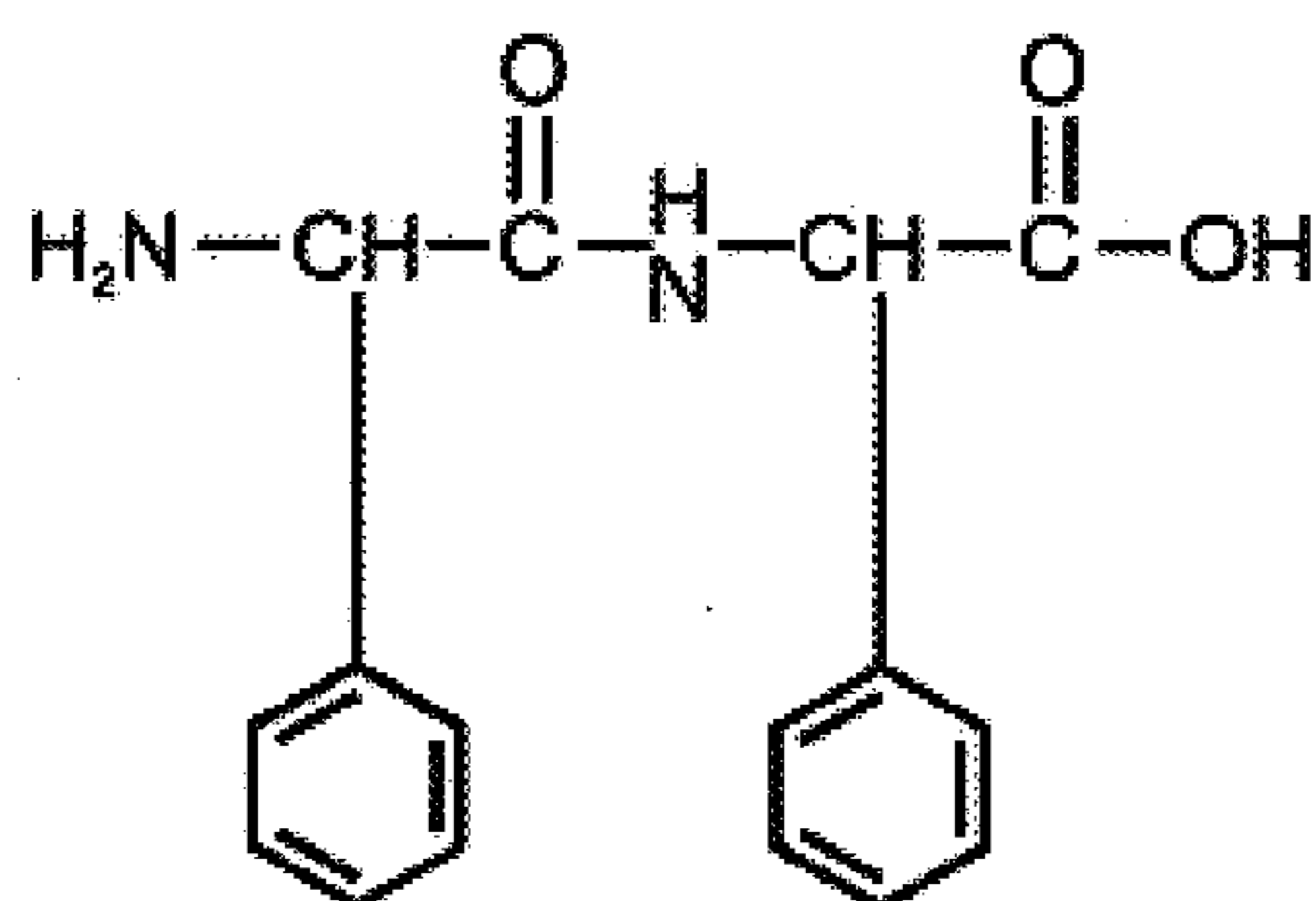
NH 2 -Phg-Phg-COOH
