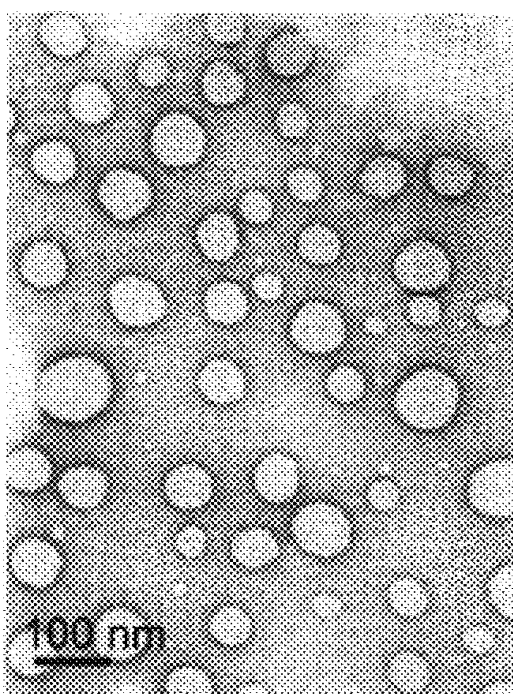
Phg-Phg+10%TFA
