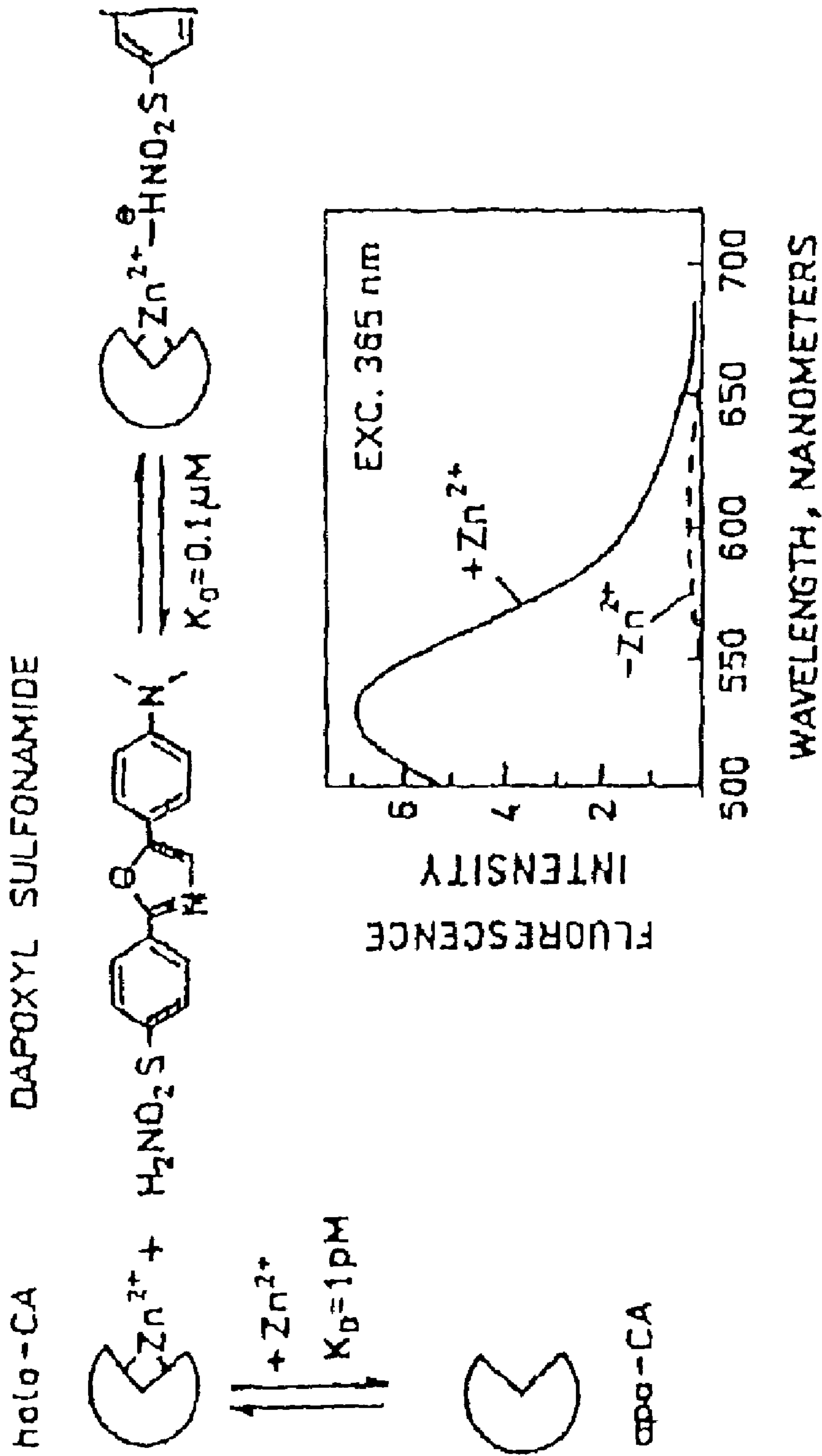
Fig. 1 Schematic of Zn(II) determination by fluorescence using apocarbonic anhydrase and Dapoxyl sulfonamide.
