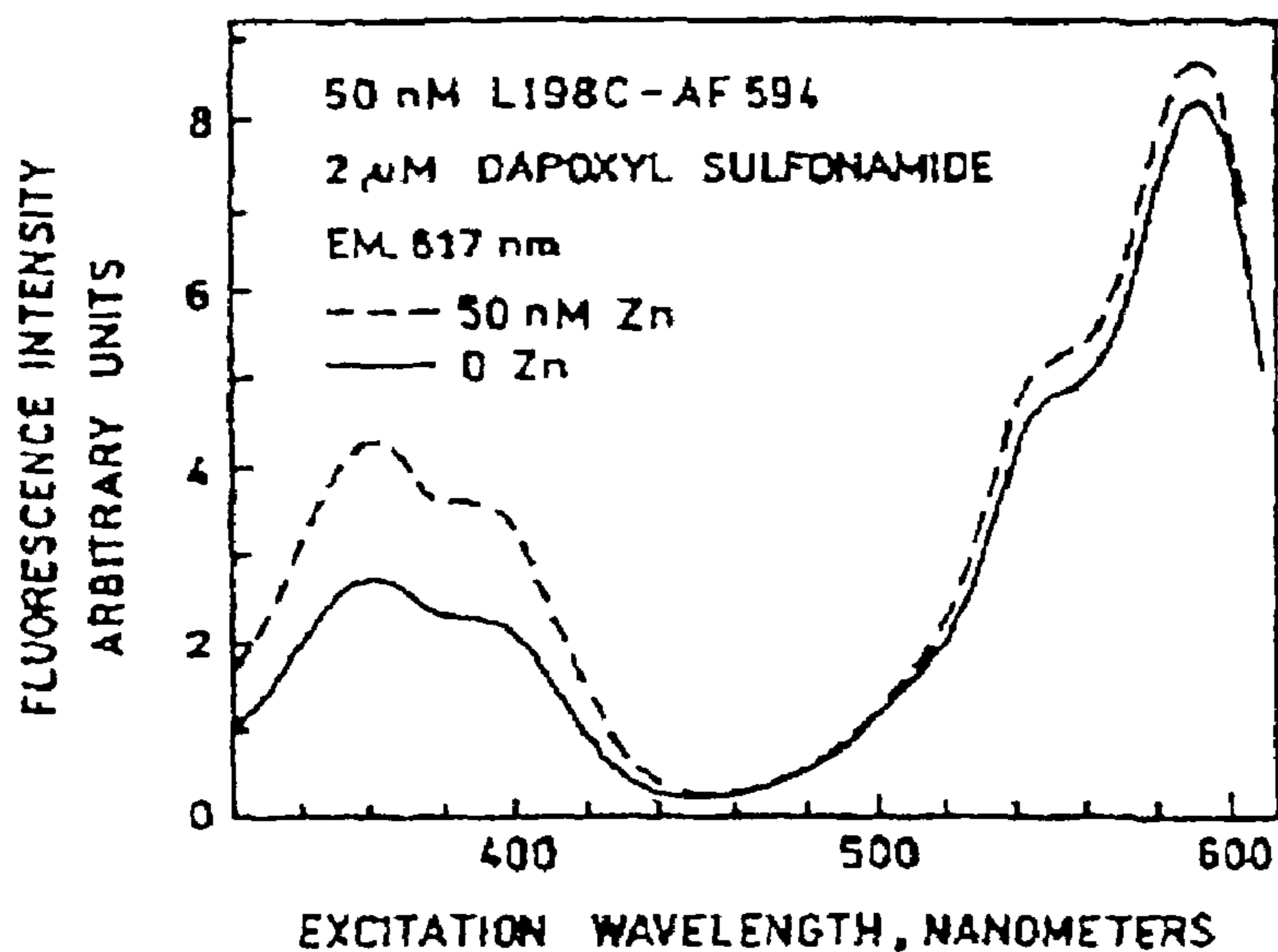
Fig. 5 Excitation spectra of 50 nM apoL198C-Alexa Fluor 594 and 2 μM Dapoxyl sulfonamide in the absence (—) and presence of 50 nM free Zn(II) (---); emission at 617 nm.
