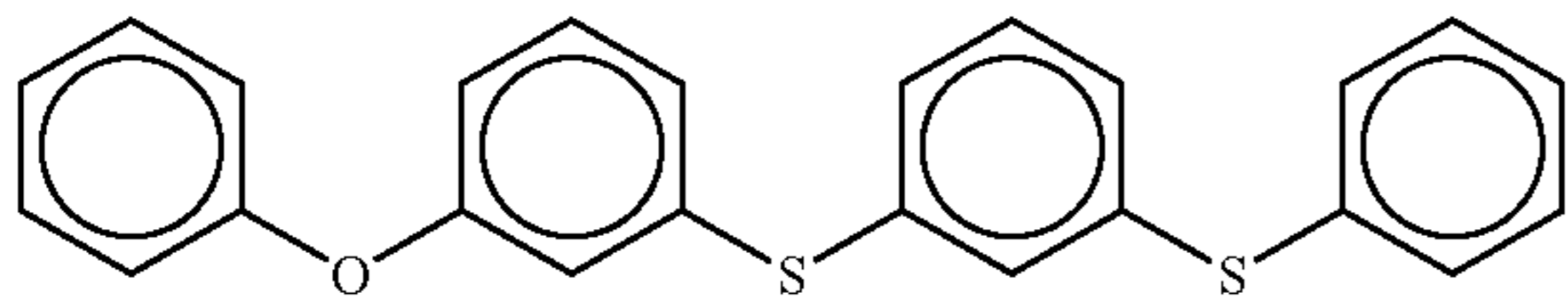
1-phenoxy-3-[[3-(phenylthio)phenyl]thio]benzene
