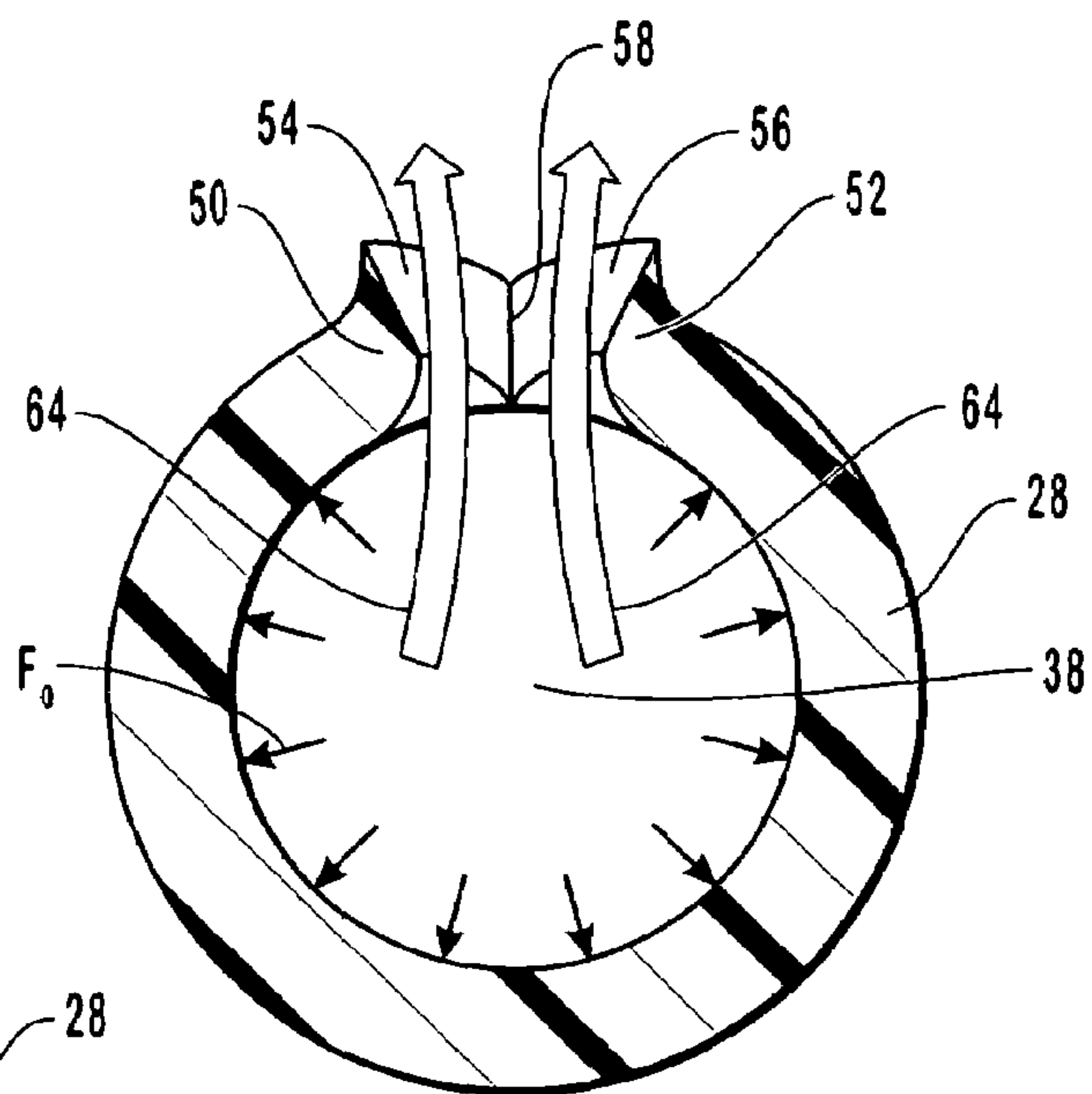
FIG. 5 (PRIOR ART)
