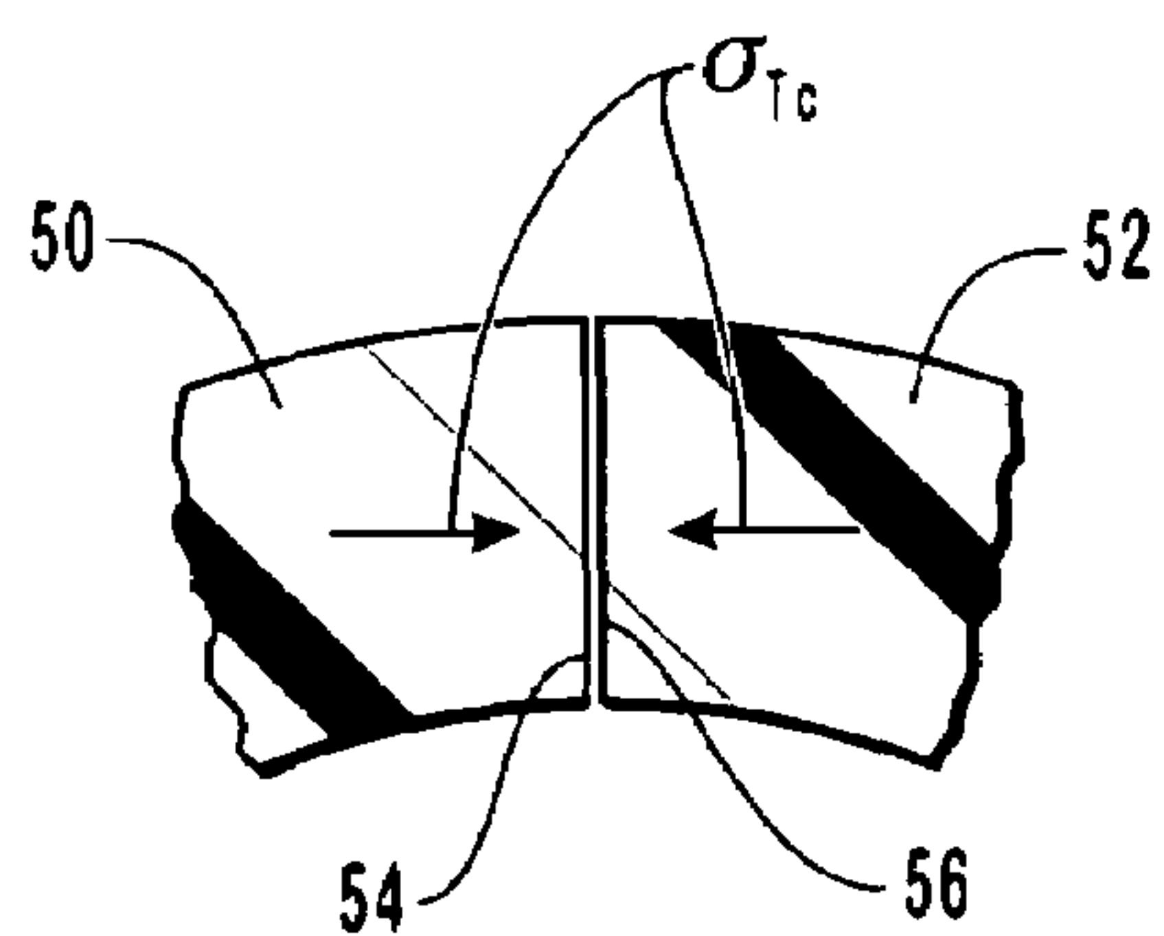
FIG. 7 (PRIOR ART)
