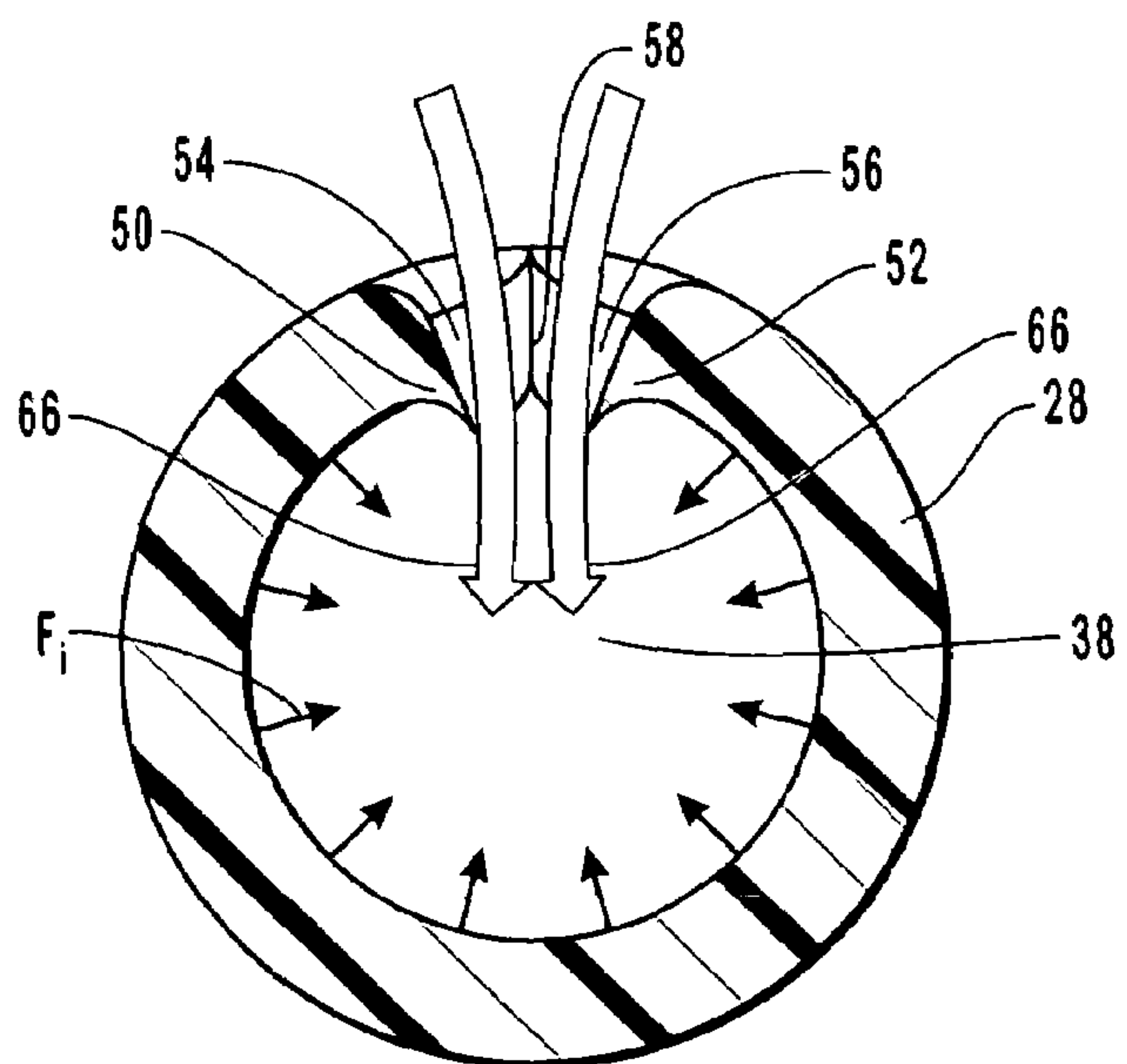
FIG. 8 (PRIOR ART)
