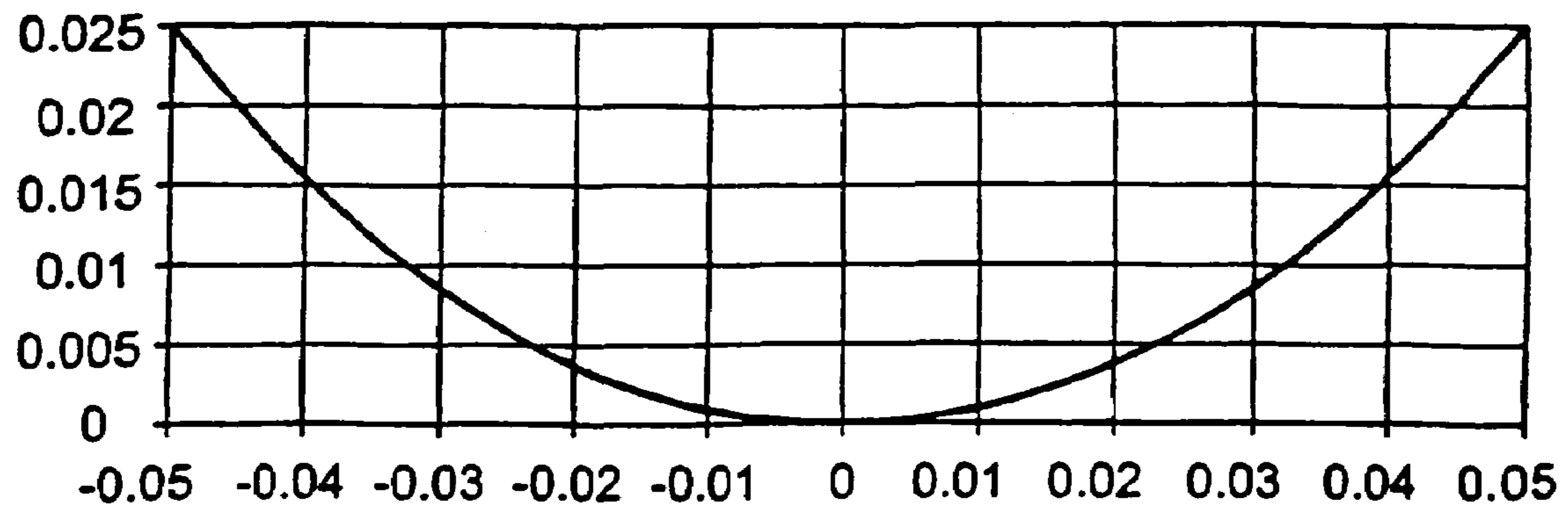
COSH Dimple Profile a=20, r=0.05, d=0.025, \nu r=0.51
