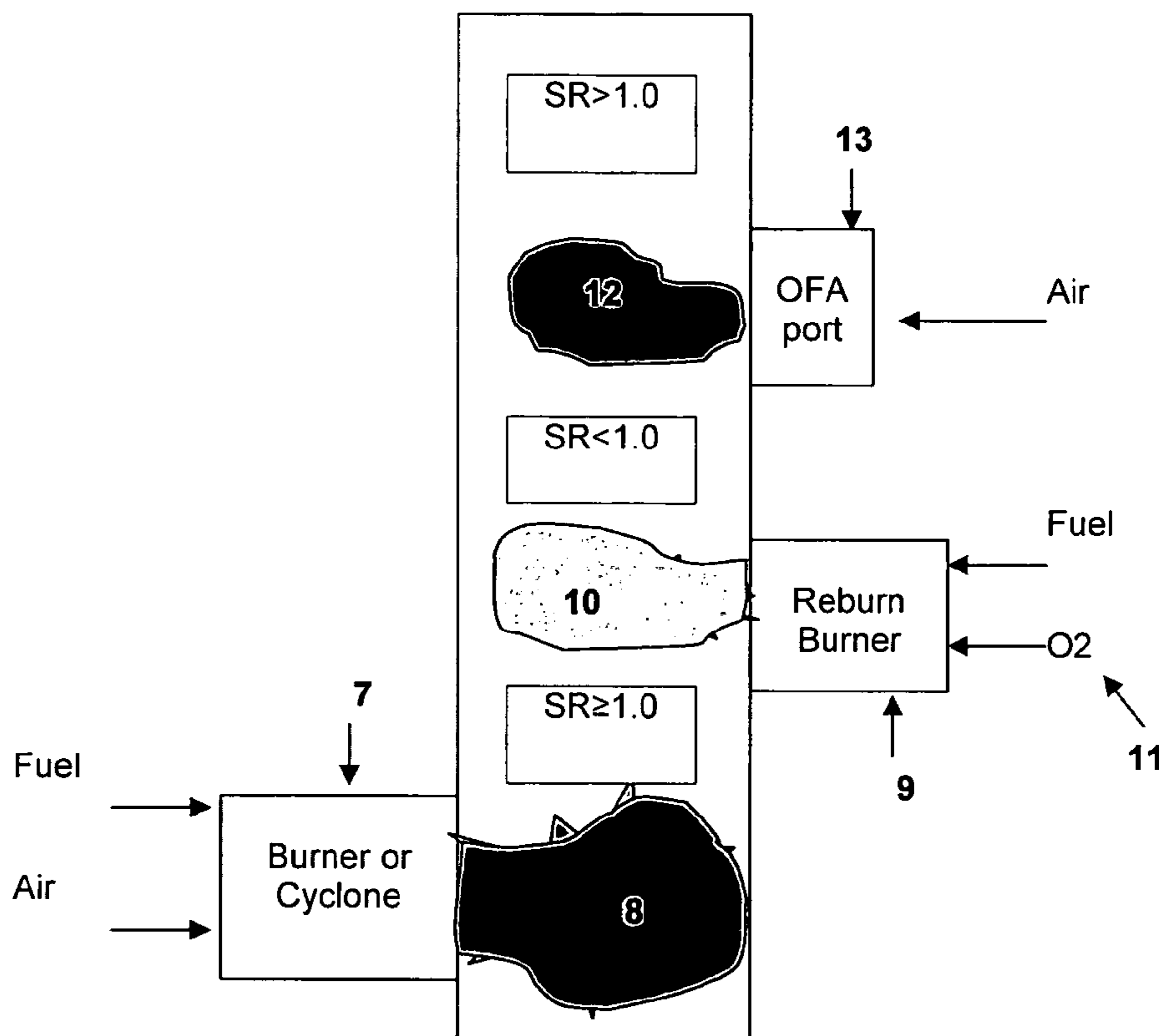
Oxy-fuel reburning
