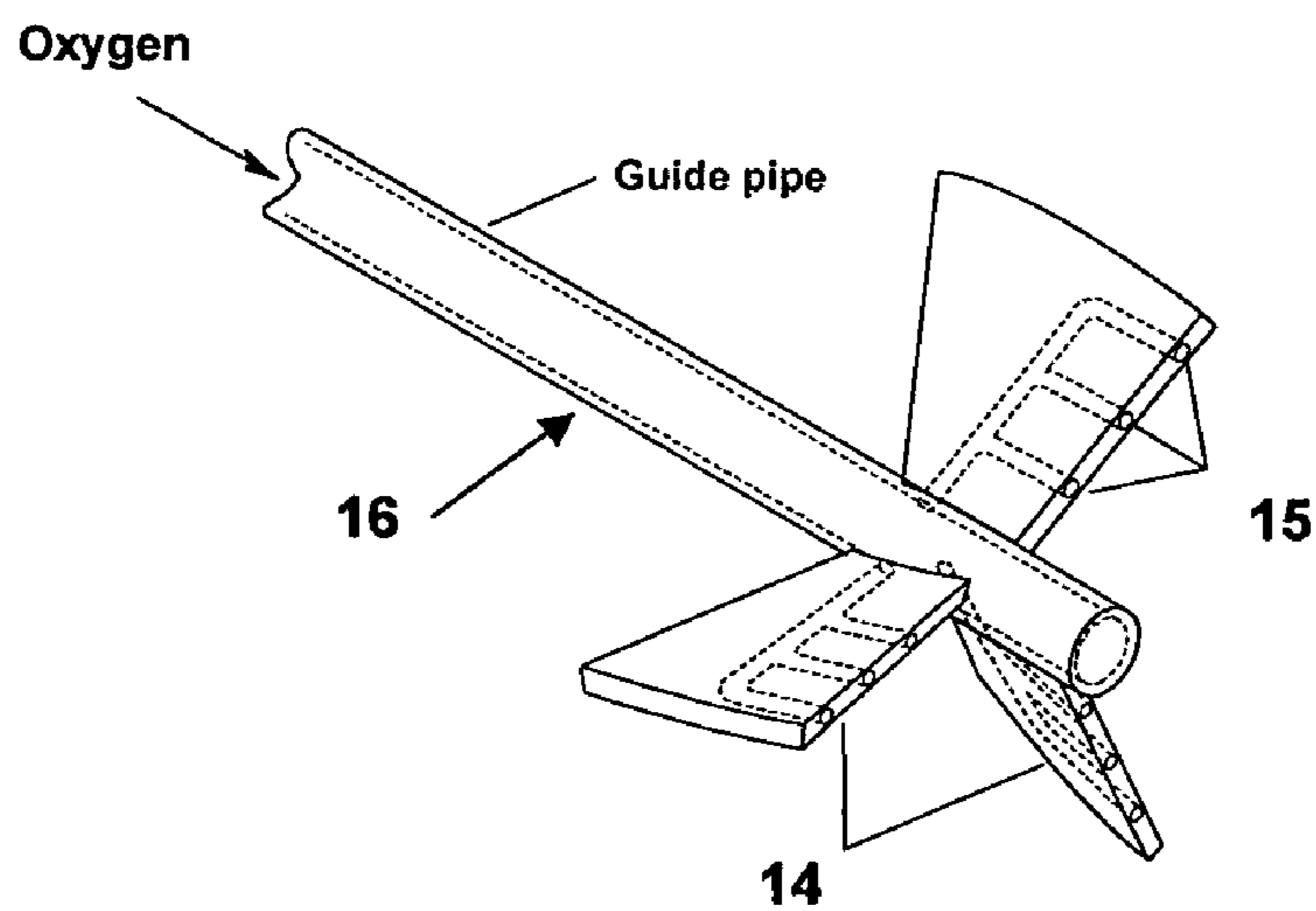
Fig. 3 Oxygen injection device
