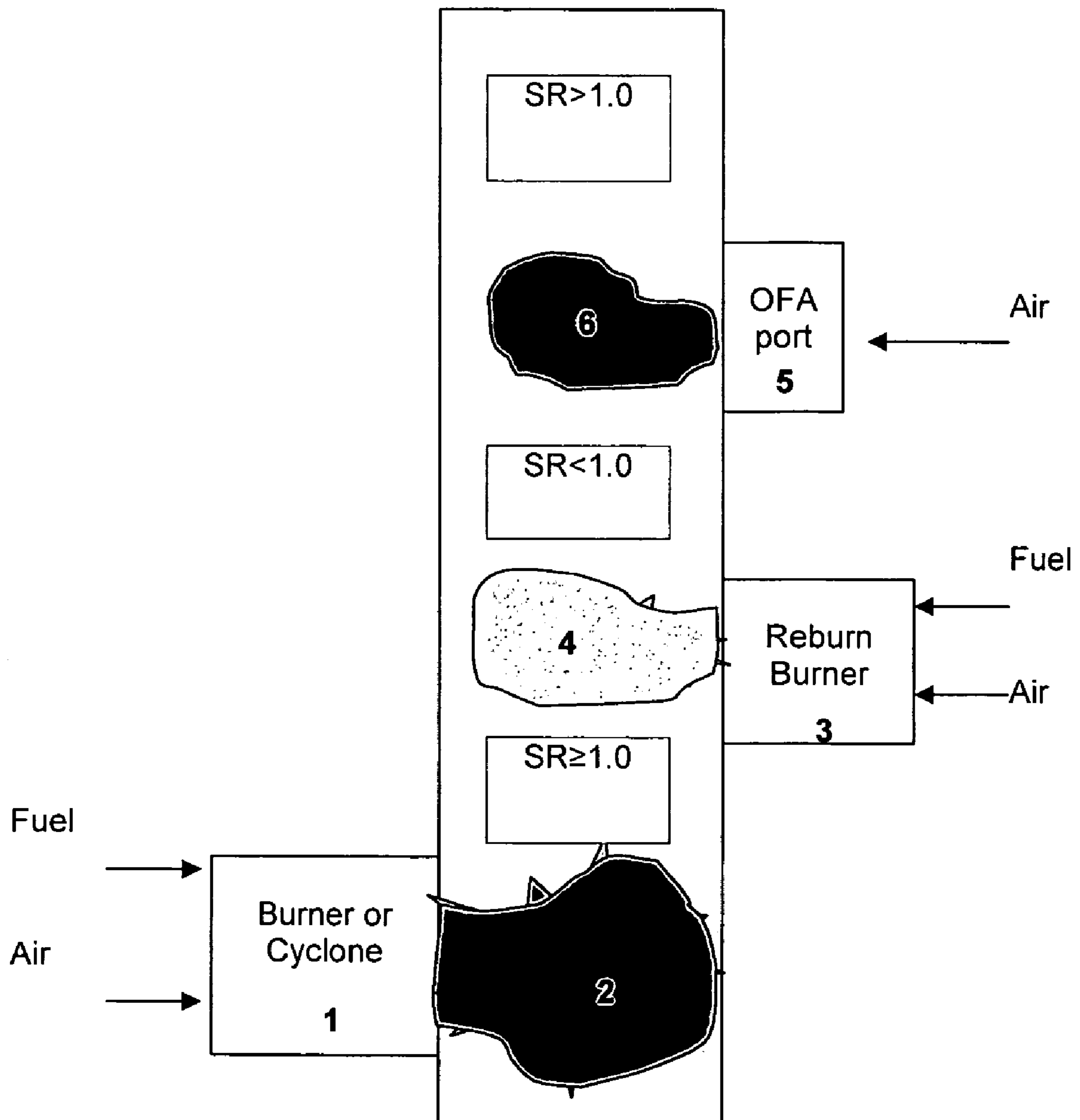
Fig. 1 Conventional reburning
