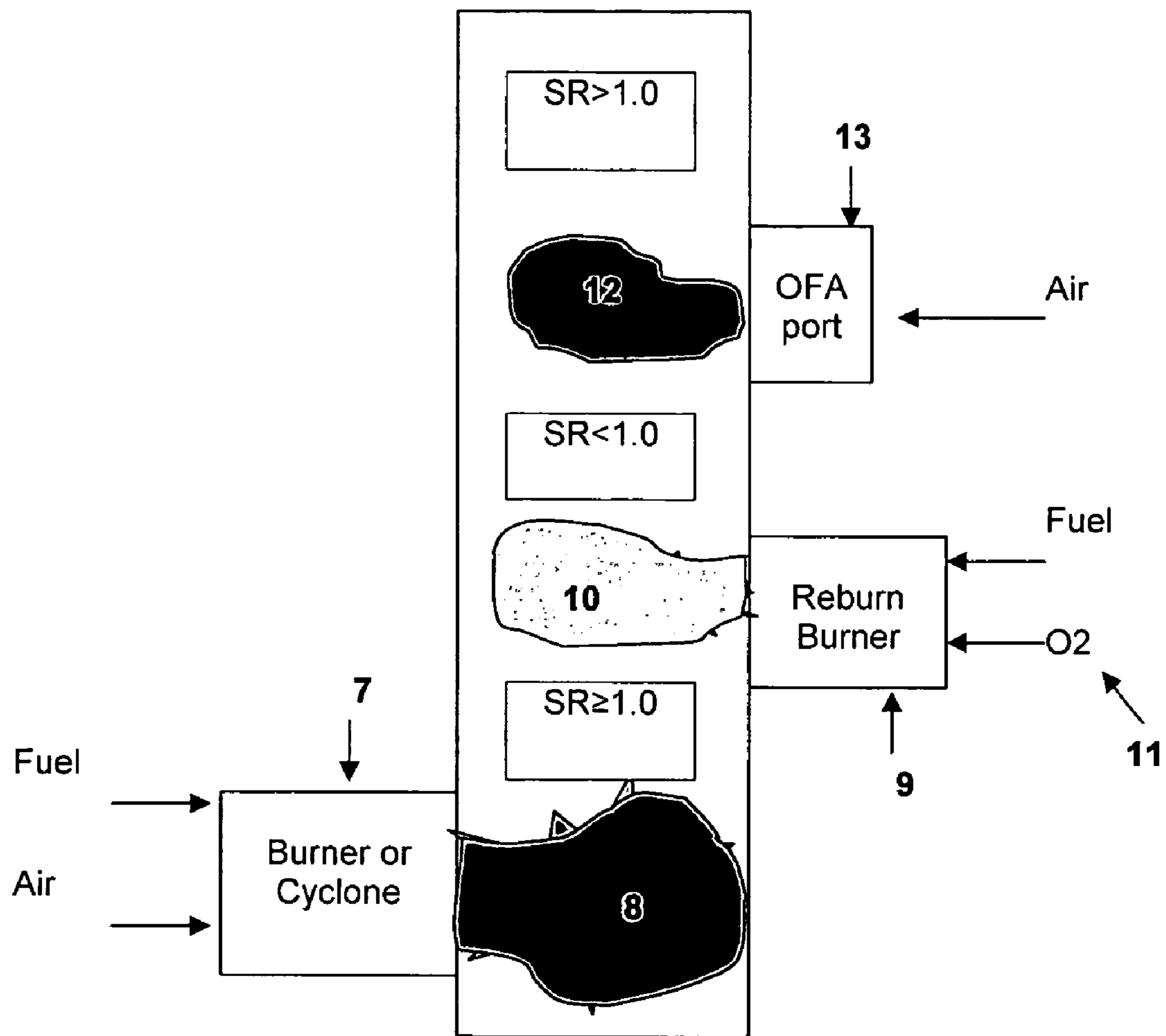
Fig. 2 Oxy-fuel reburning
