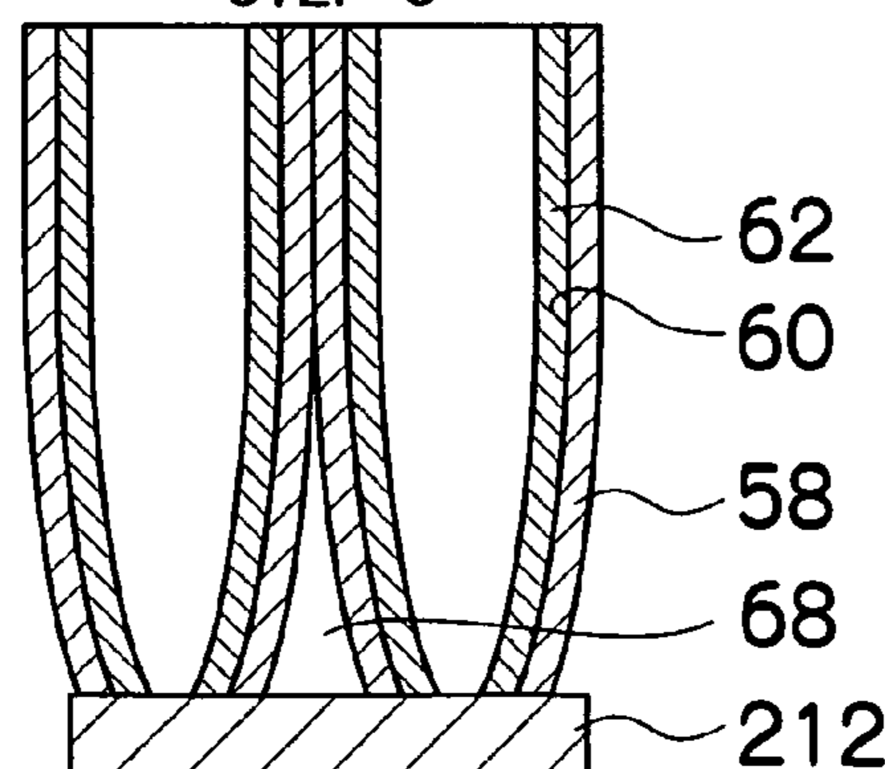
FIG.11C STEP 3
