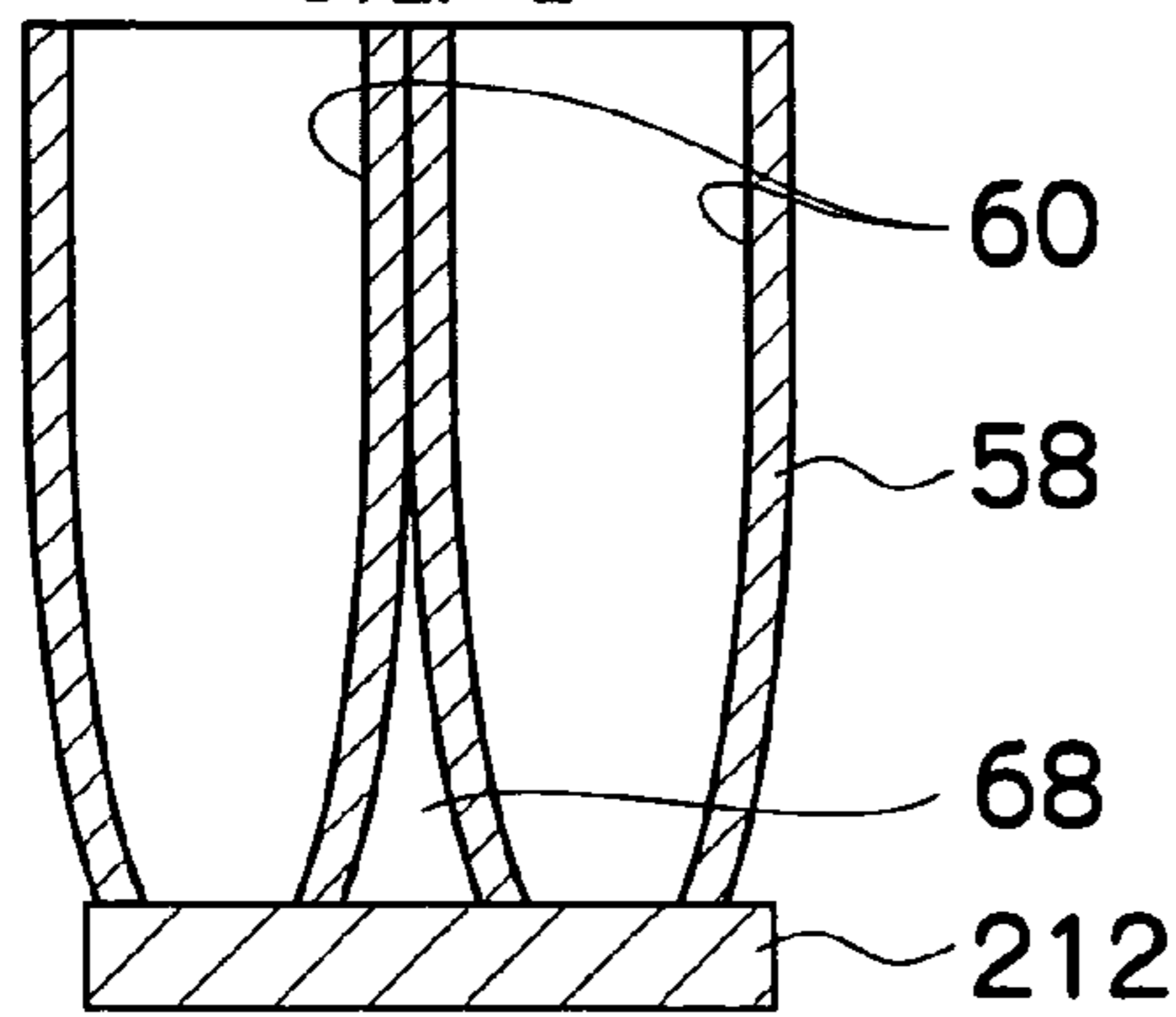
FIG.11B STEP 2
