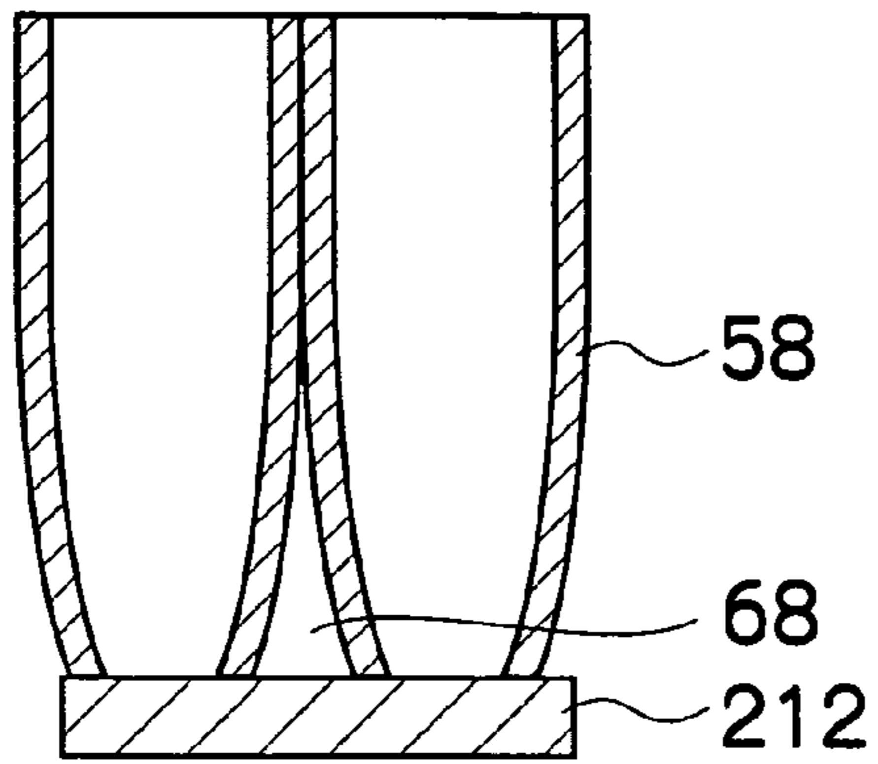
FIG.11A STEP 1
