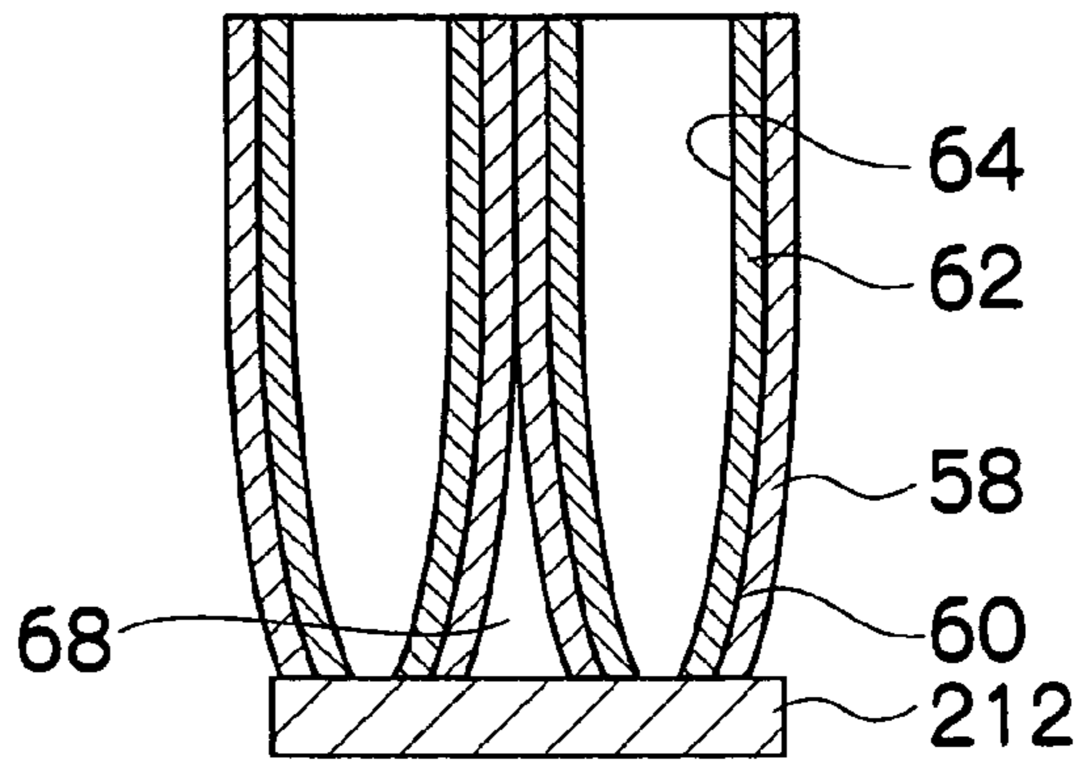
FIG.11D STEP 4
