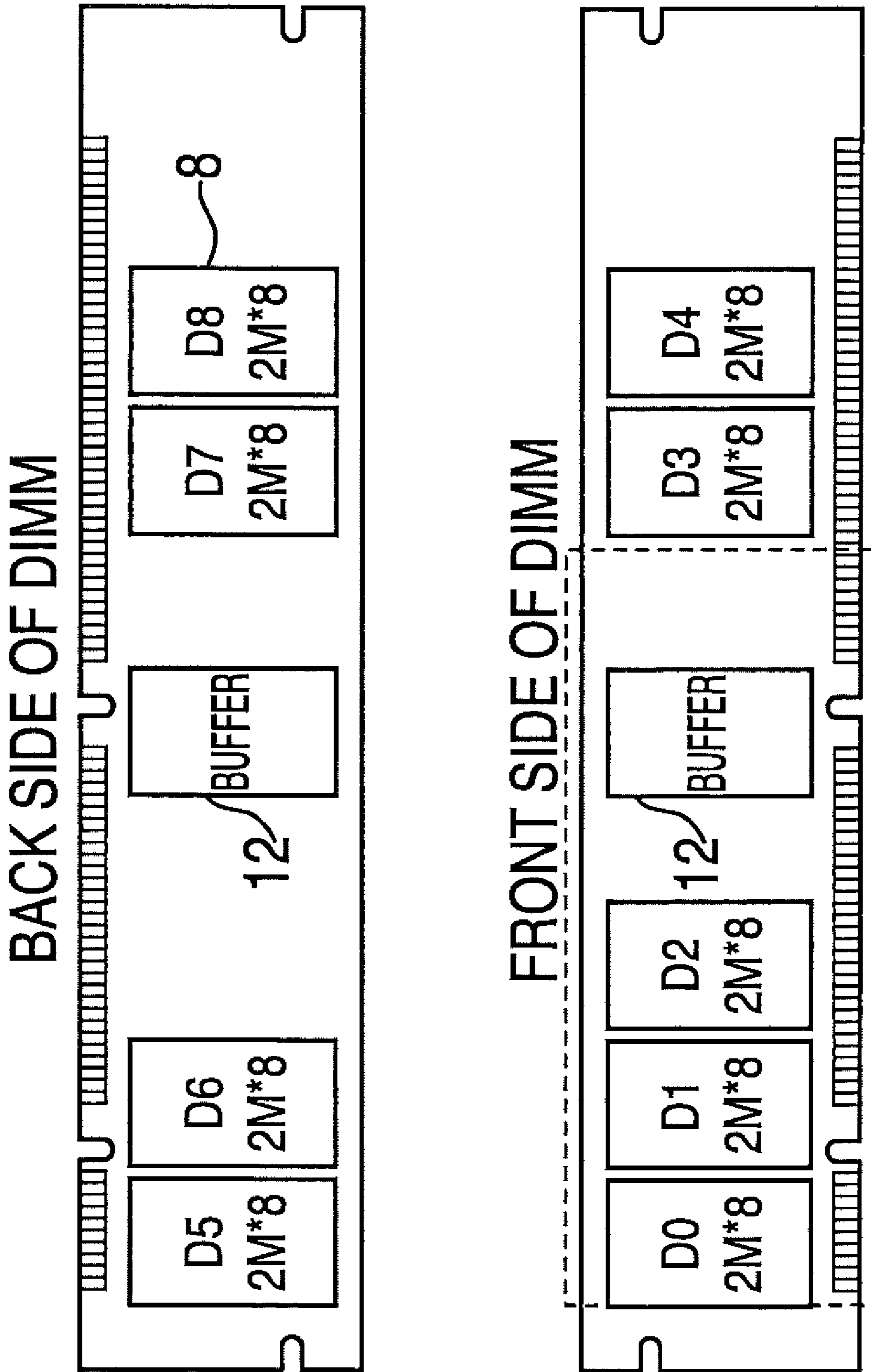
FIG. 1 (PRIOR ART)
