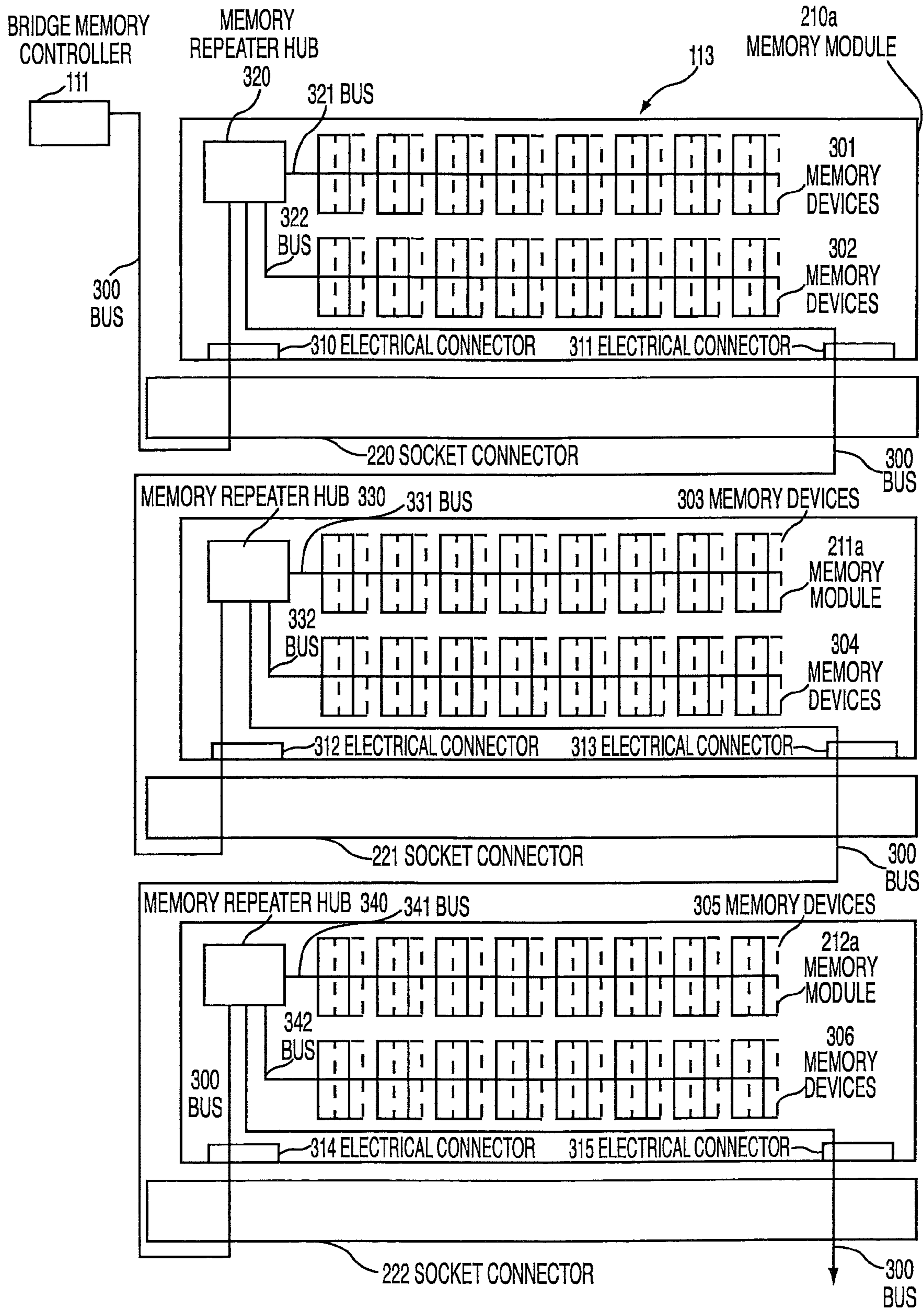
FIG. 4 (PRIOR ART)
