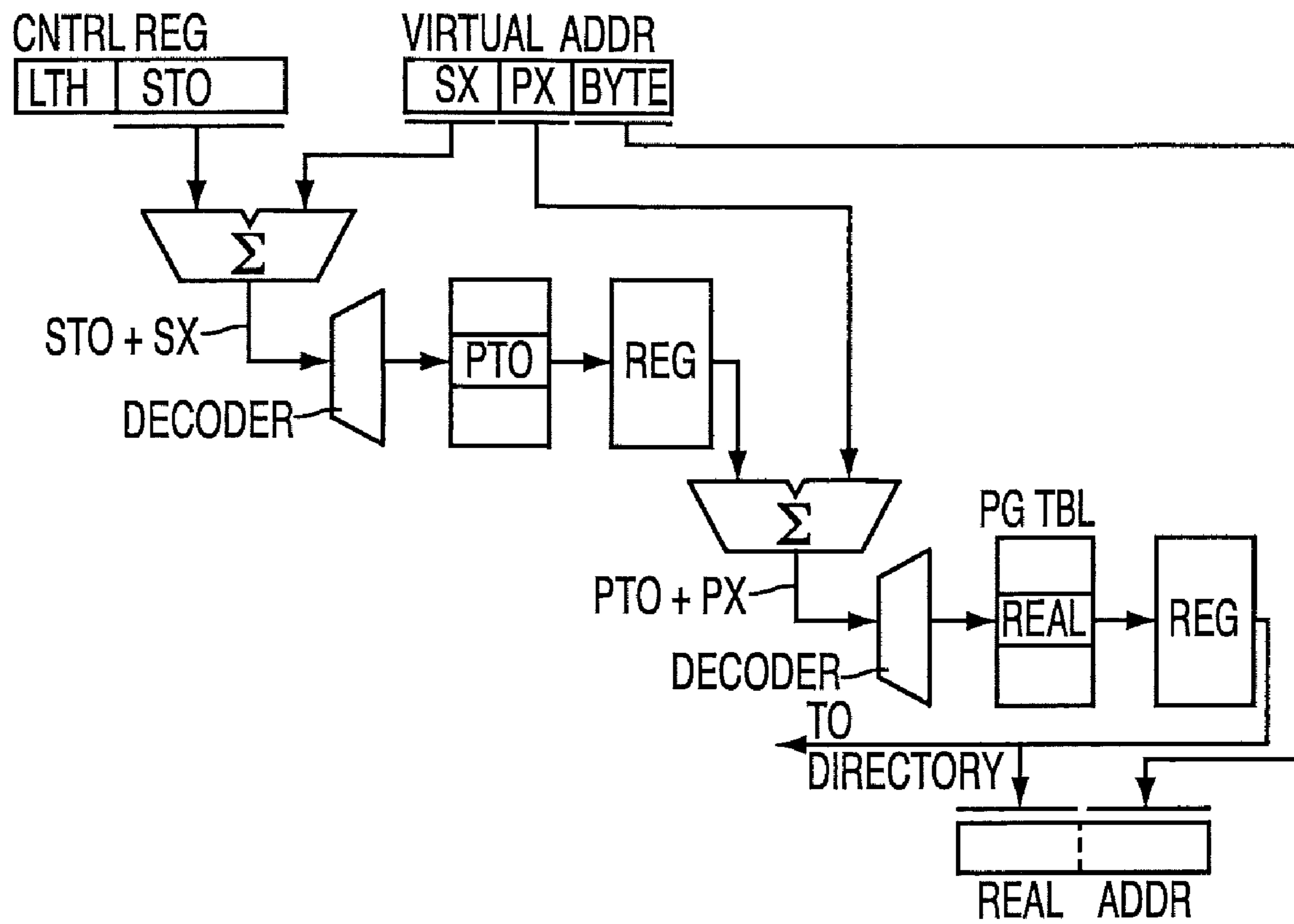
FIG. 5 (PRIOR ART)
