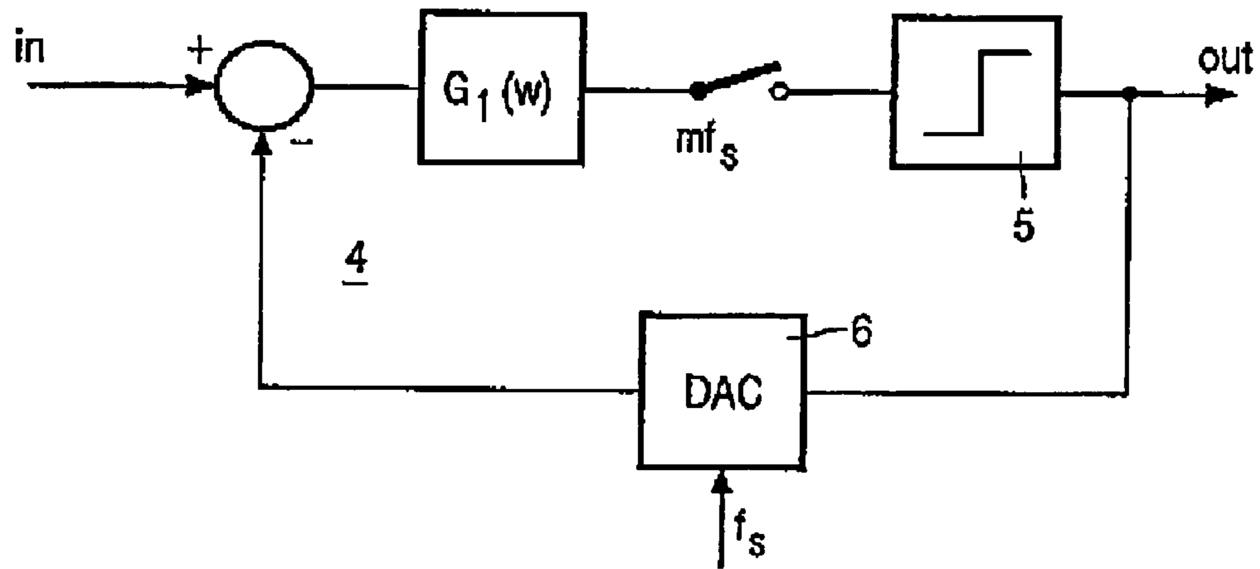
FIG. 2 (PRIOR ART)
