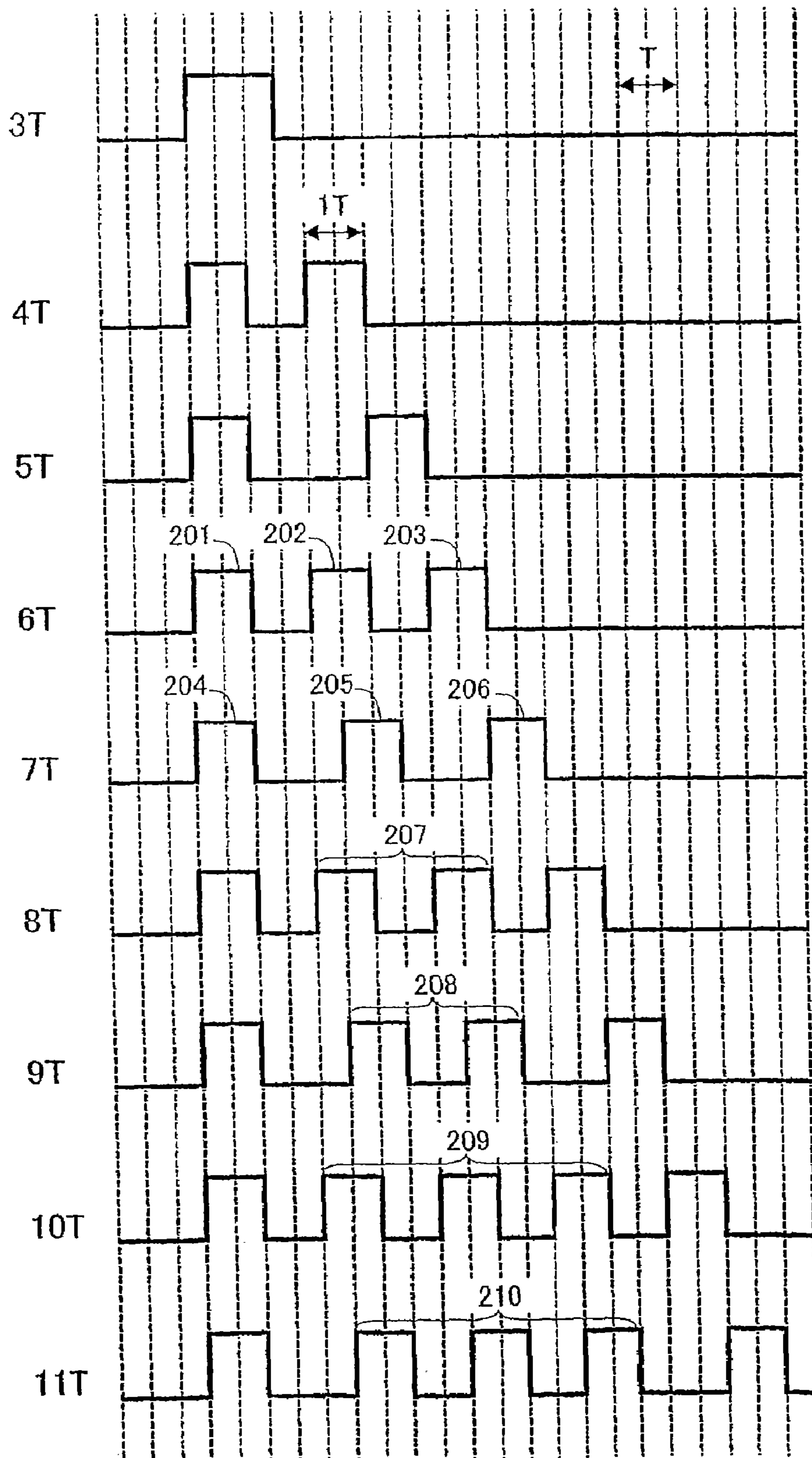
FIG. 6 (Prior Art)
