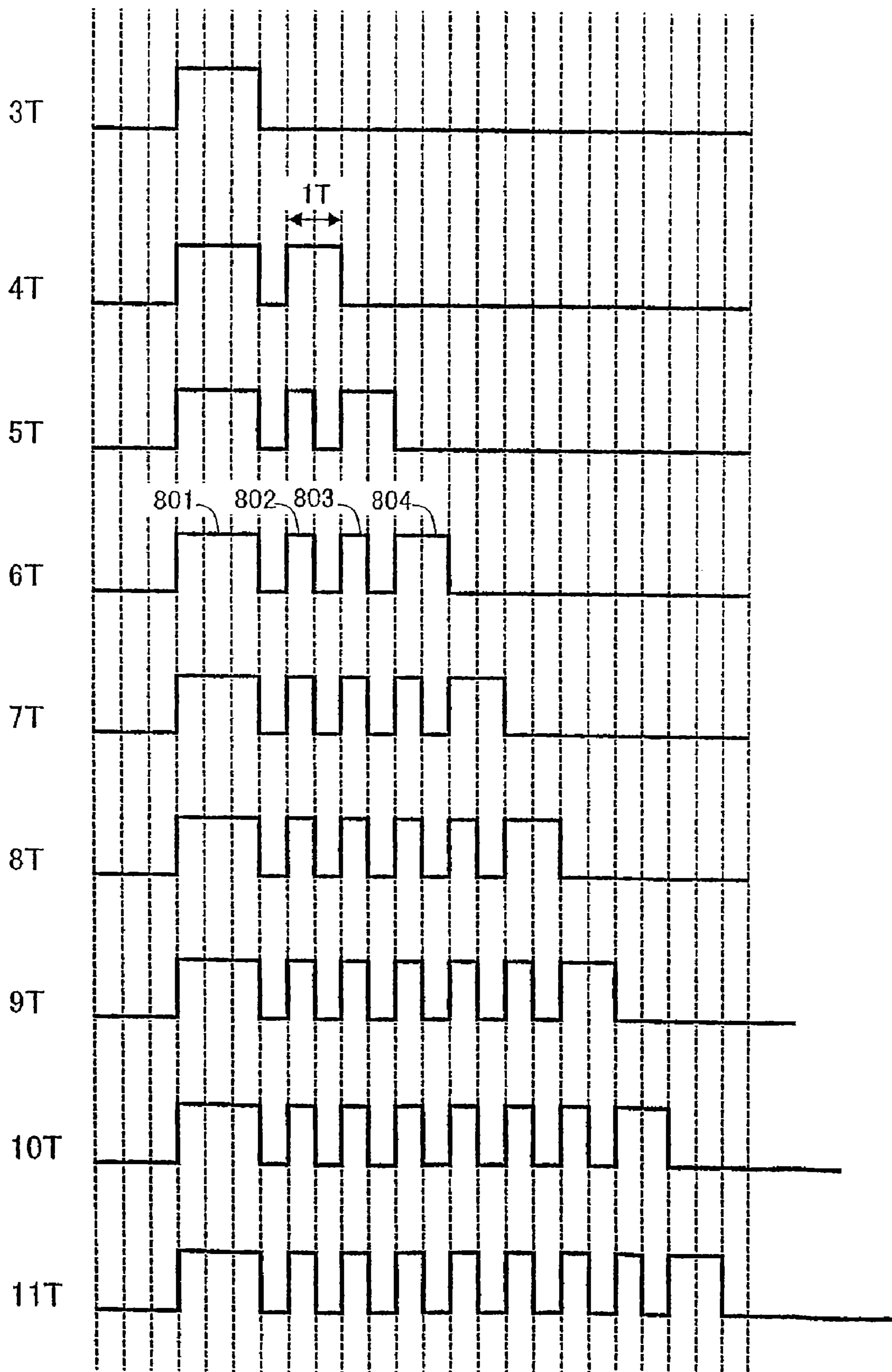
FIG. 1 (Prior Art)
