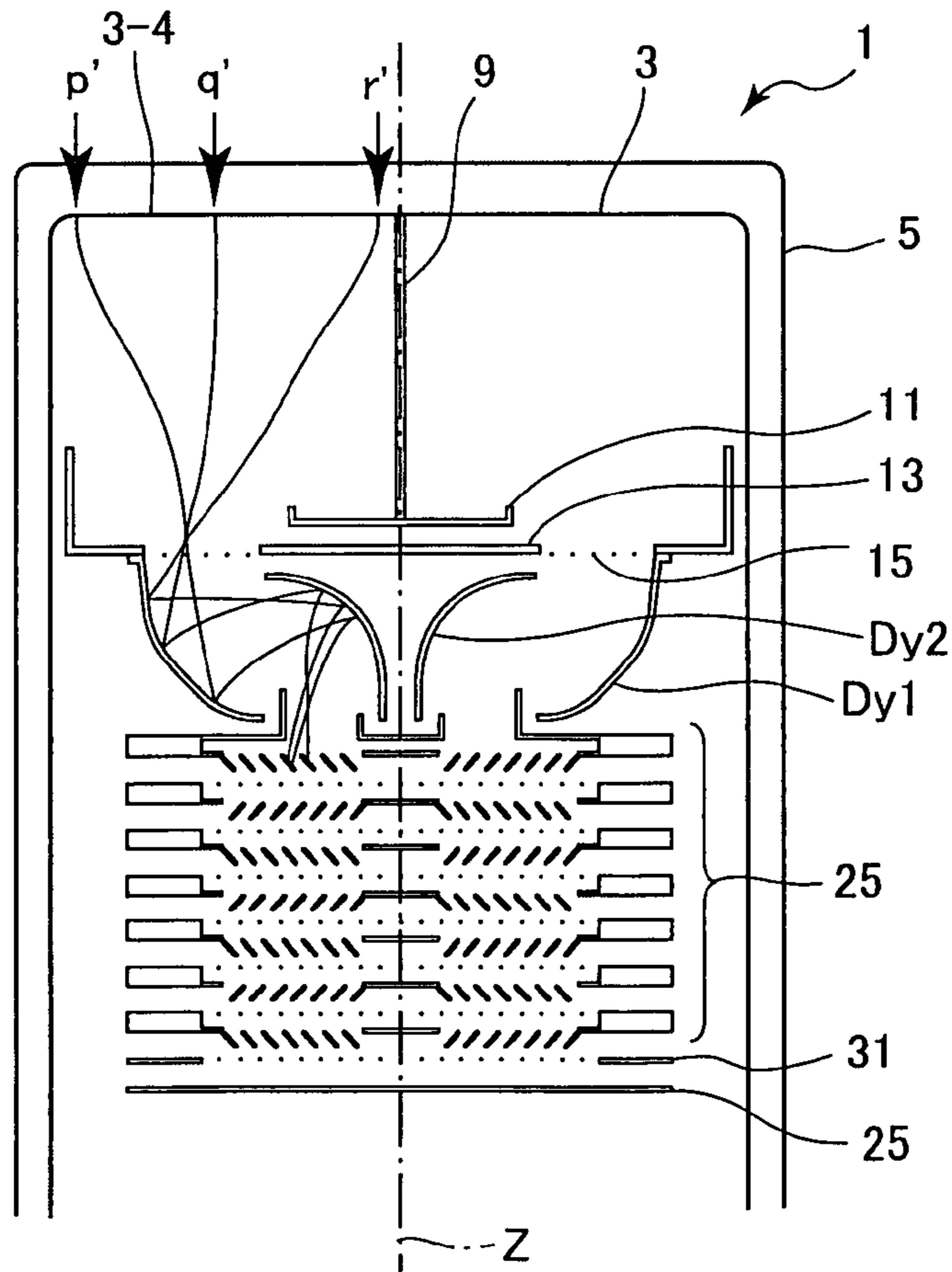
FIG.6(b)
