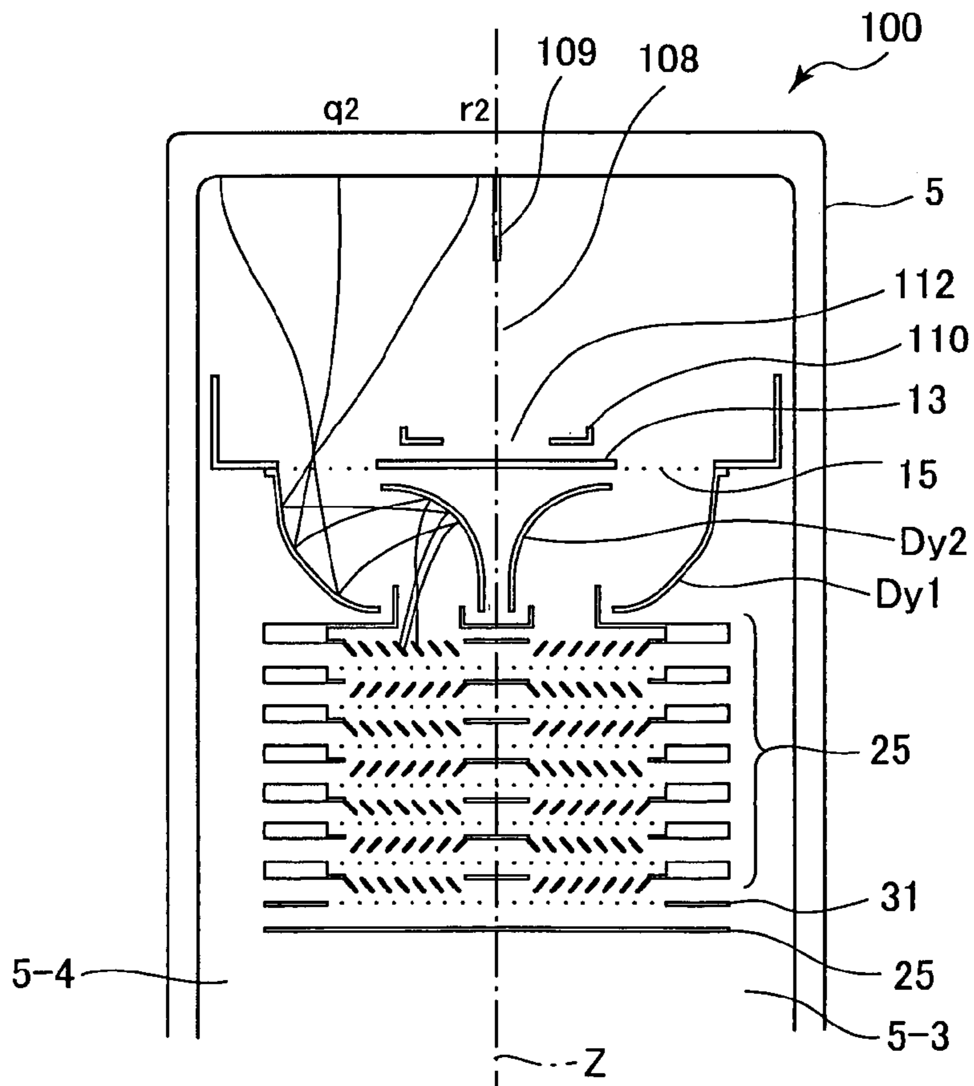
FIG.8(b)
