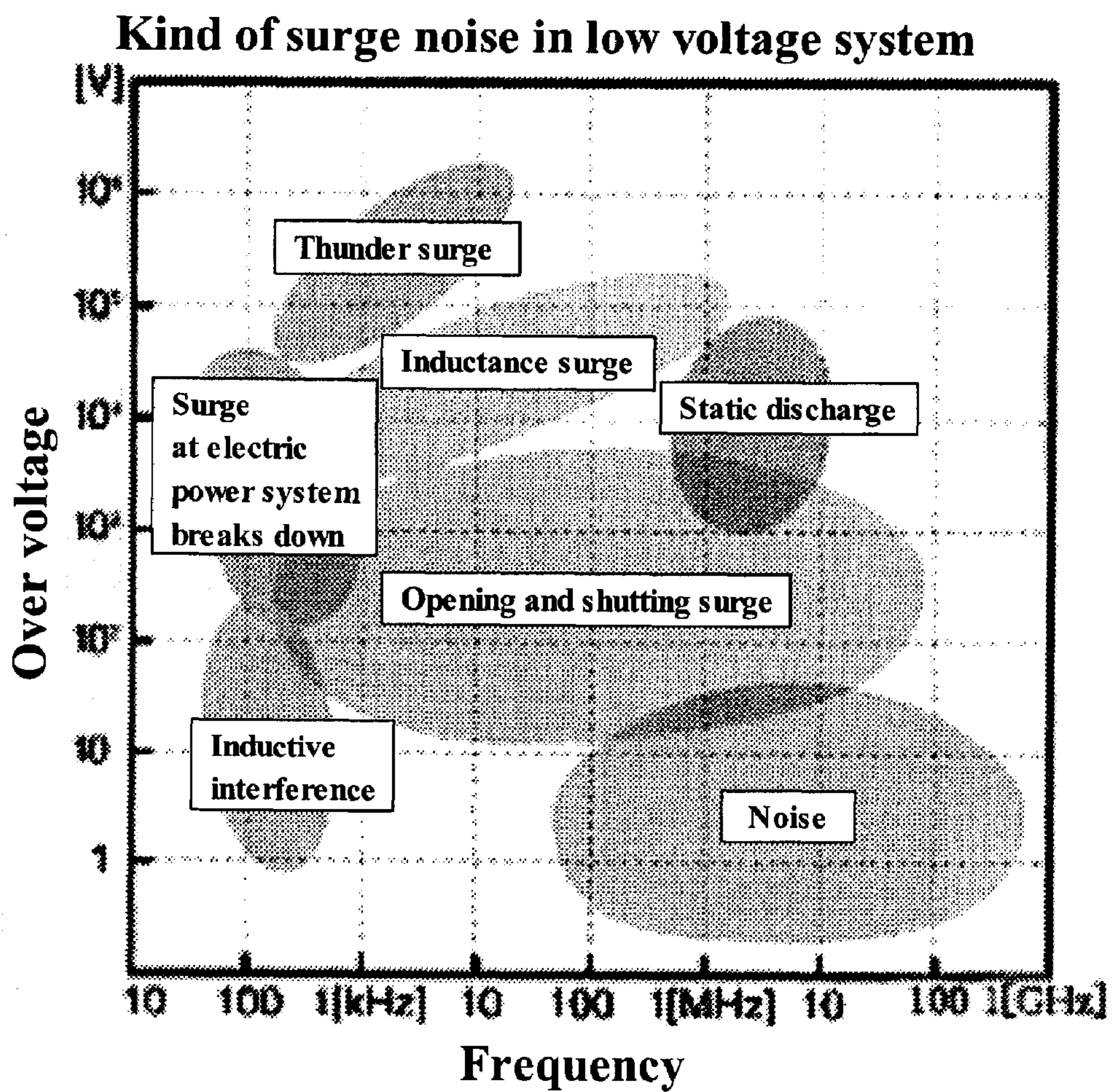
Frequency distribution of surge
