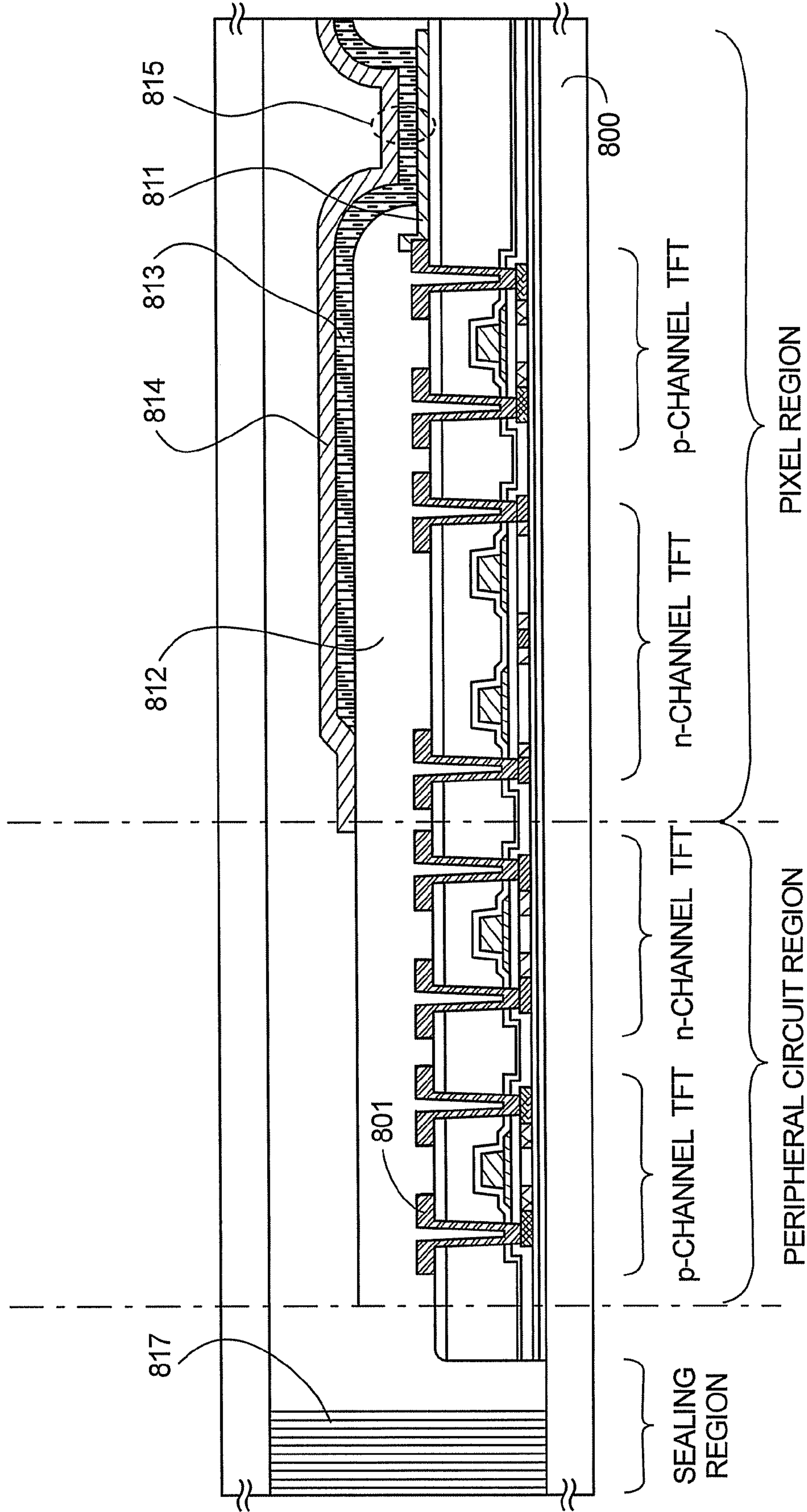
FIG. 6 PRIOR ART
