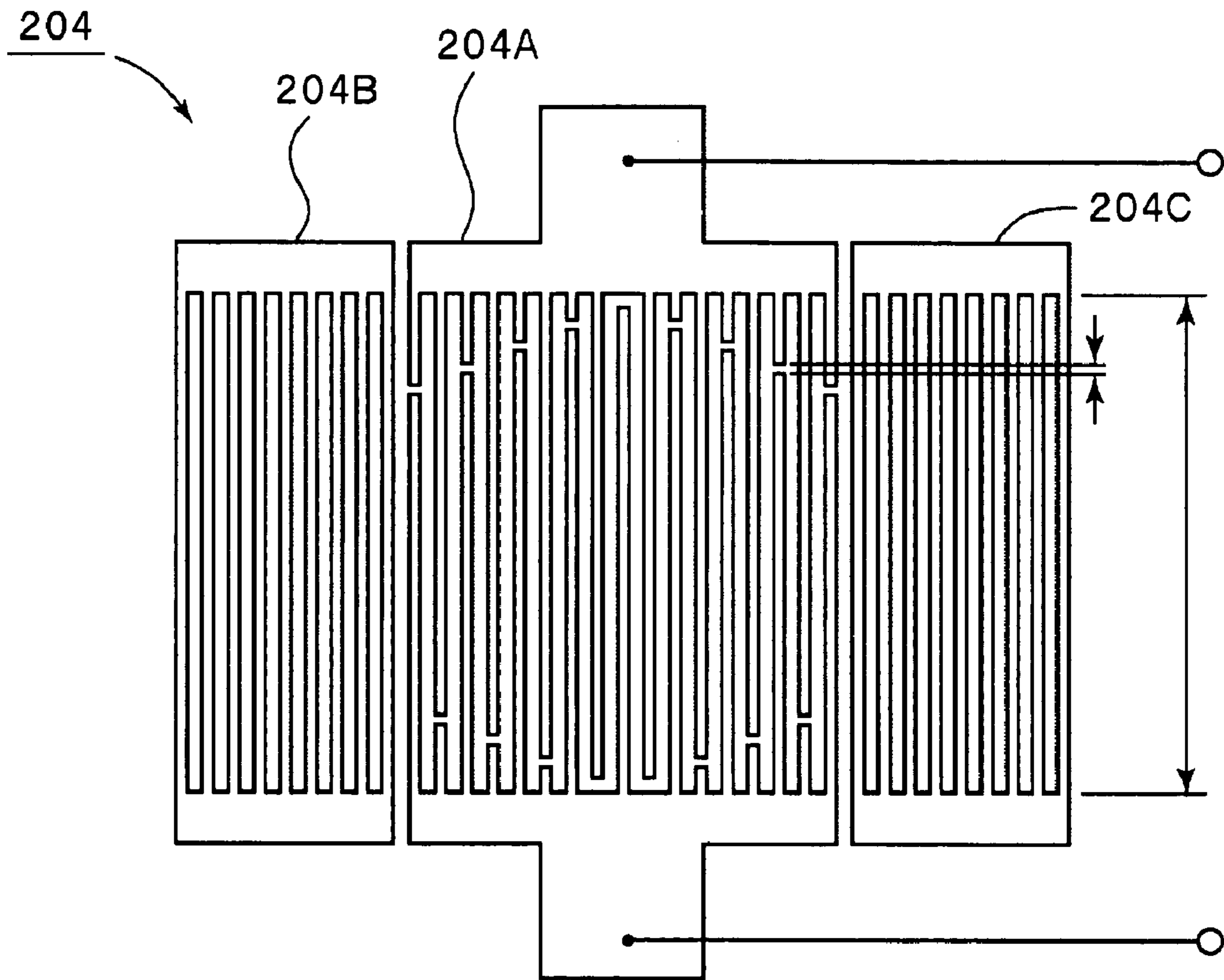
FIG. 34 PRIOR ART
